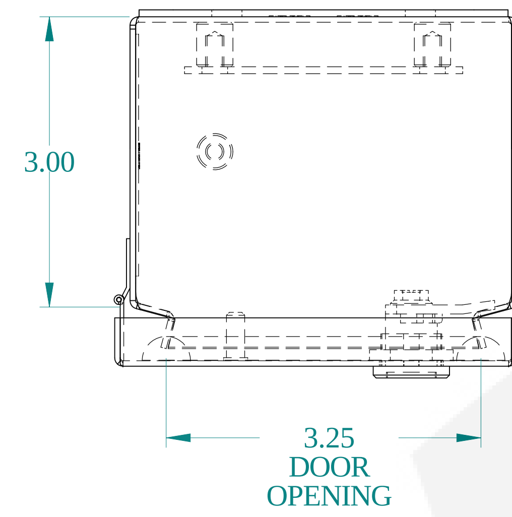
TOP VIEW
