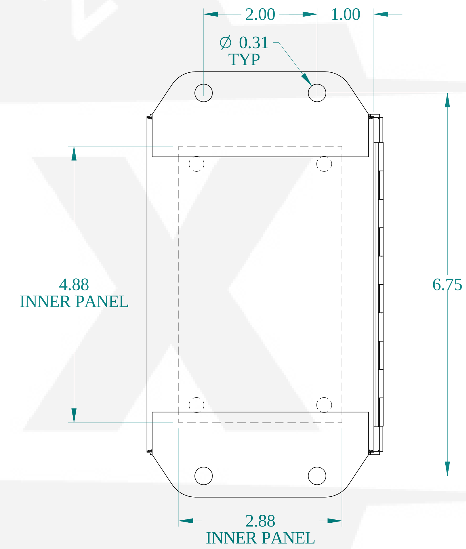
BACK VIEW
