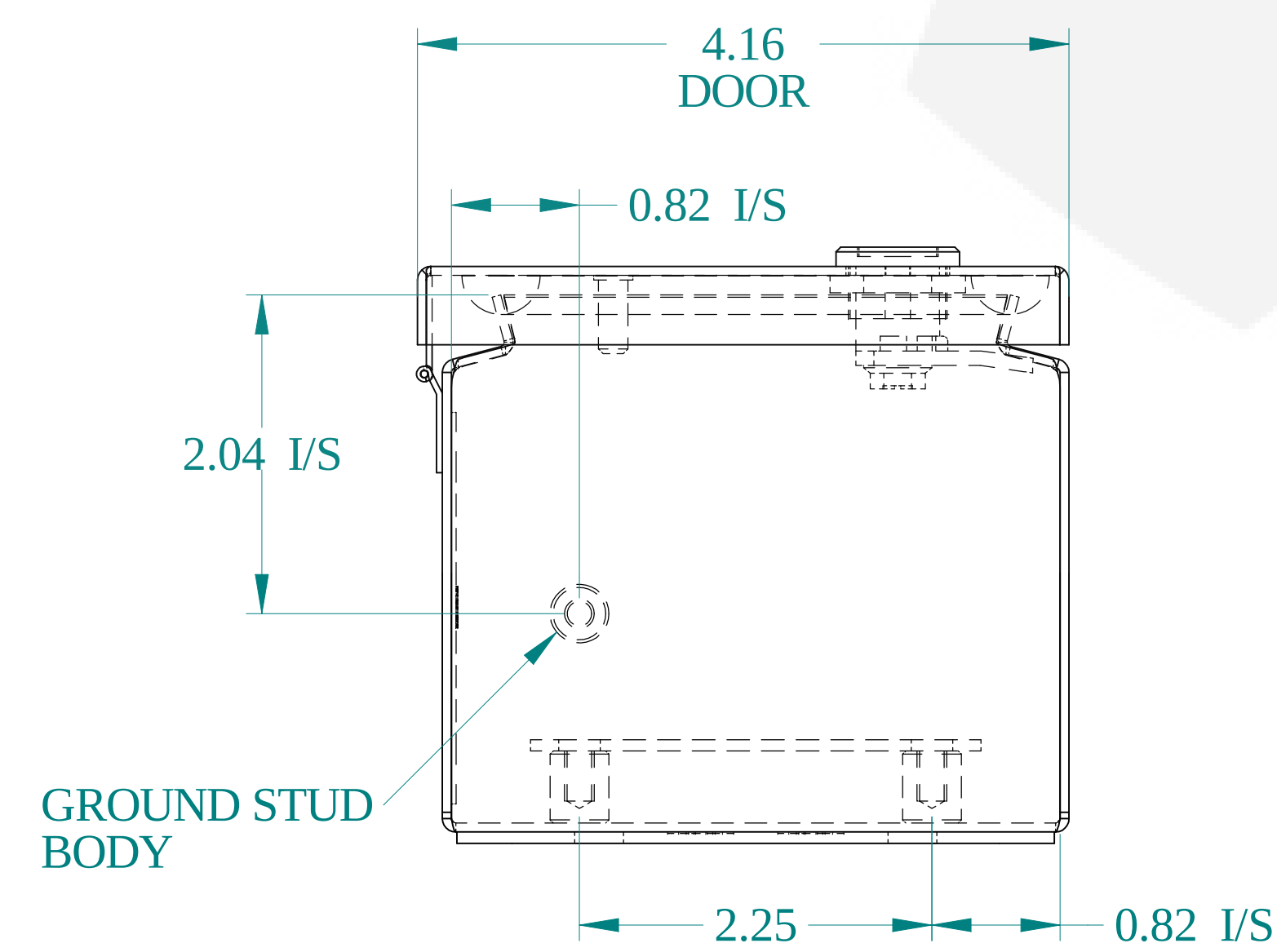
BOTTOM VIEW
