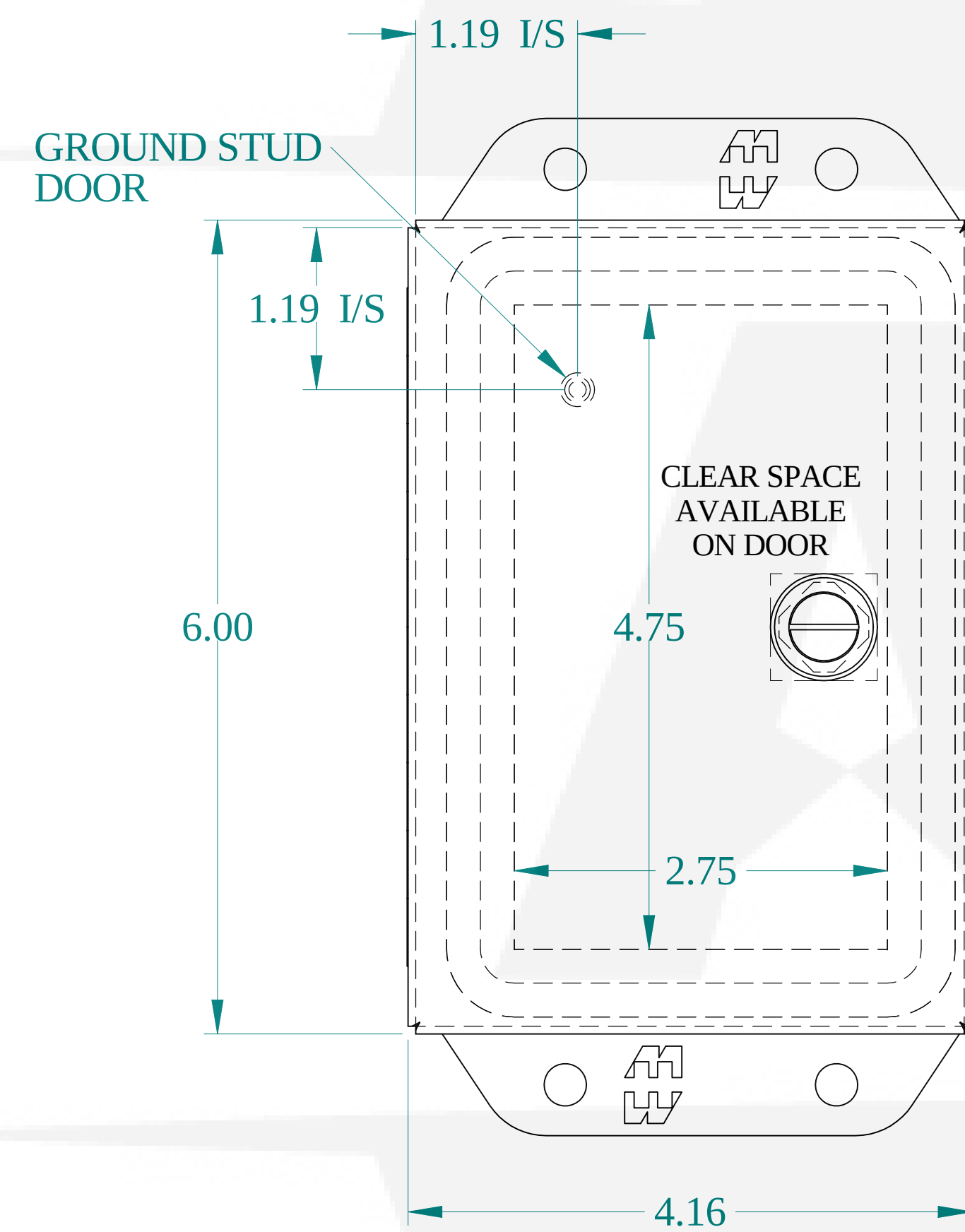
FRONT VIEW
