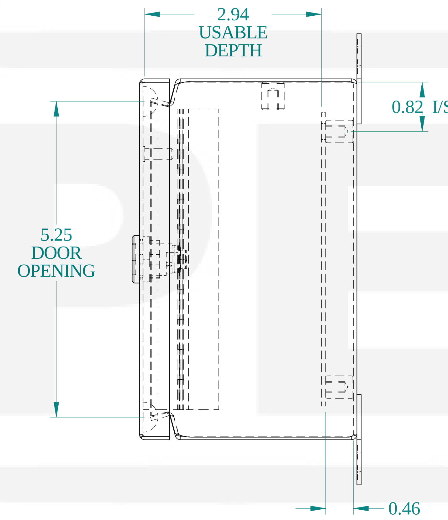
SIDE VIEW
