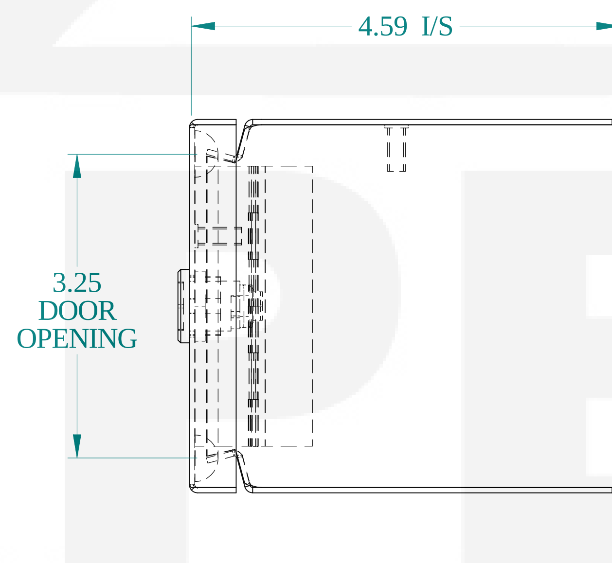
SIDE VIEW
