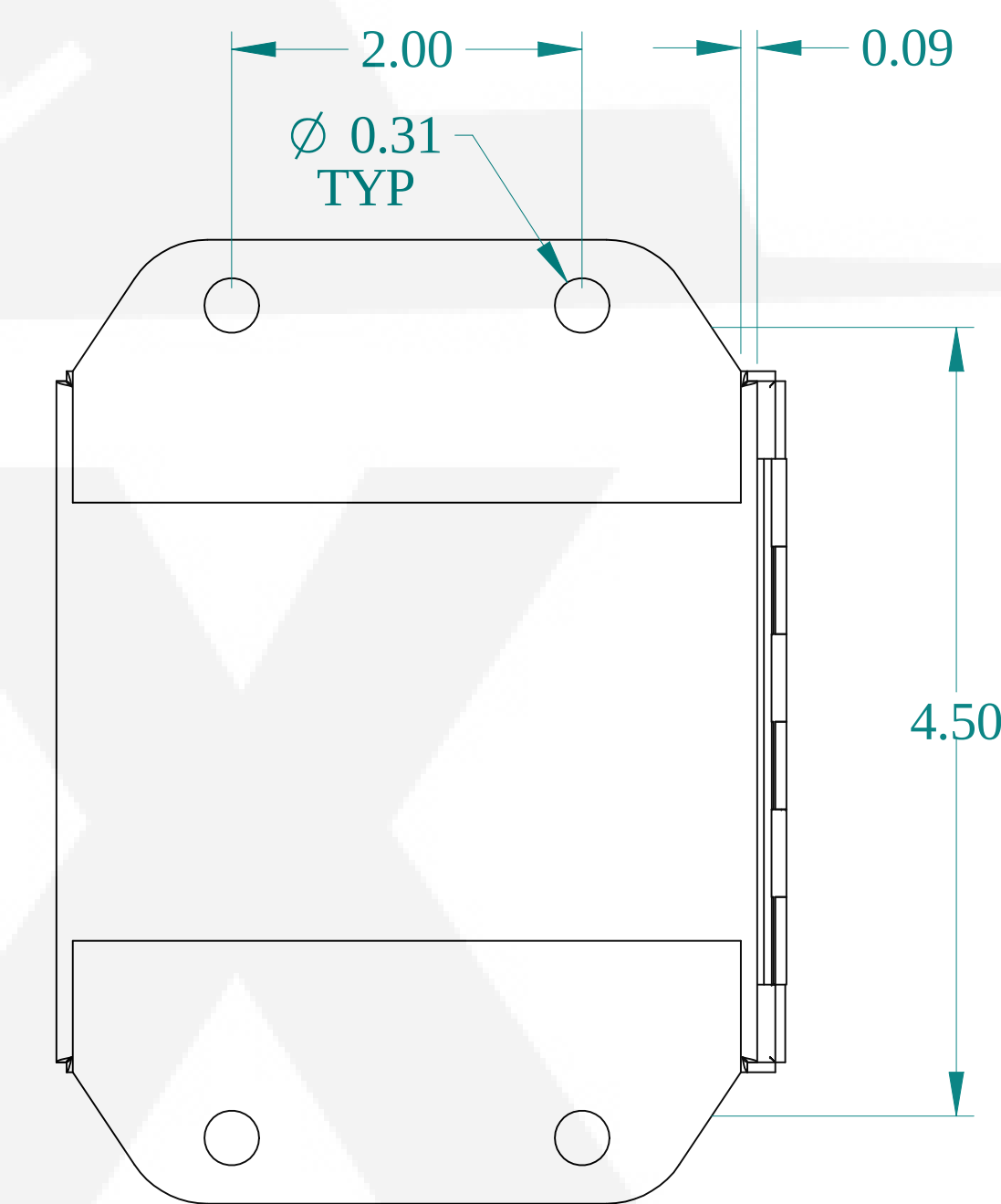
BACK VIEW
