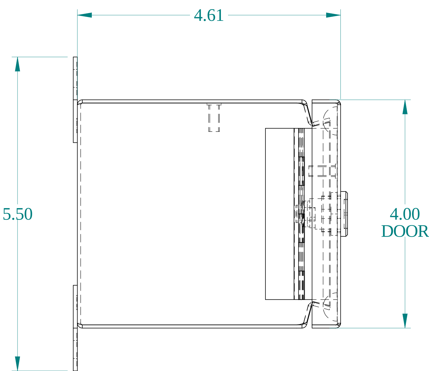
SIDE VIEW
