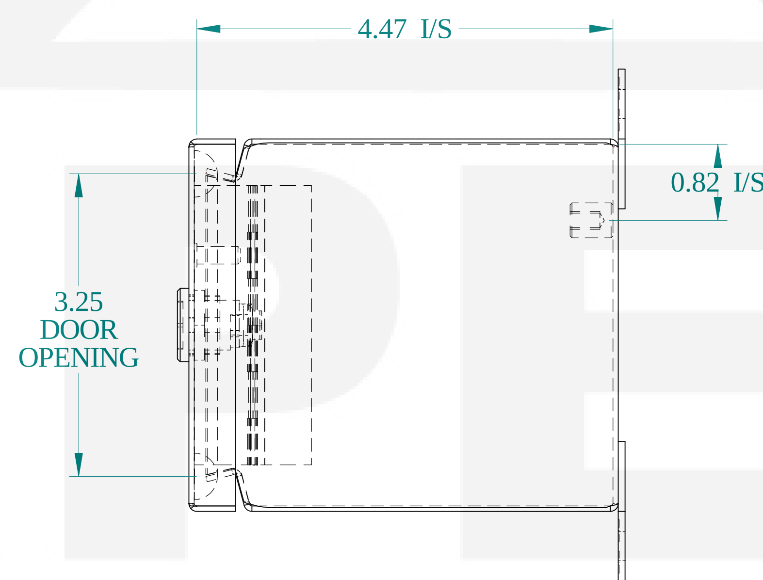
SIDE VIEW
