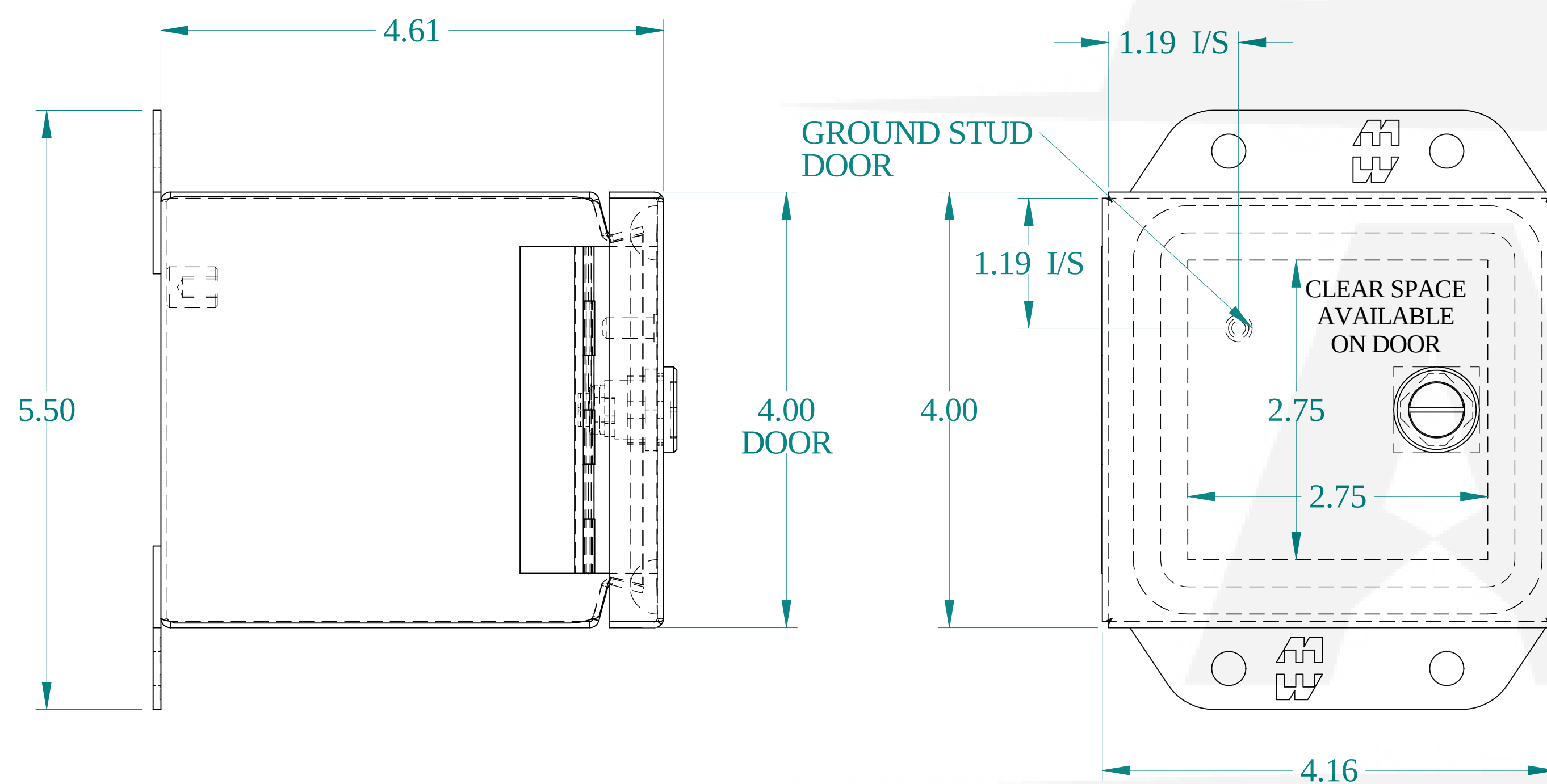
SIDE VIEW
