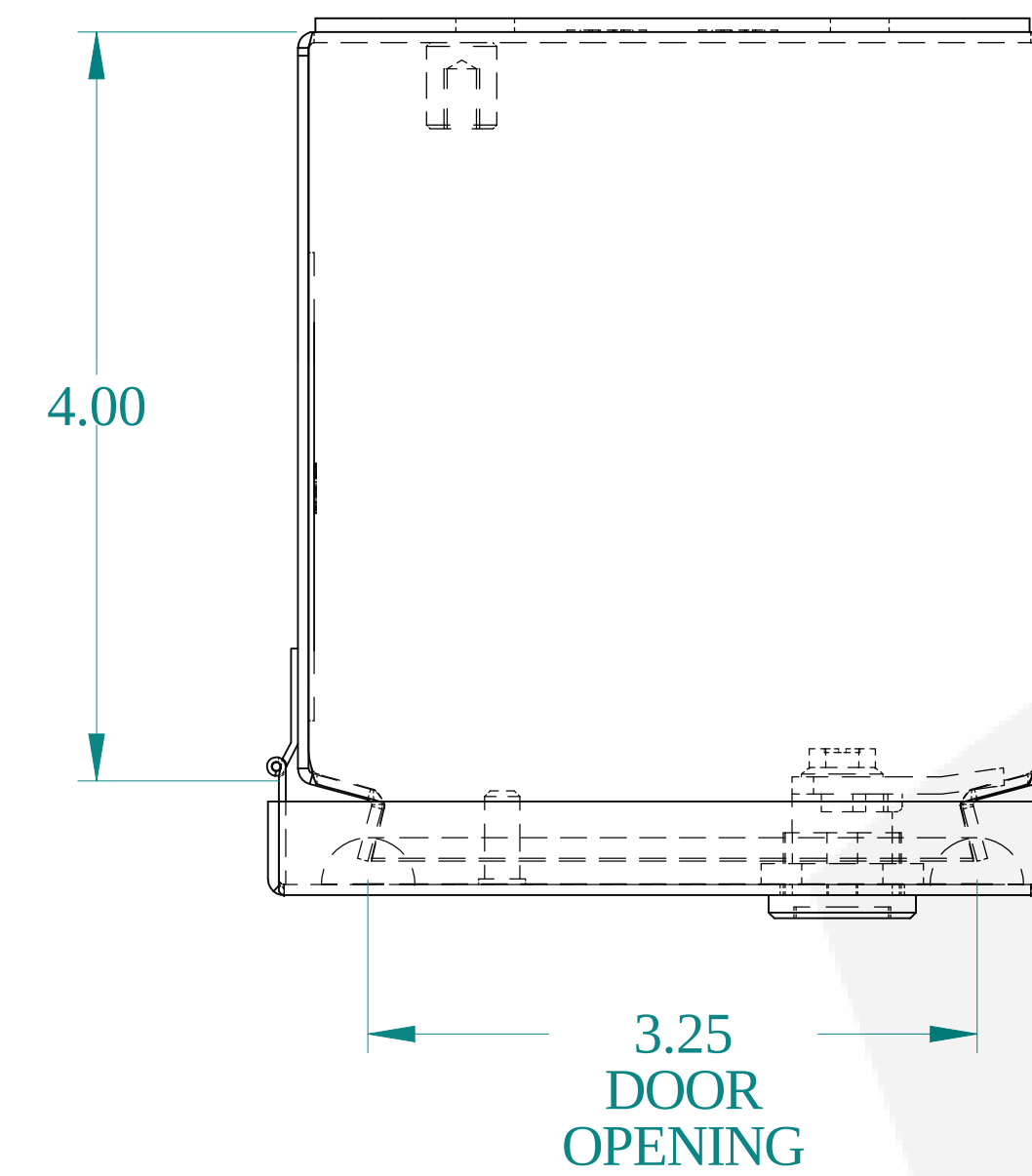
TOP VIEW
