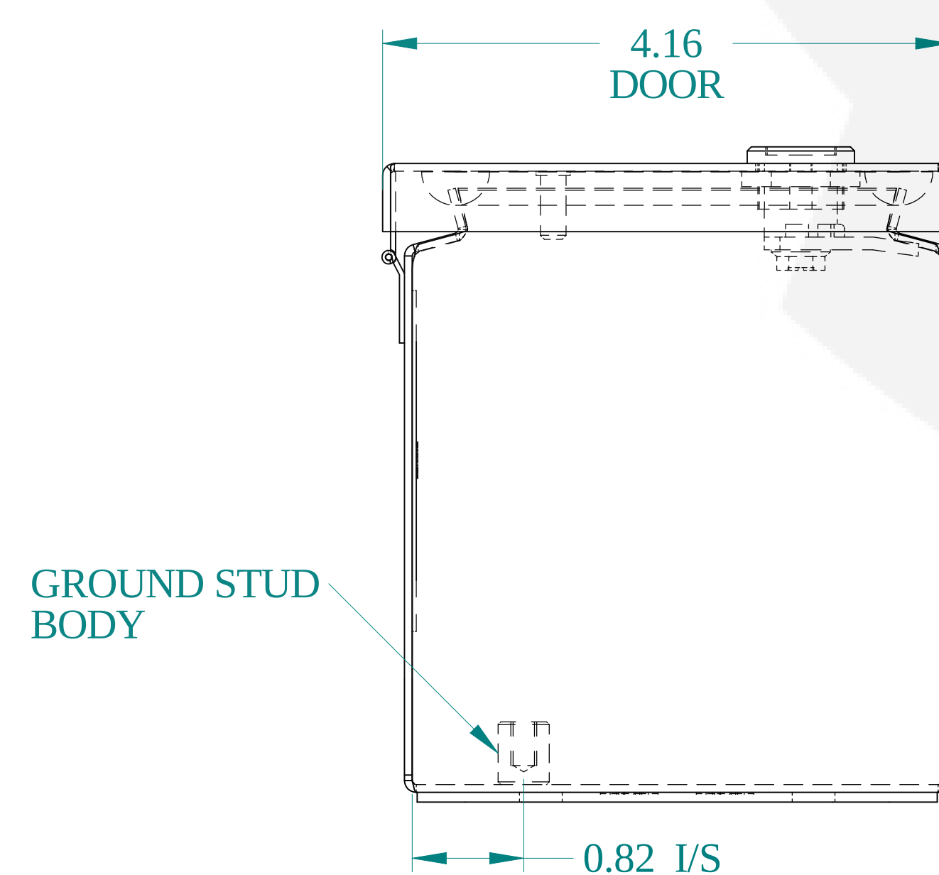
BOTTOM VIEW
