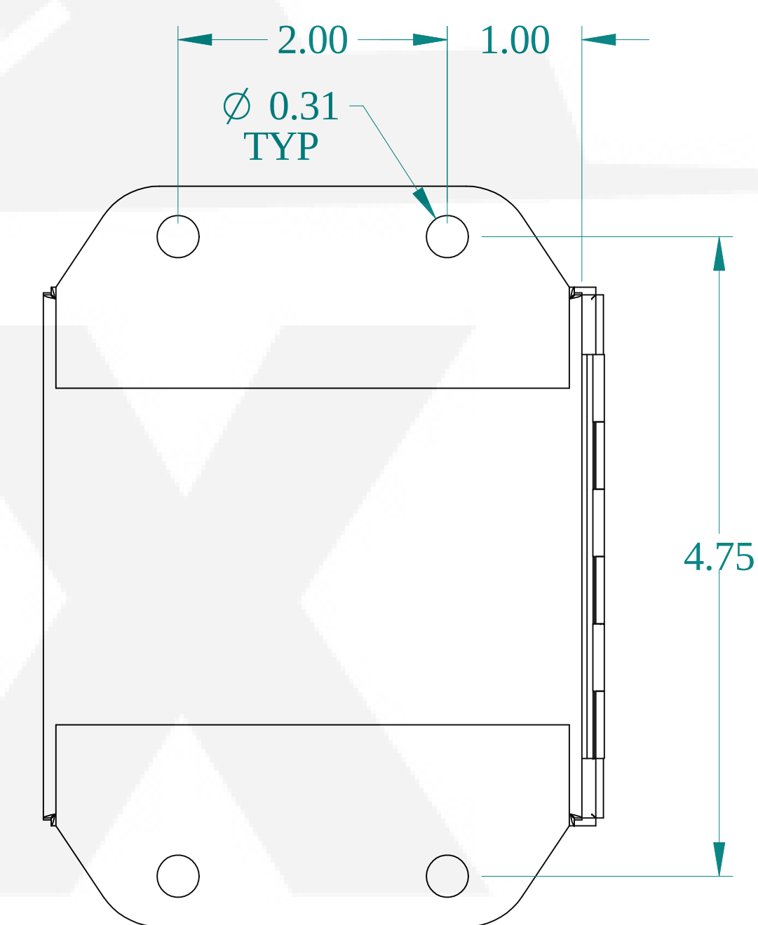
BACK VIEW
