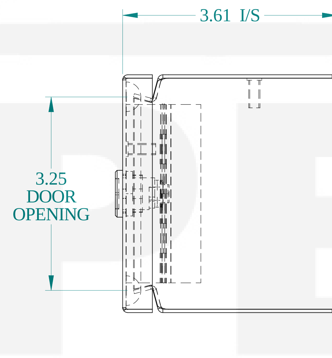
SIDE VIEW
