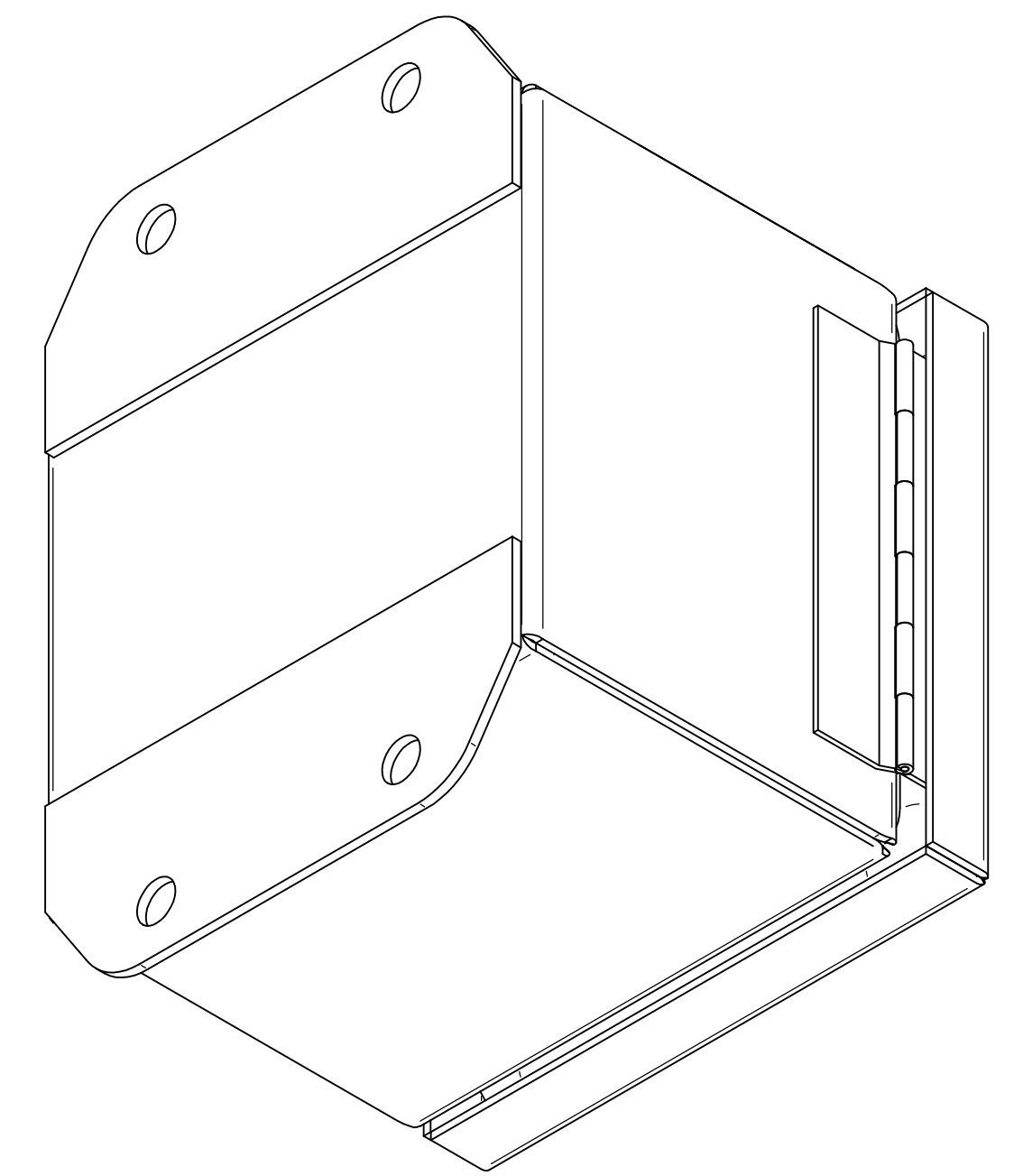
ISOMETRIC VIEWS
