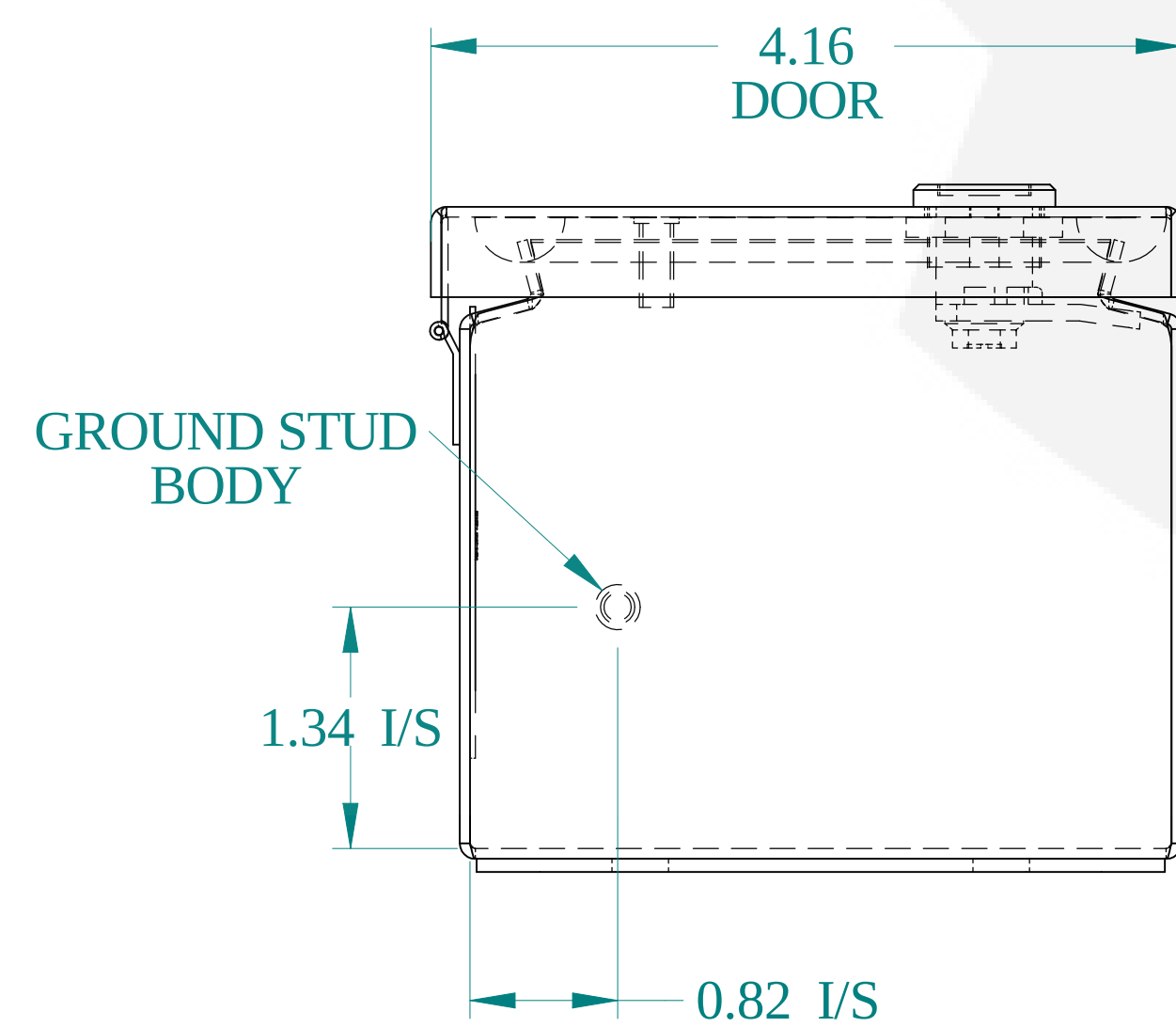
BOTTOM VIEW
