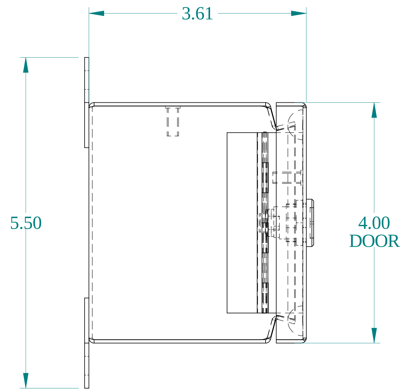
SIDE VIEW
