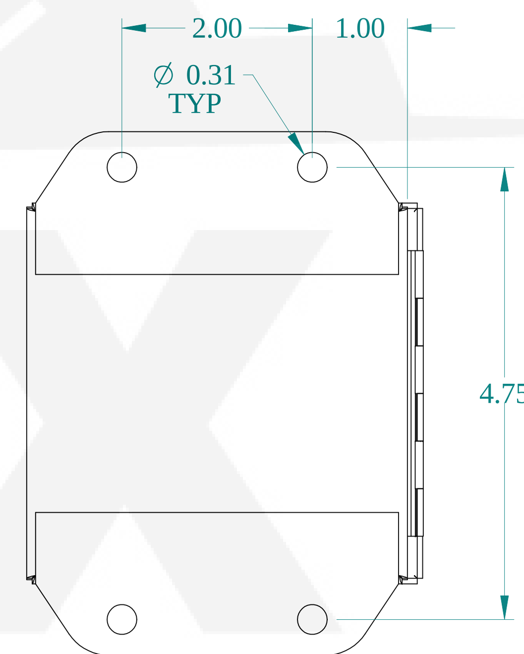
BACK VIEW
