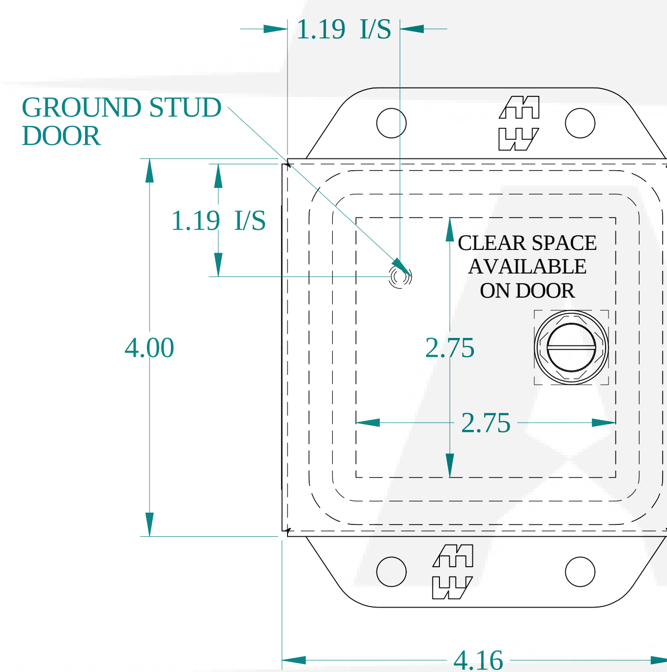
FRONT VIEW
