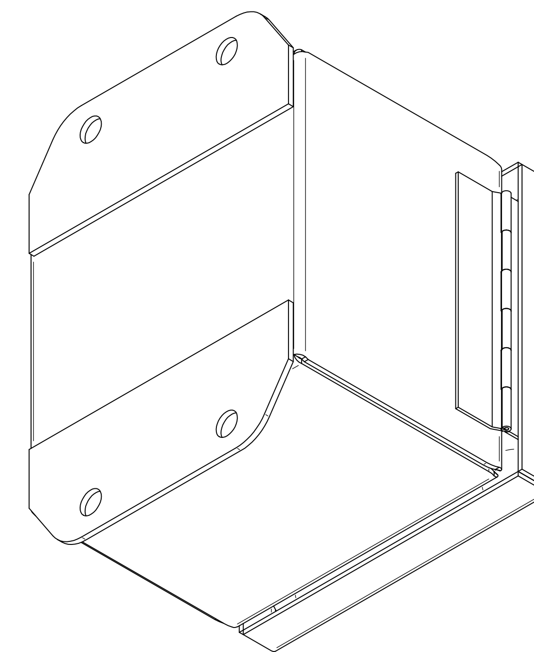
ISOMETRIC VIEWS
