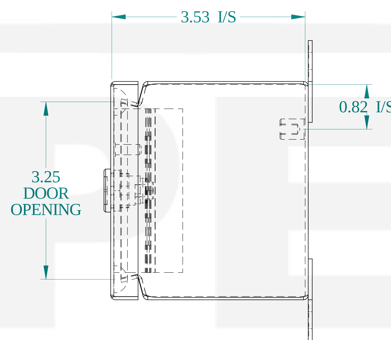
SIDE VIEW
