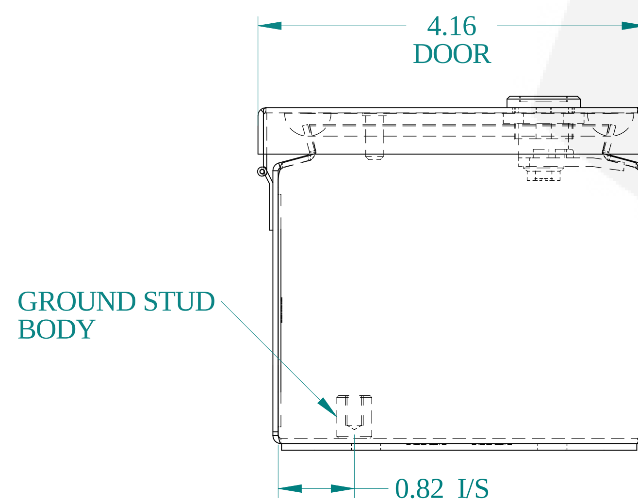
BOTTOM VIEW
