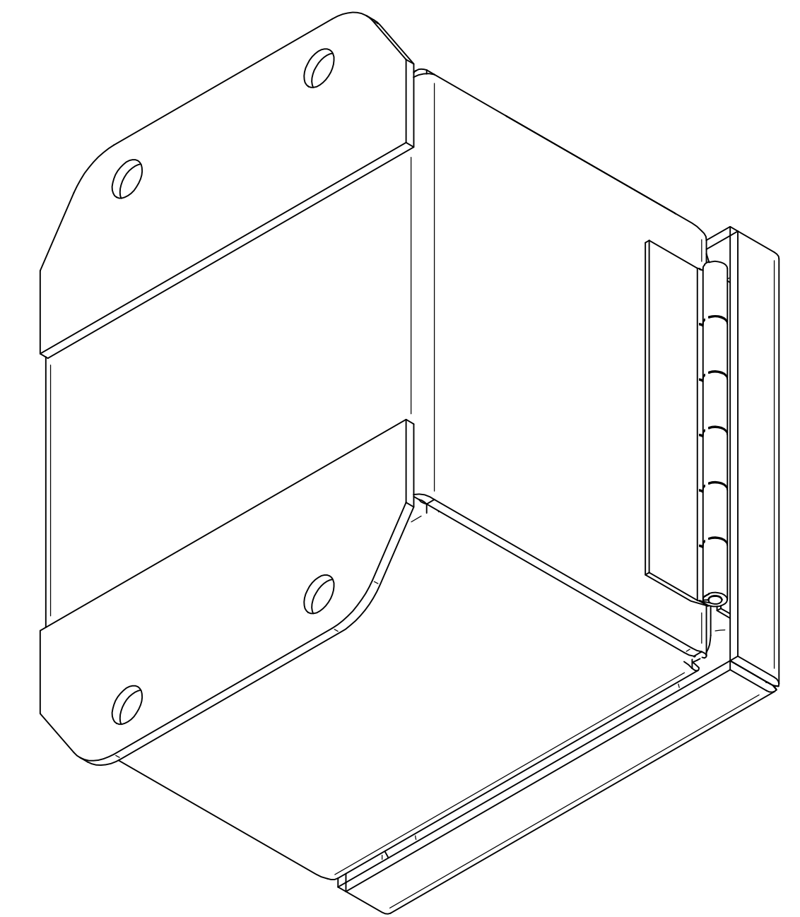
ISOMETRIC VIEWS
