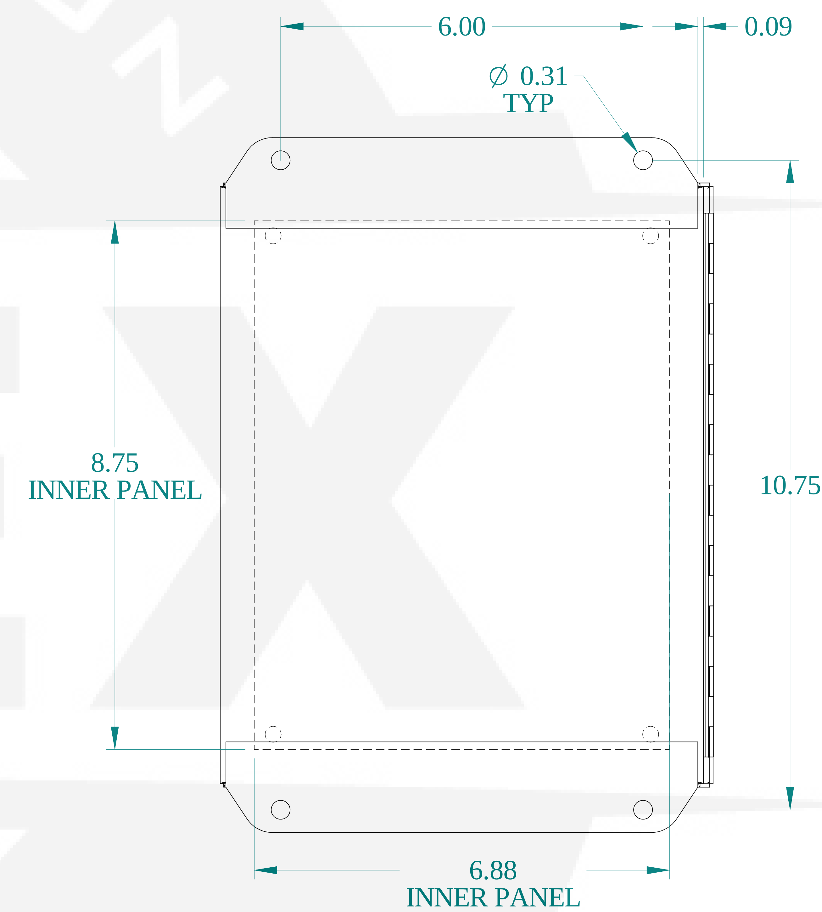
BACK VIEW
