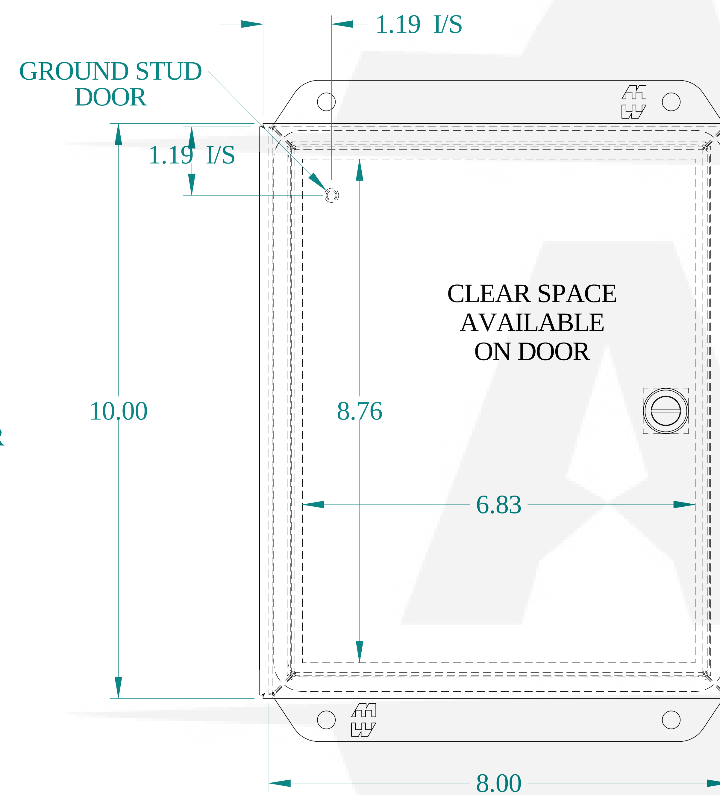
FRONT VIEW
