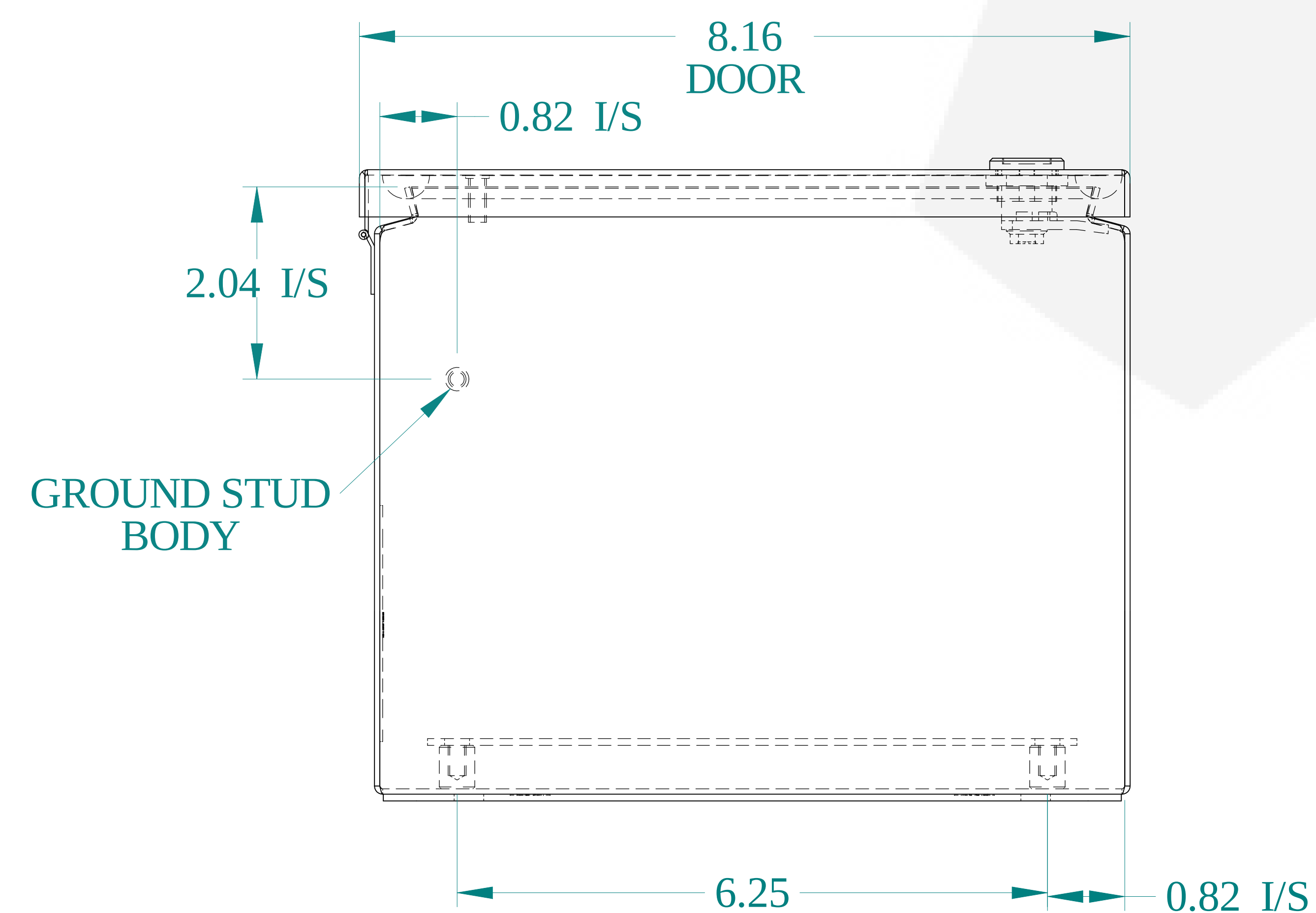
BOTTOM VIEW
