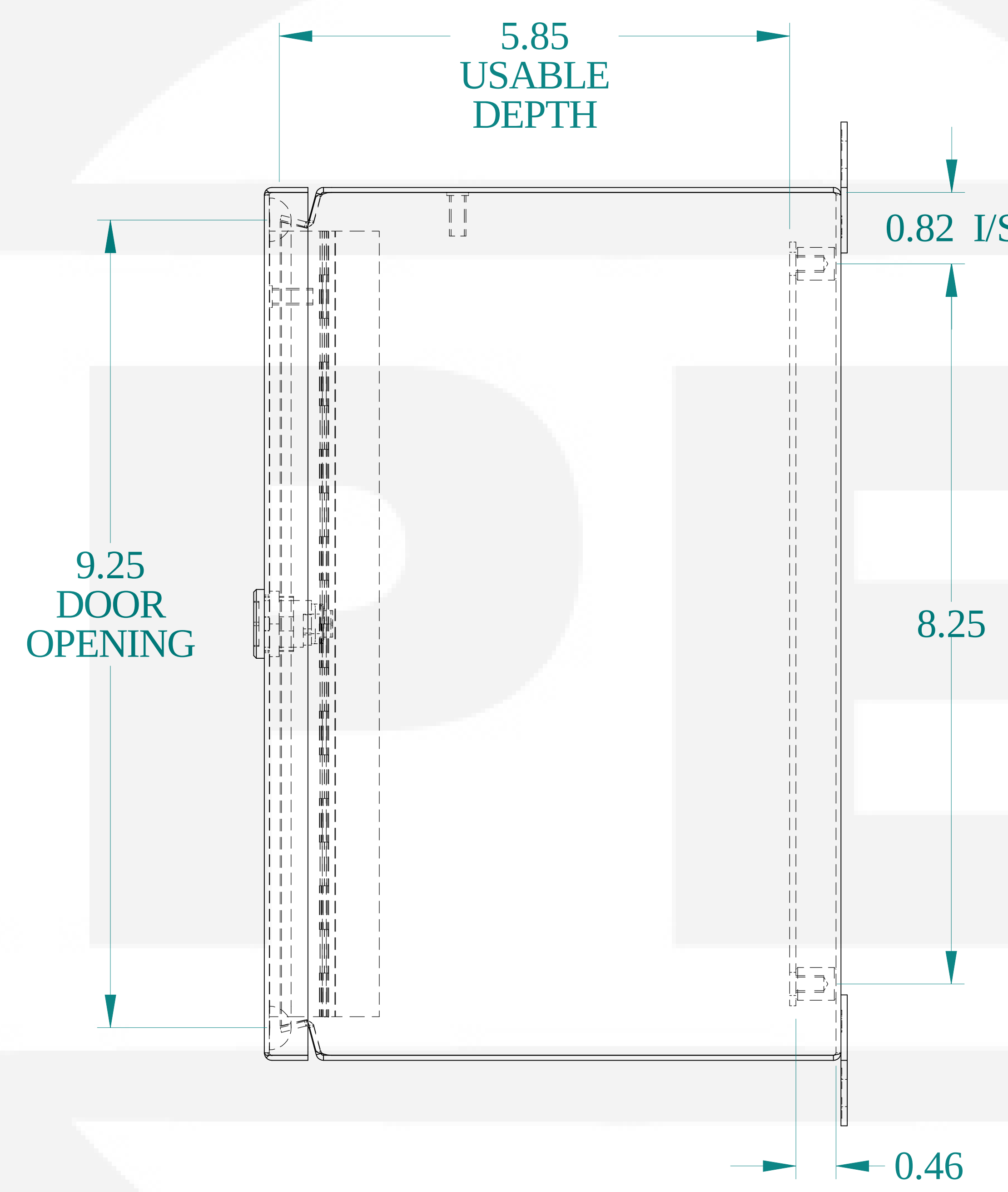
SIDE VIEW
