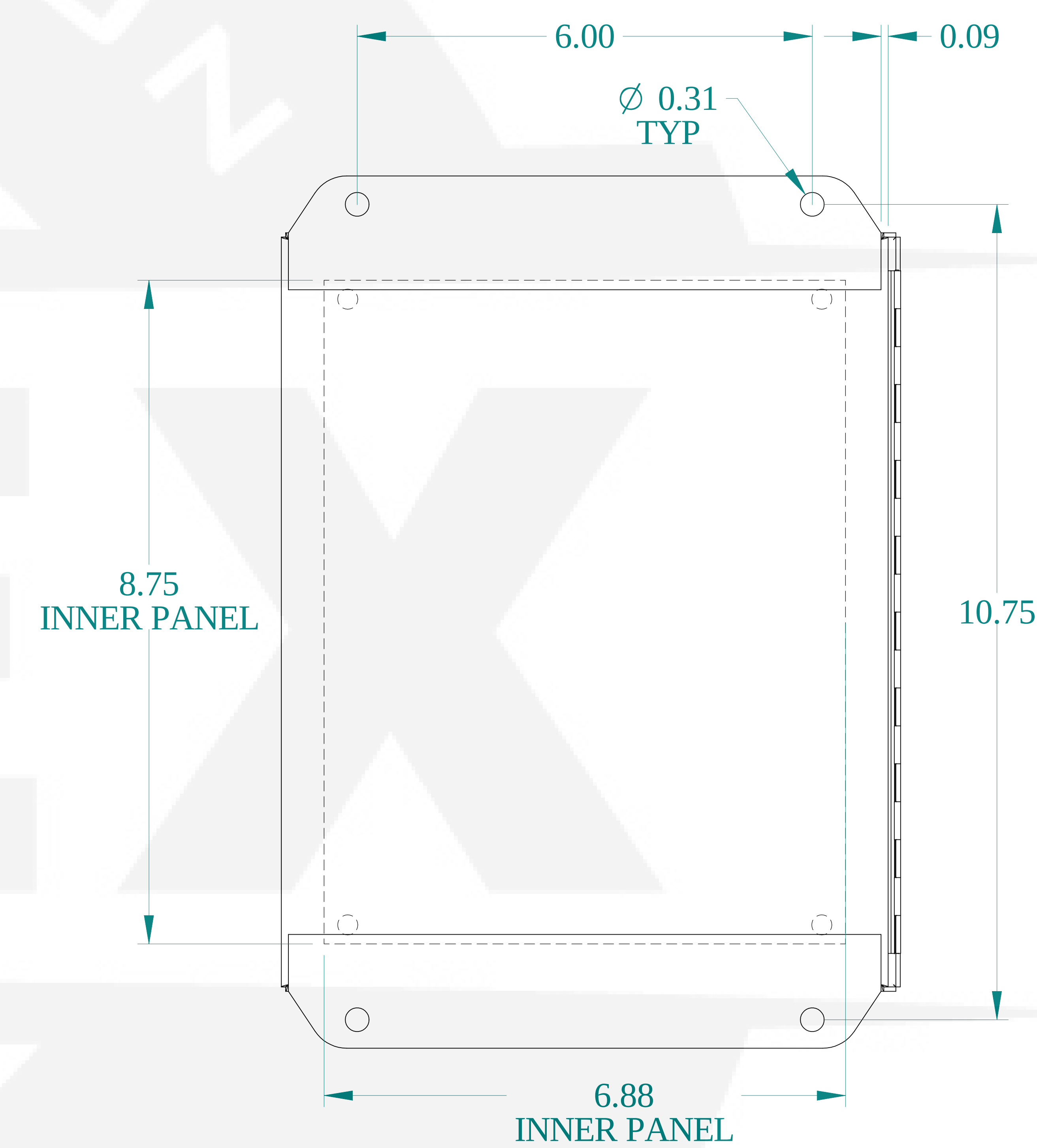
BACK VIEW
