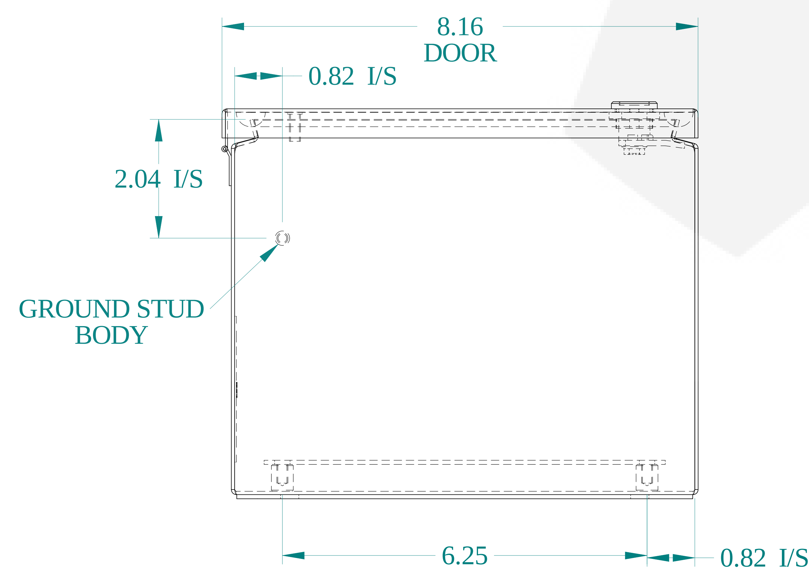
BOTTOM VIEW
