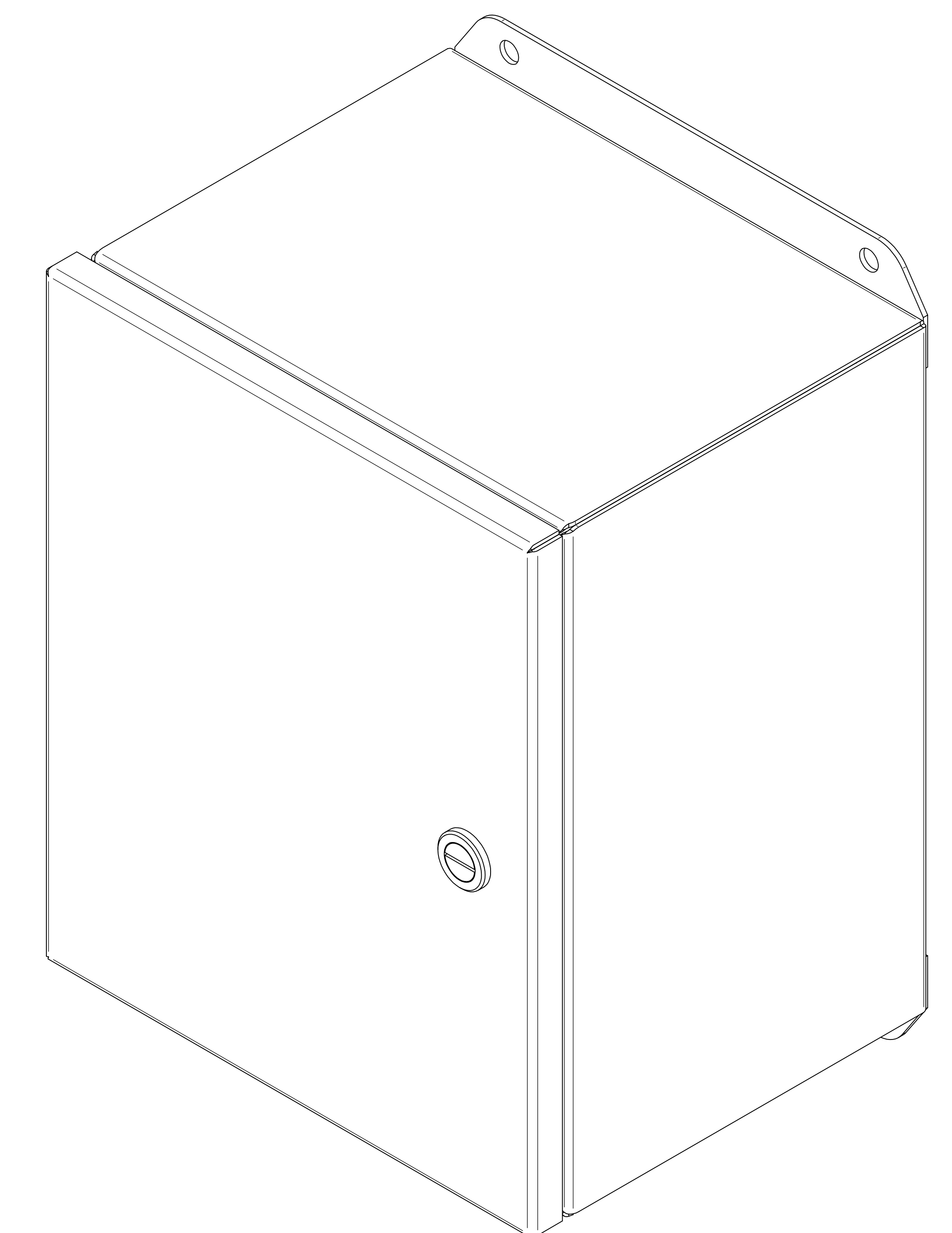
ISOMETRIC VIEWS
