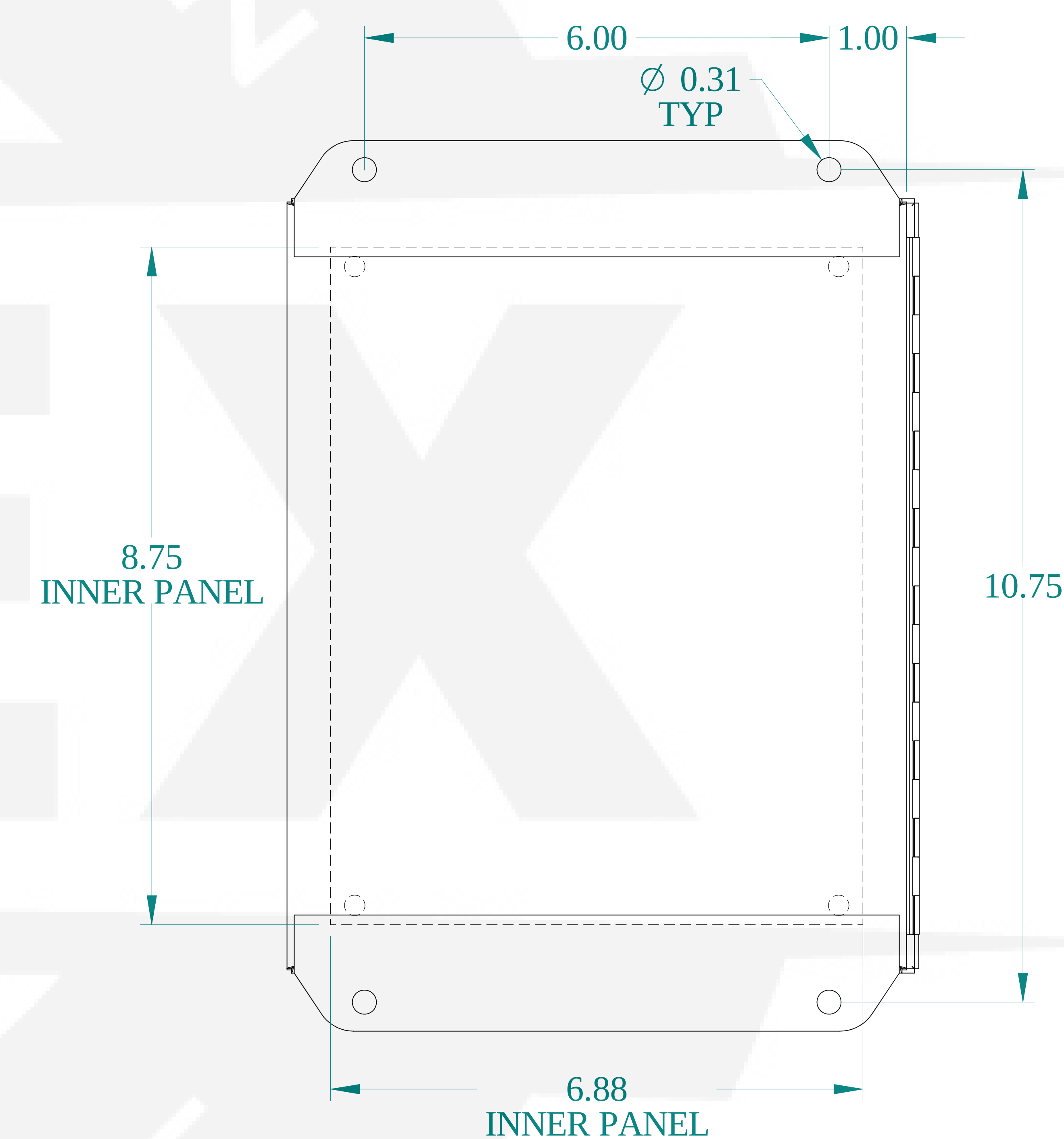
BACK VIEW
