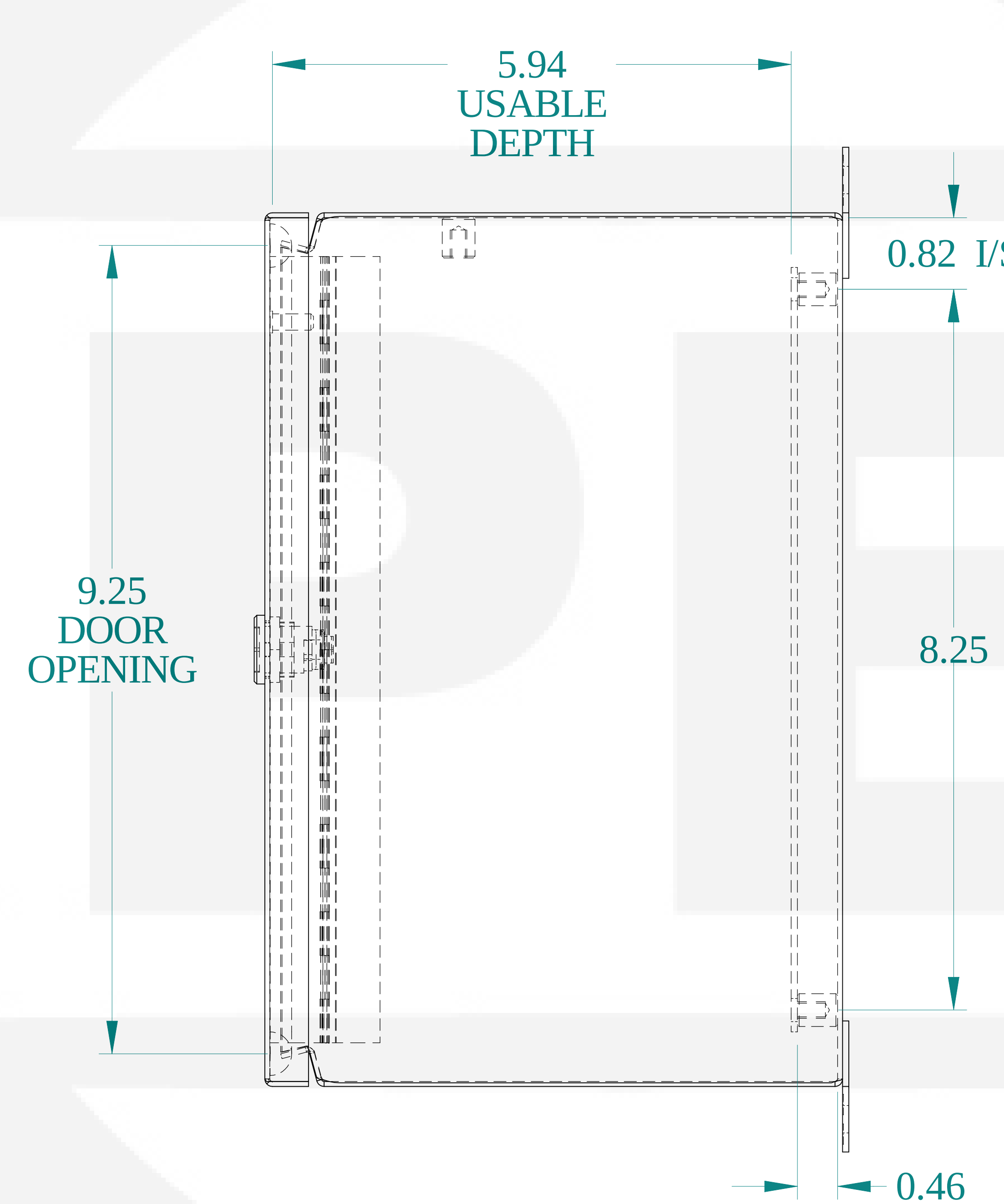
SIDE VIEW
