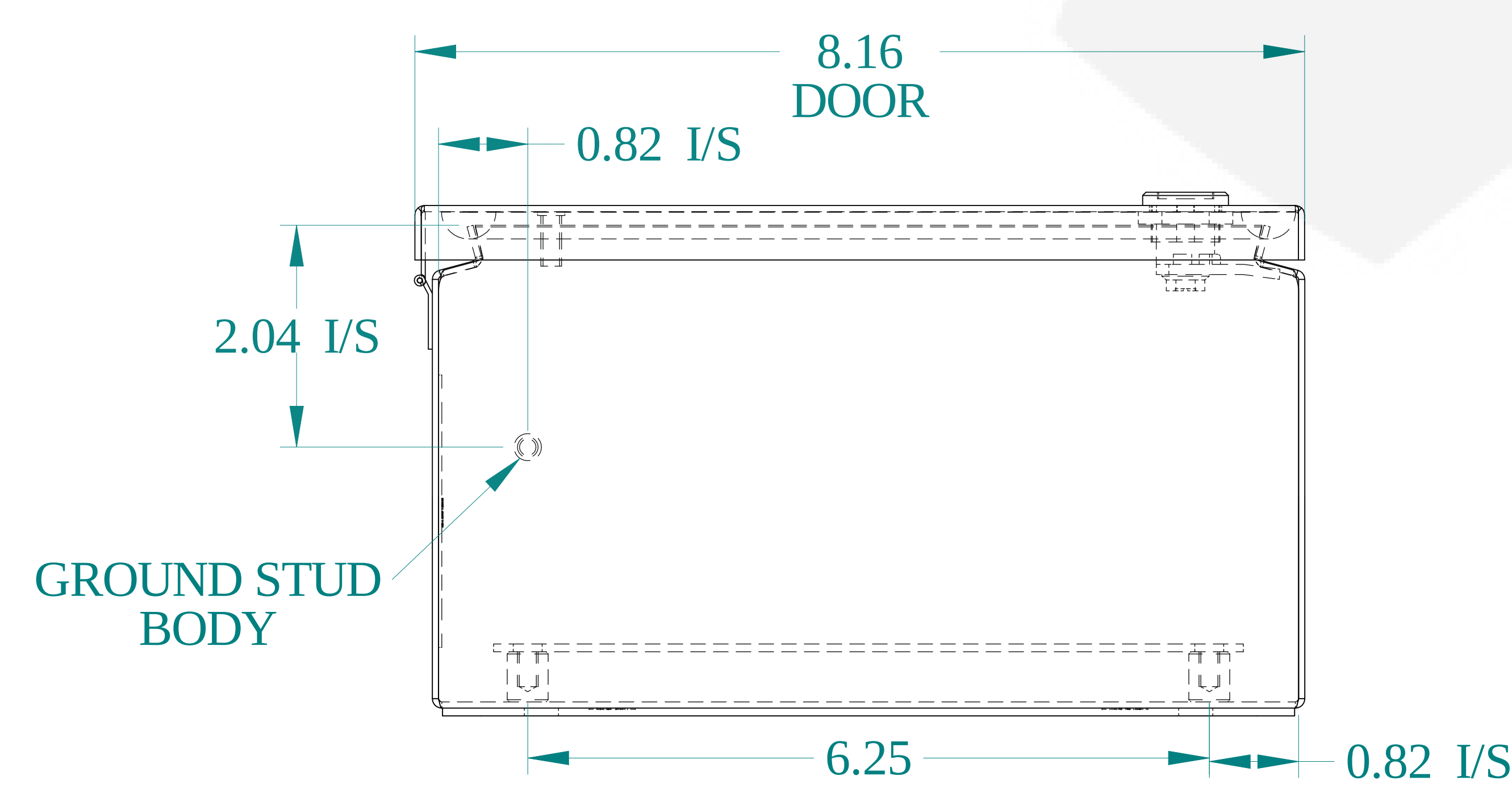
BOTTOM VIEW
