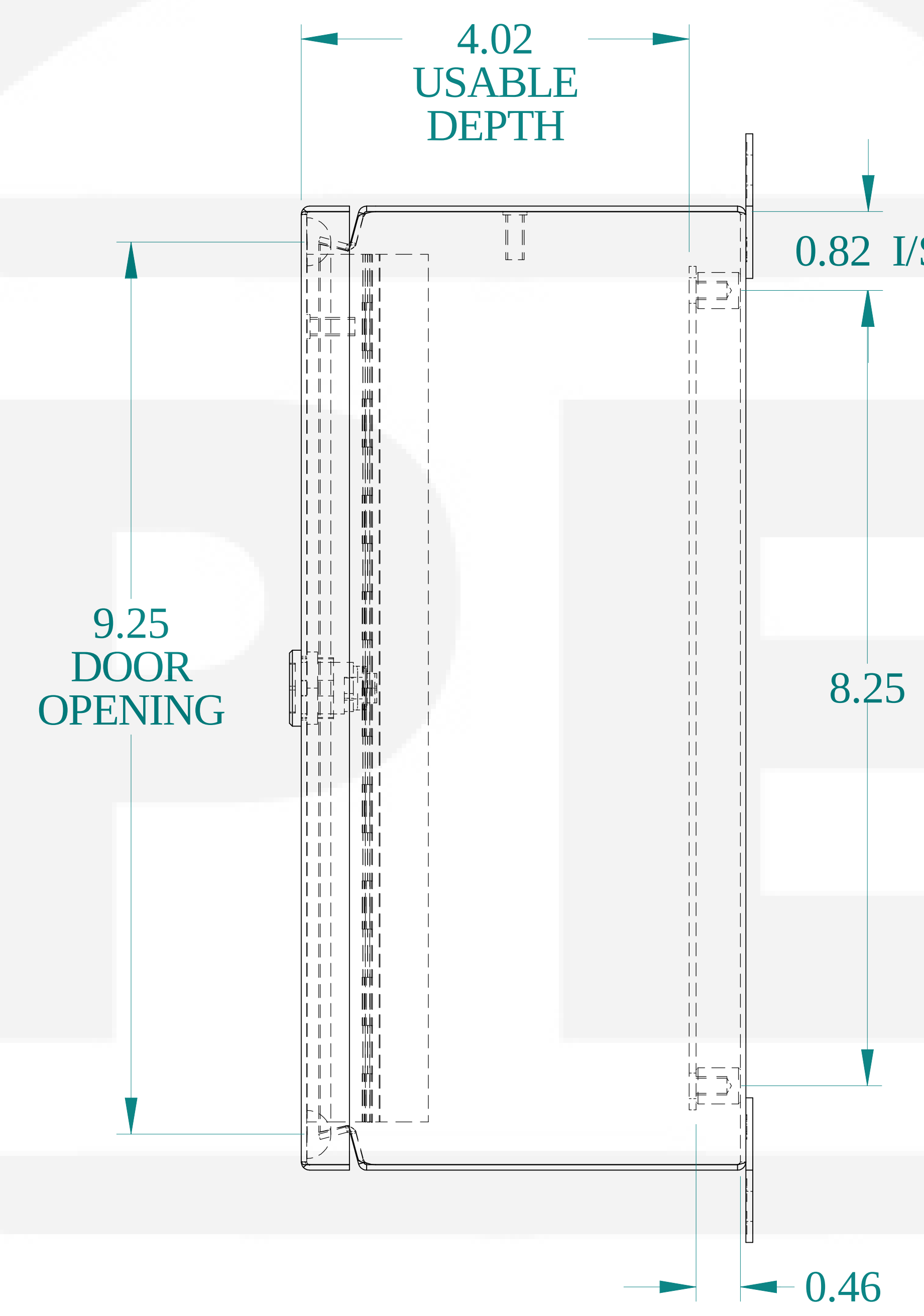
SIDE VIEW
