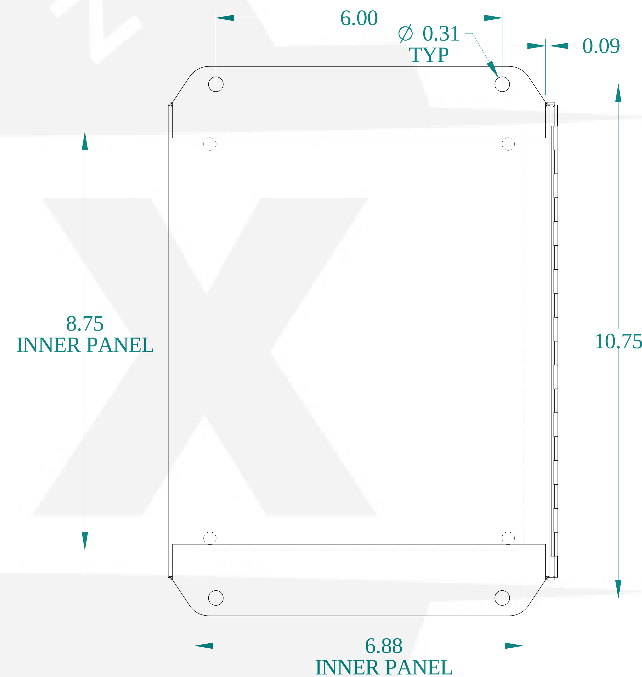
BACK VIEW
