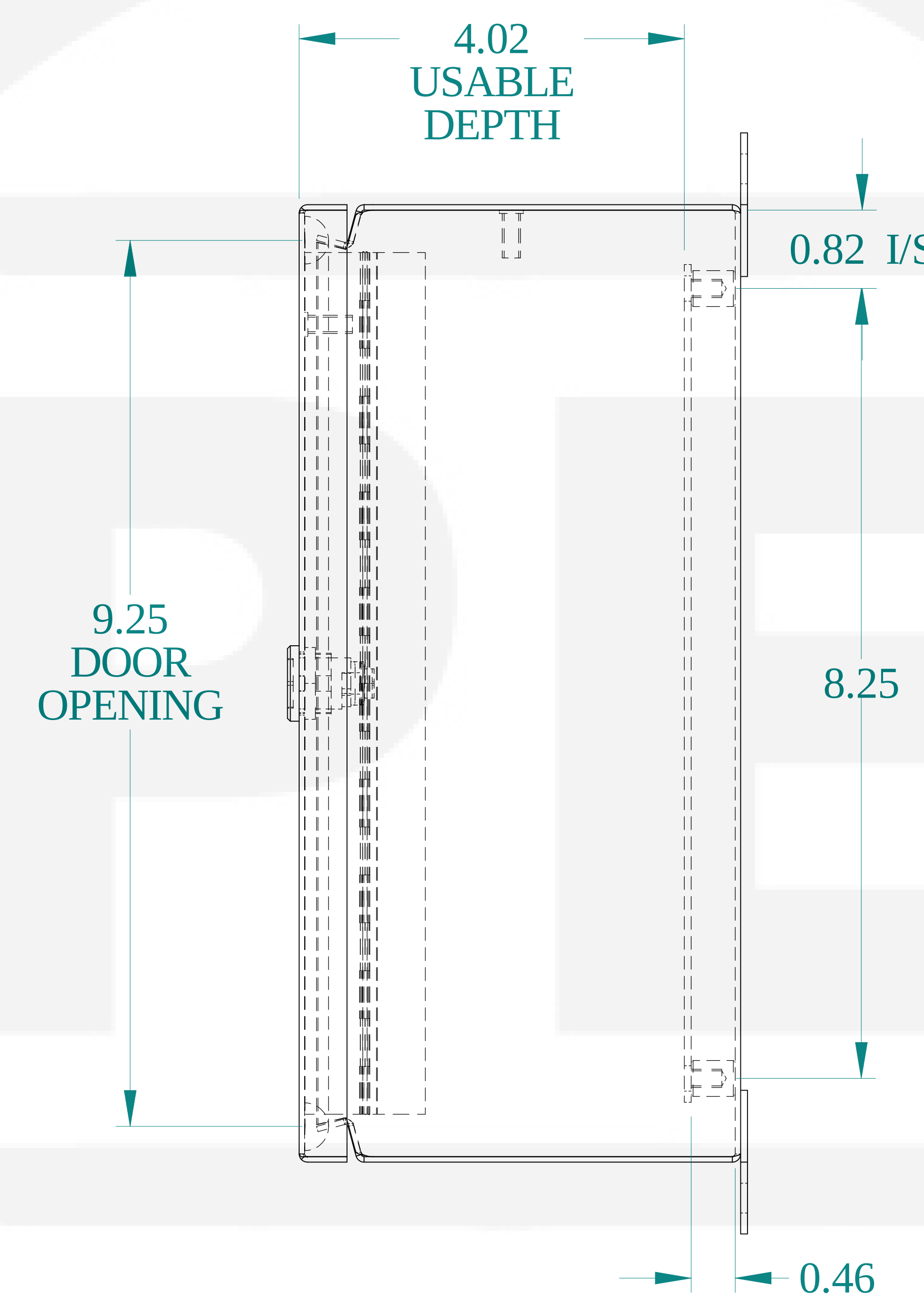
SIDE VIEW
