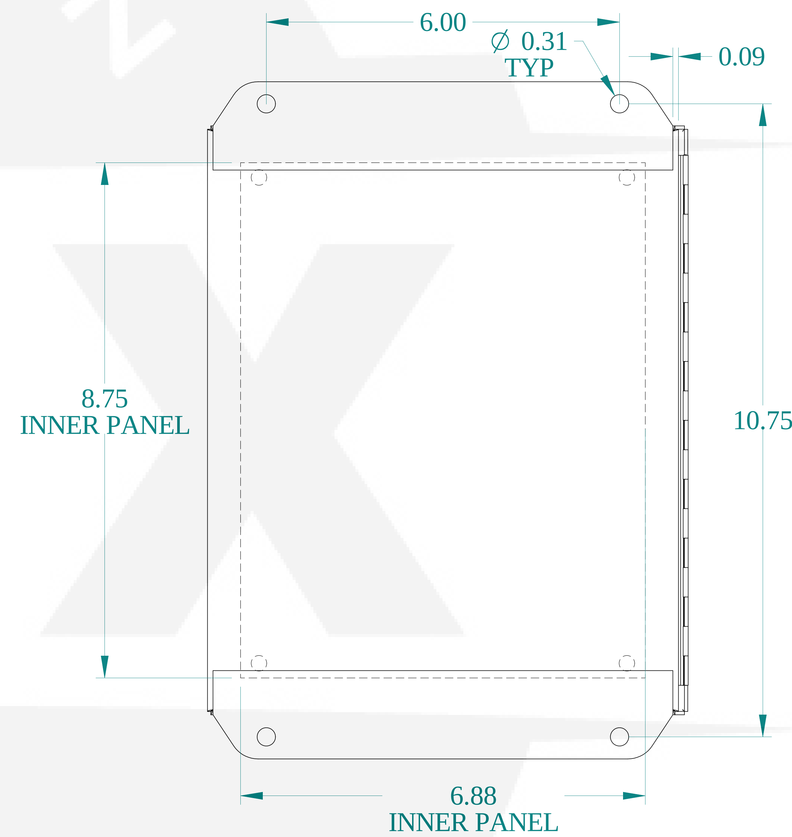
BACK VIEW
