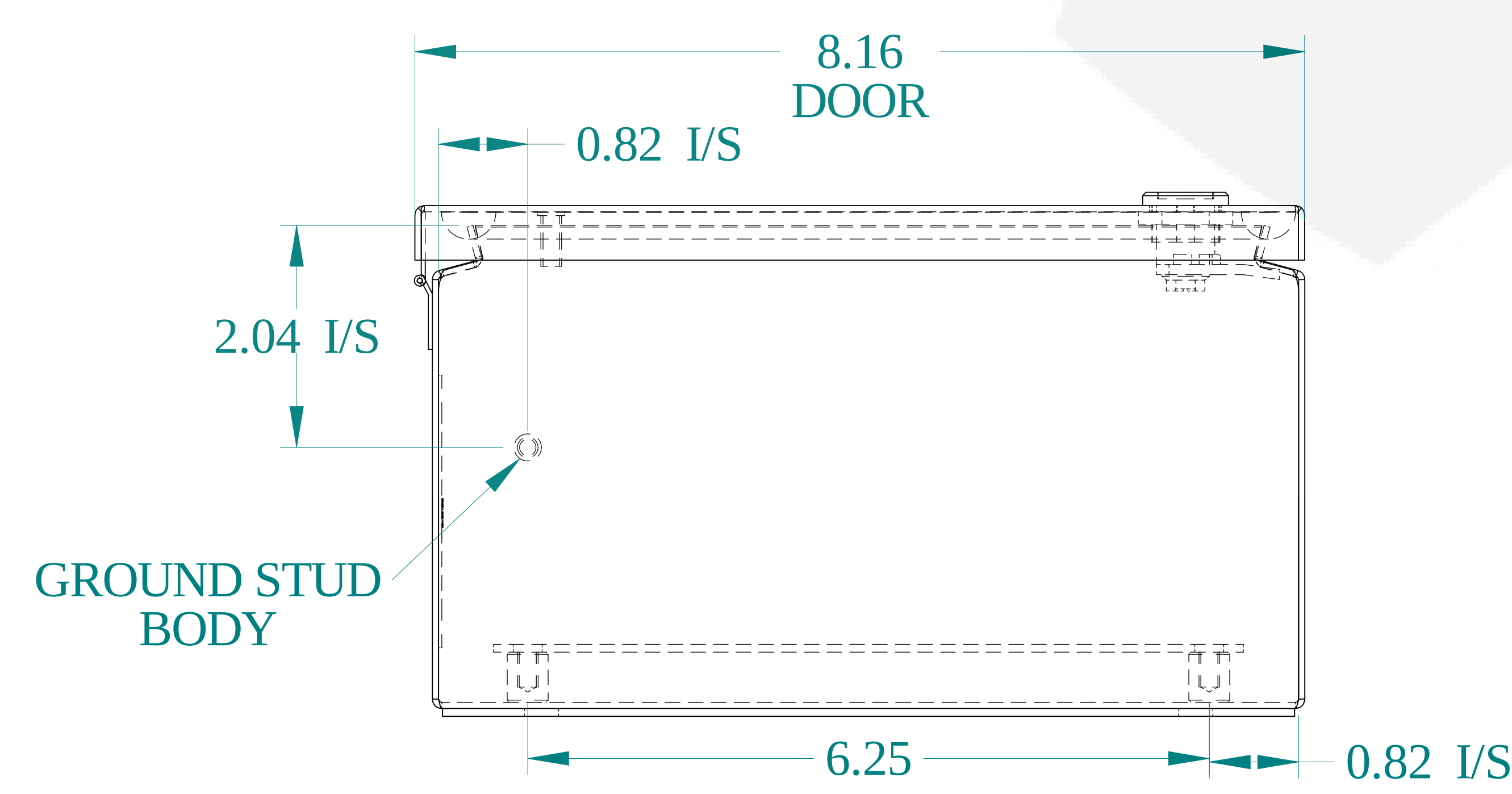
BOTTOM VIEW
