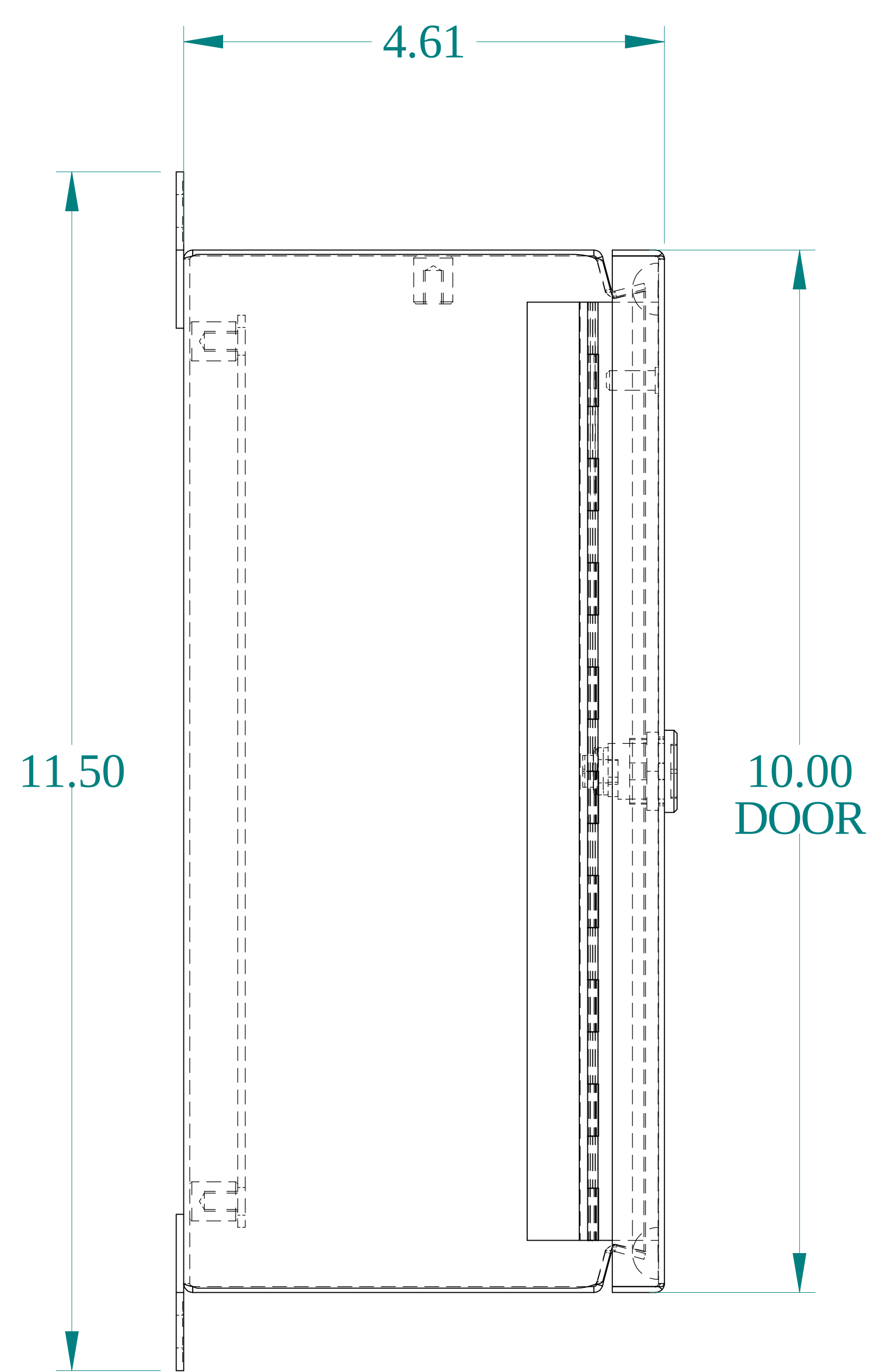
SIDE VIEW
