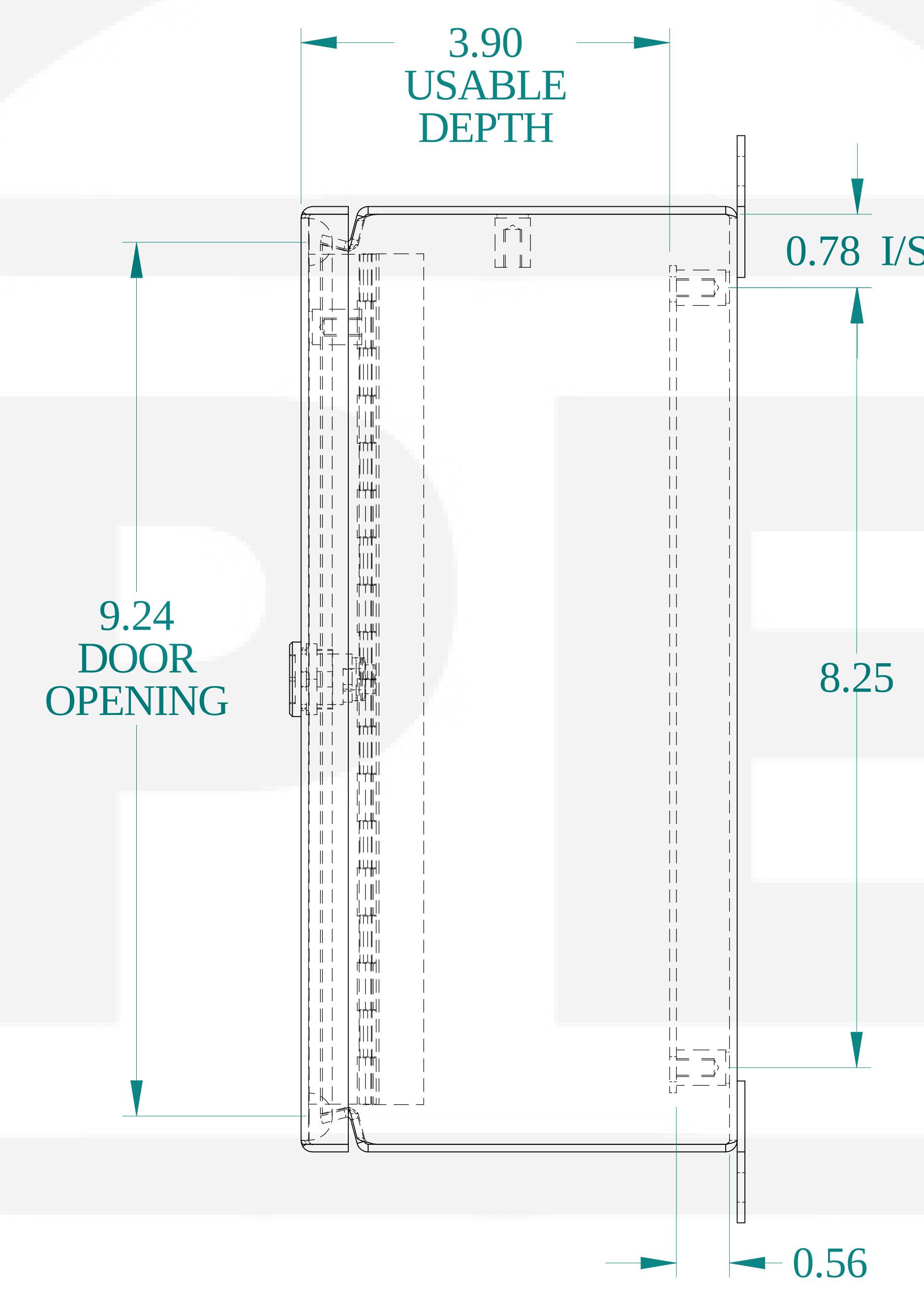
SIDE VIEW
