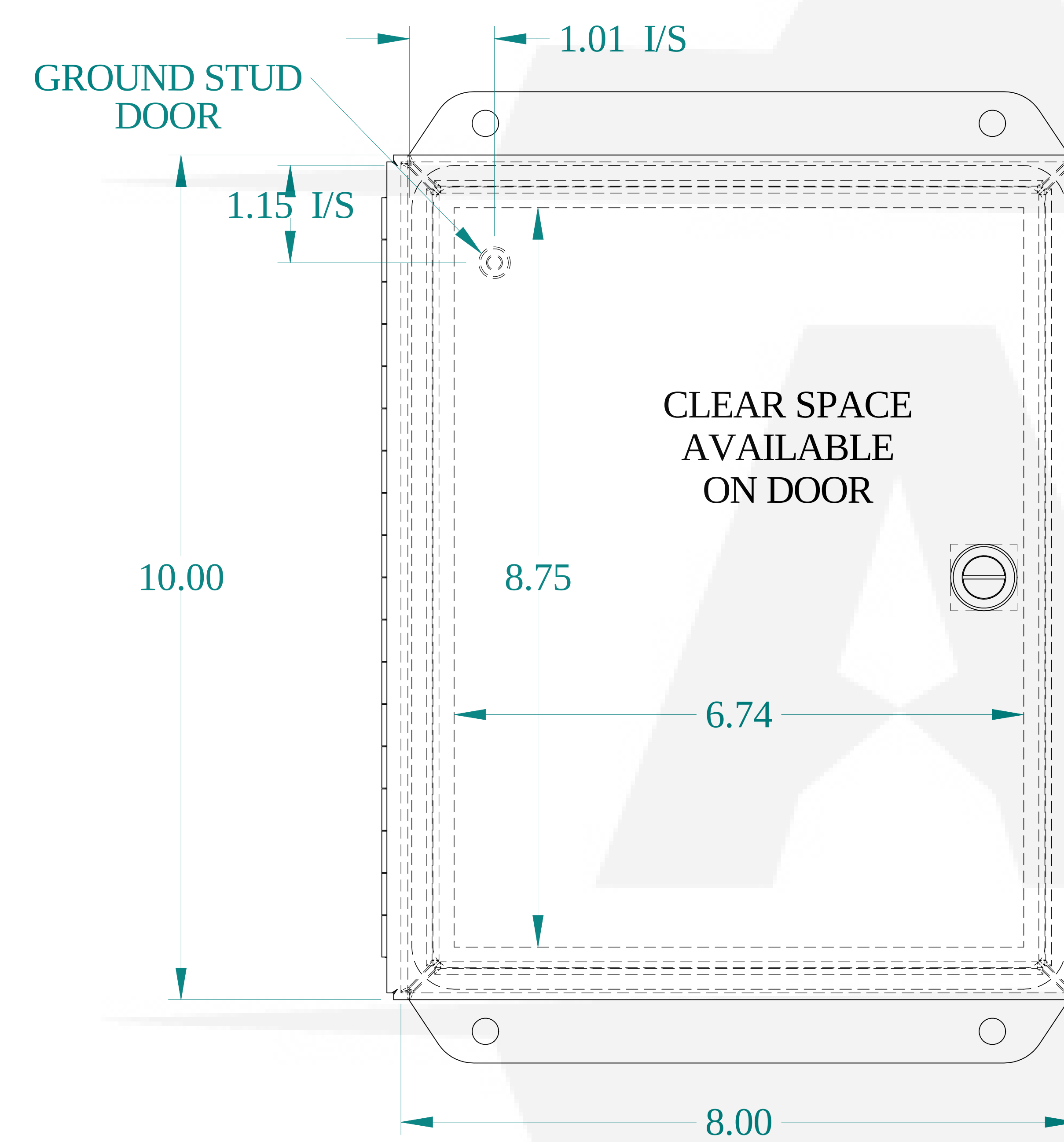
FRONT VIEW
