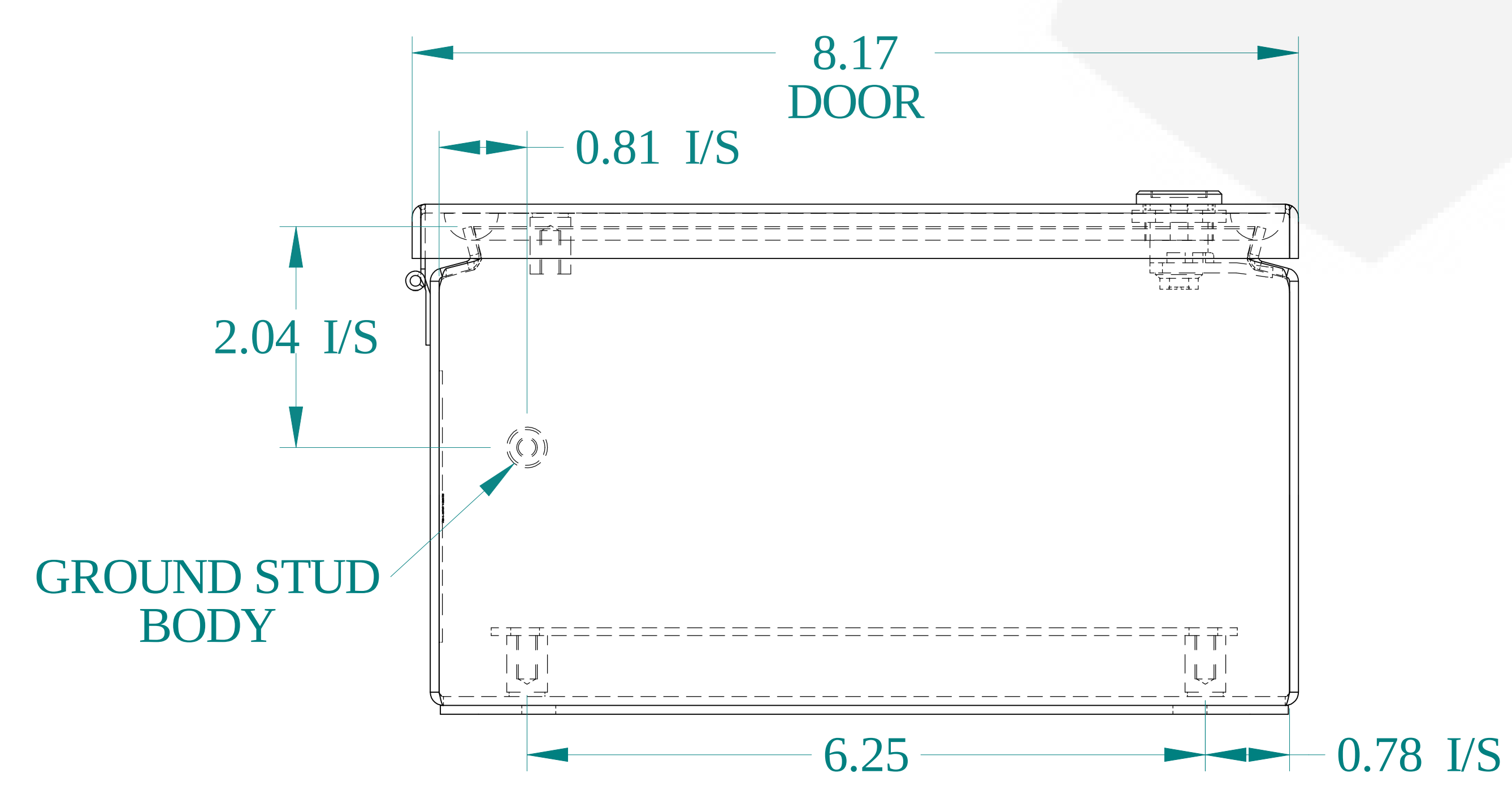
BOTTOM VIEW
