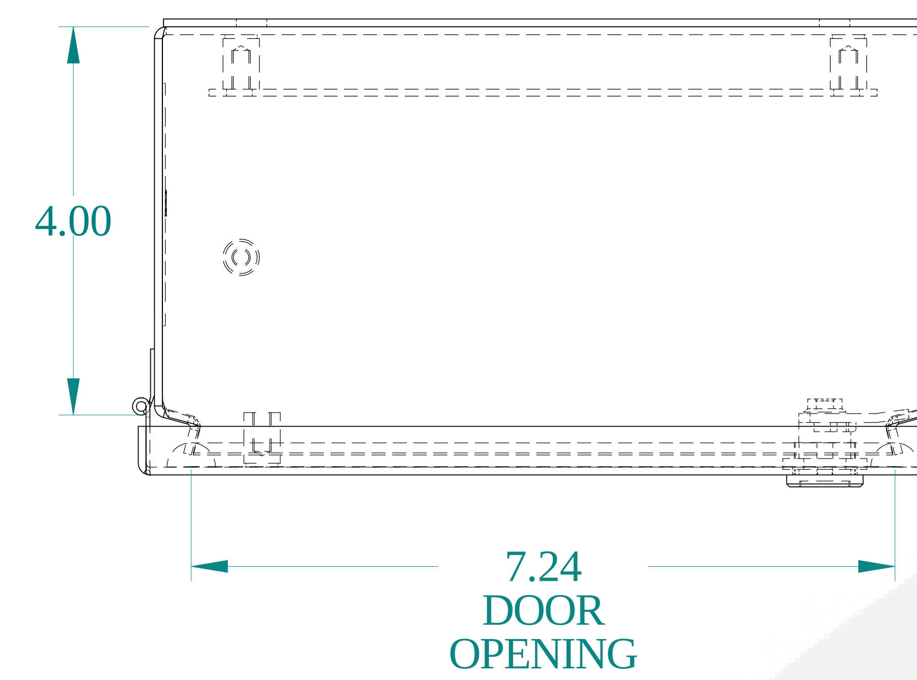
TOP VIEW
