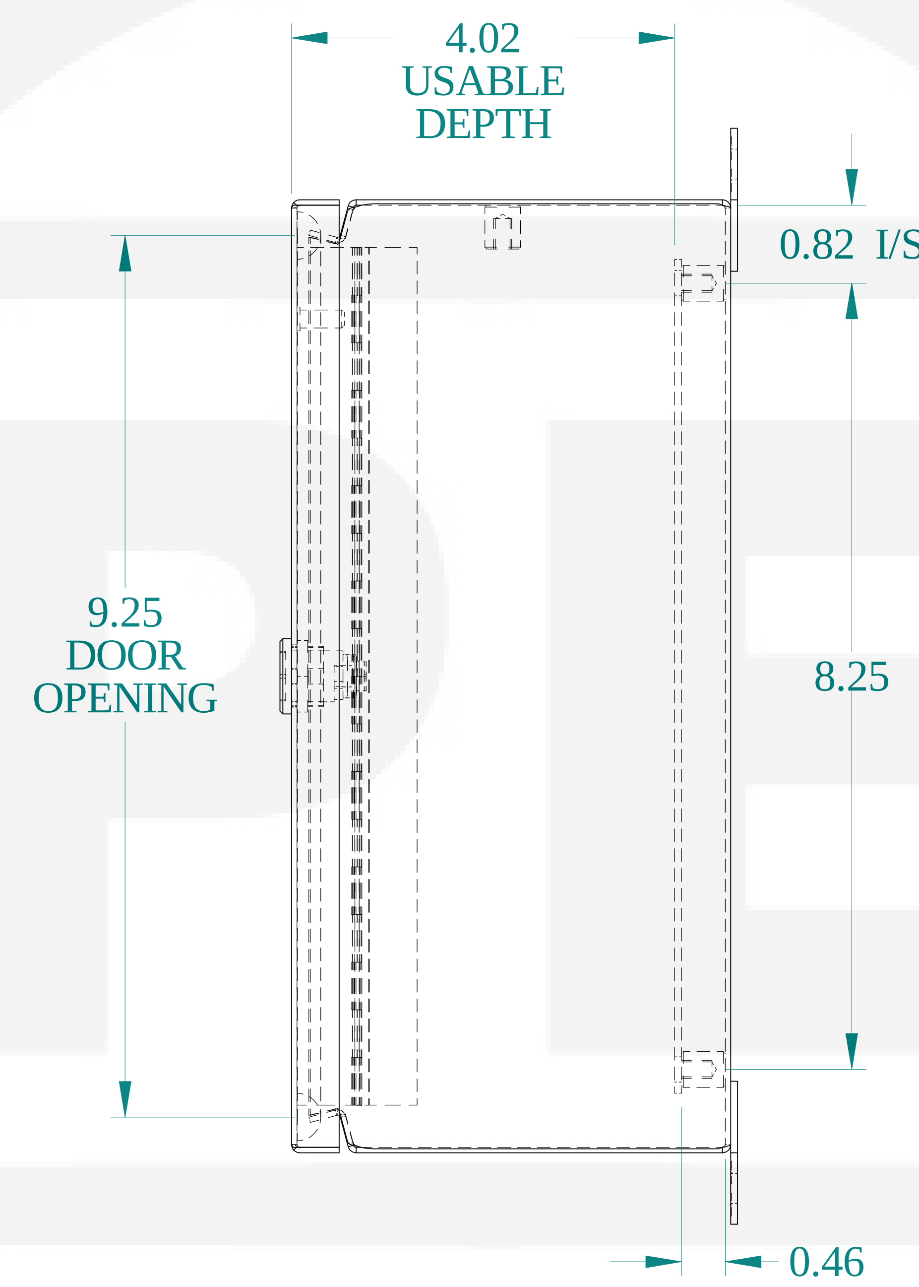
SIDE VIEW
