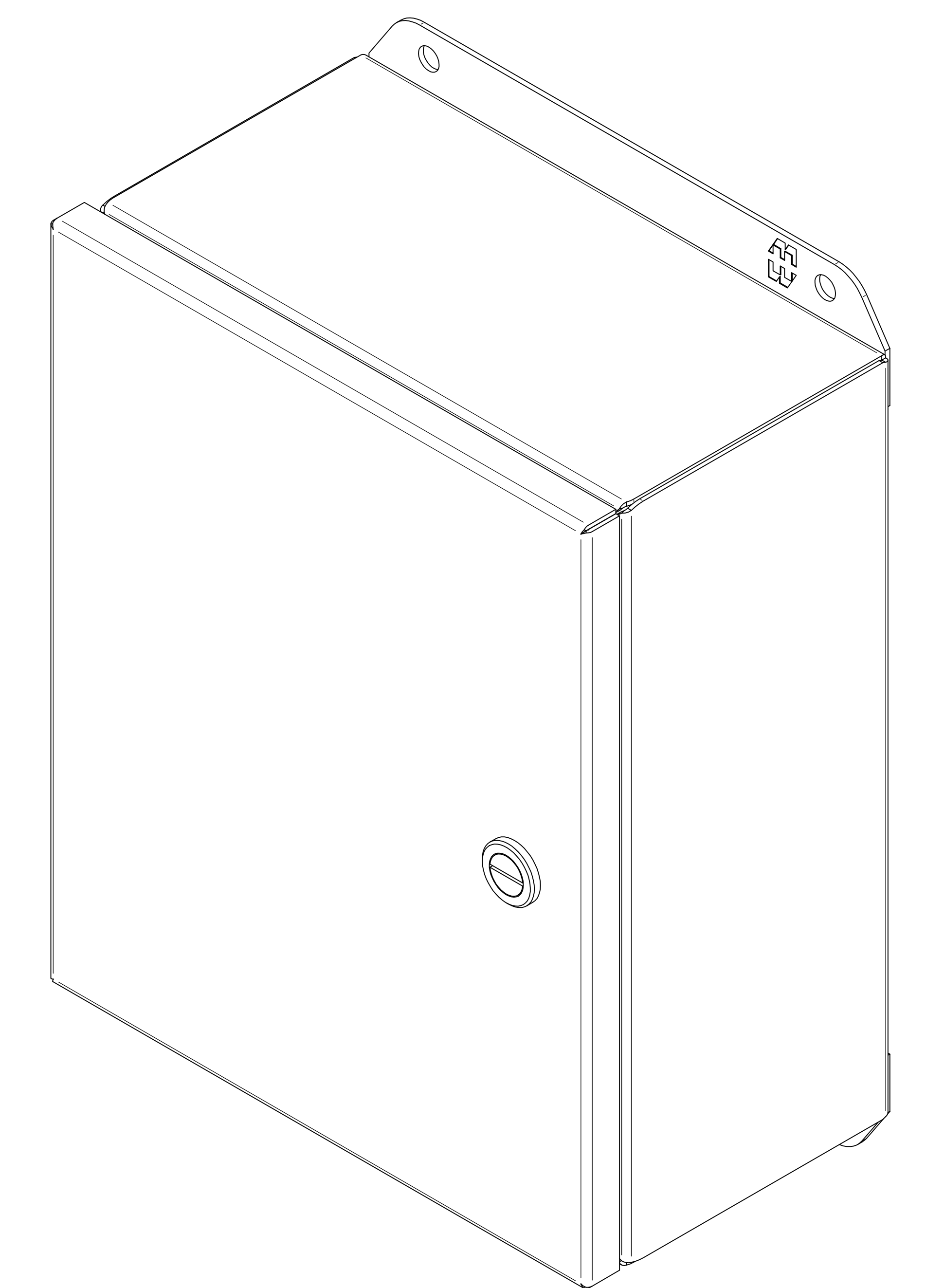
ISOMETRIC VIEWS
