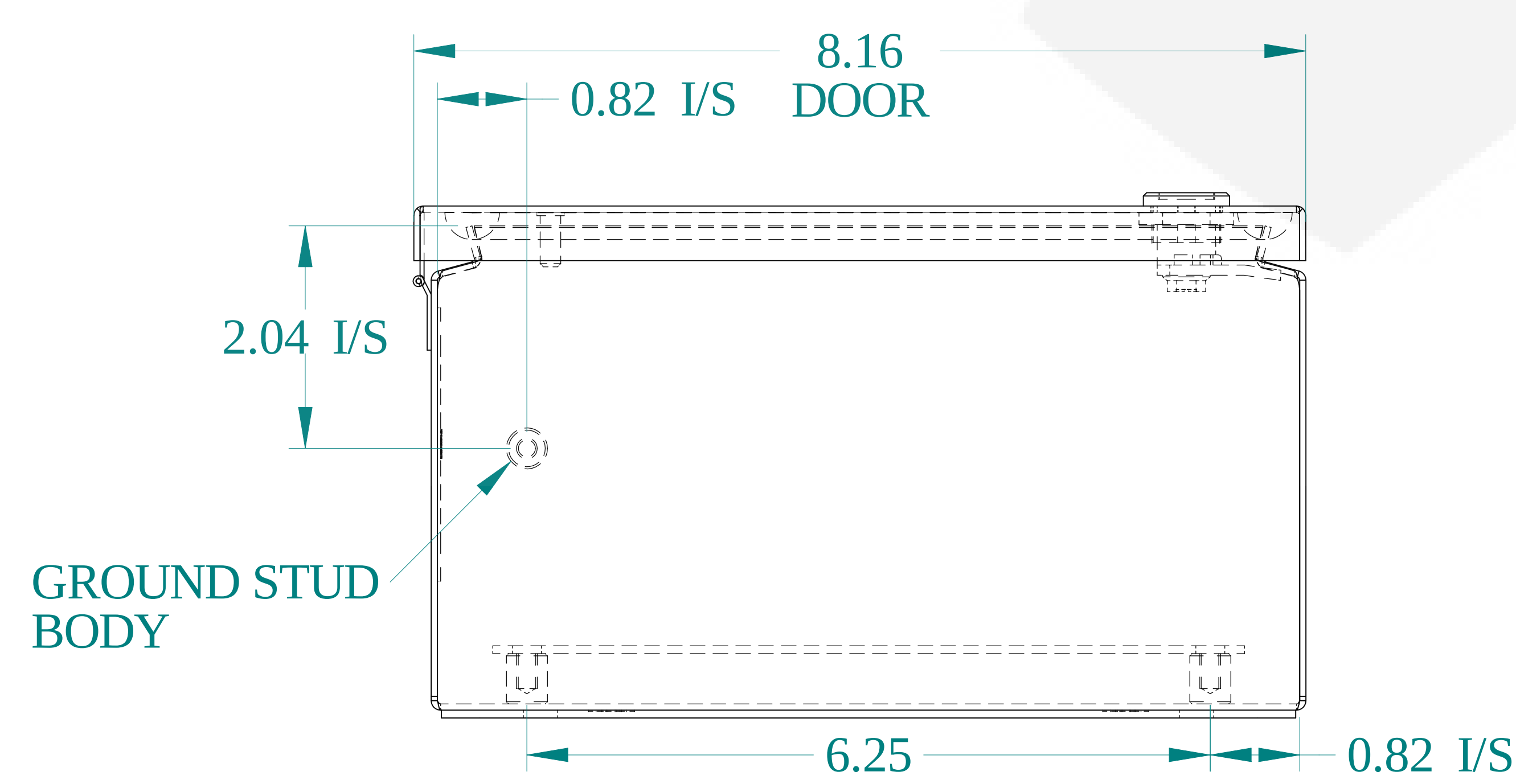
BOTTOM VIEW
