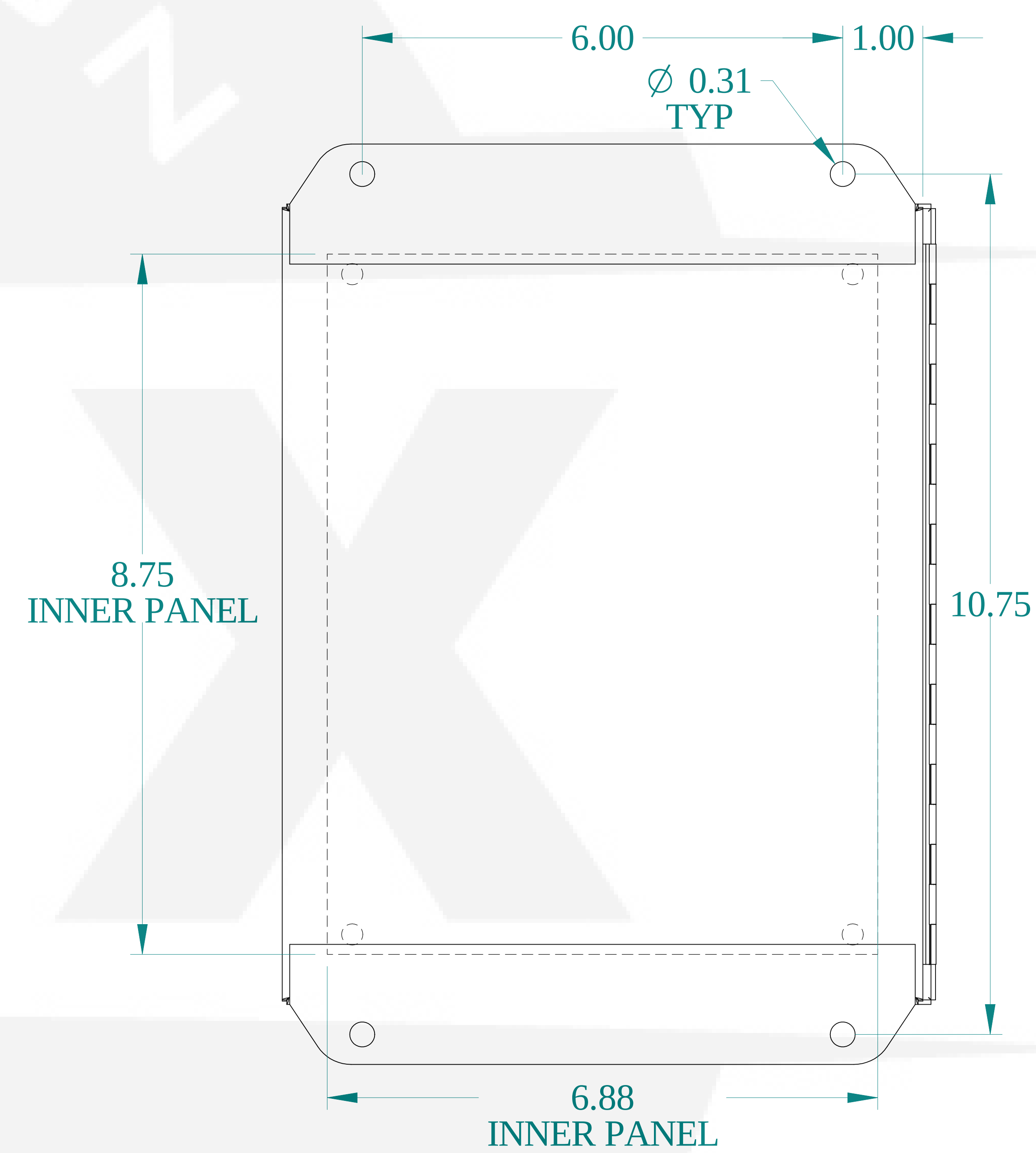
BACK VIEW
