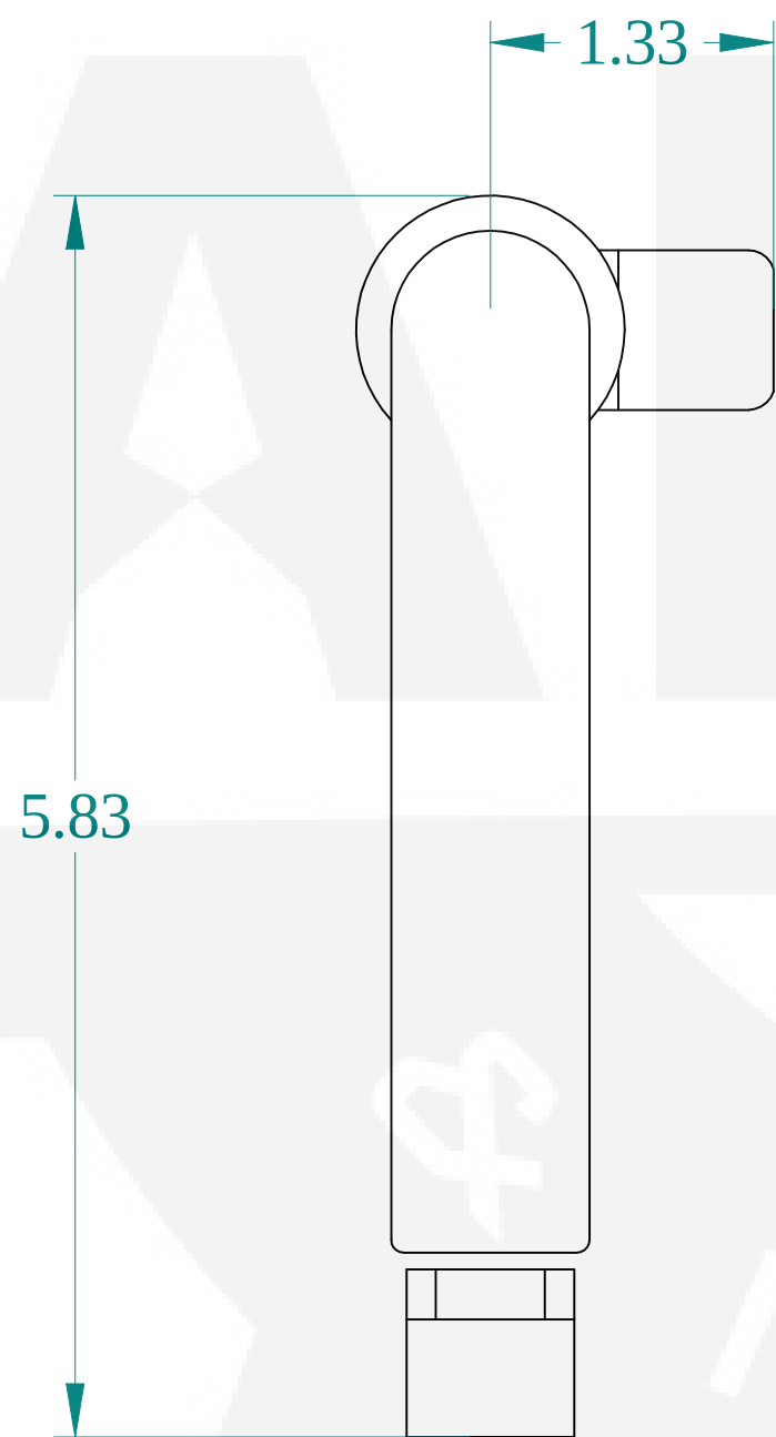
FRONT VIEW
