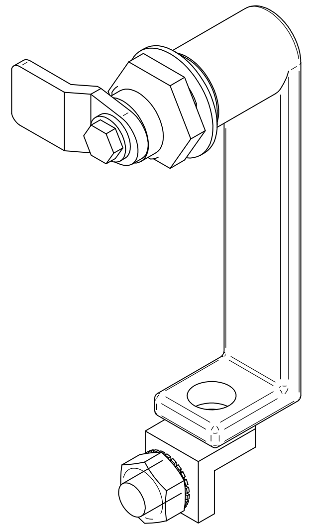
ISOMETRIC VIEWS
