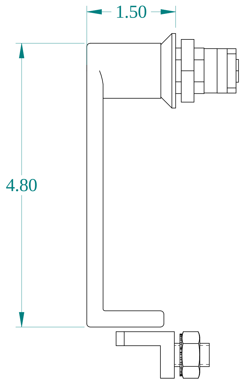
SIDE VIEW
