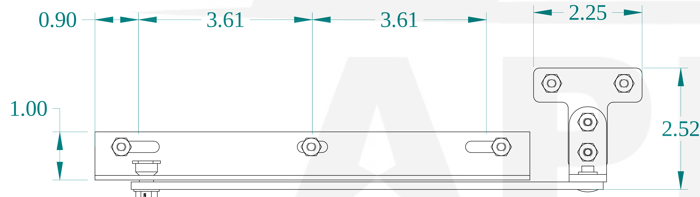
FRONT VIEW
