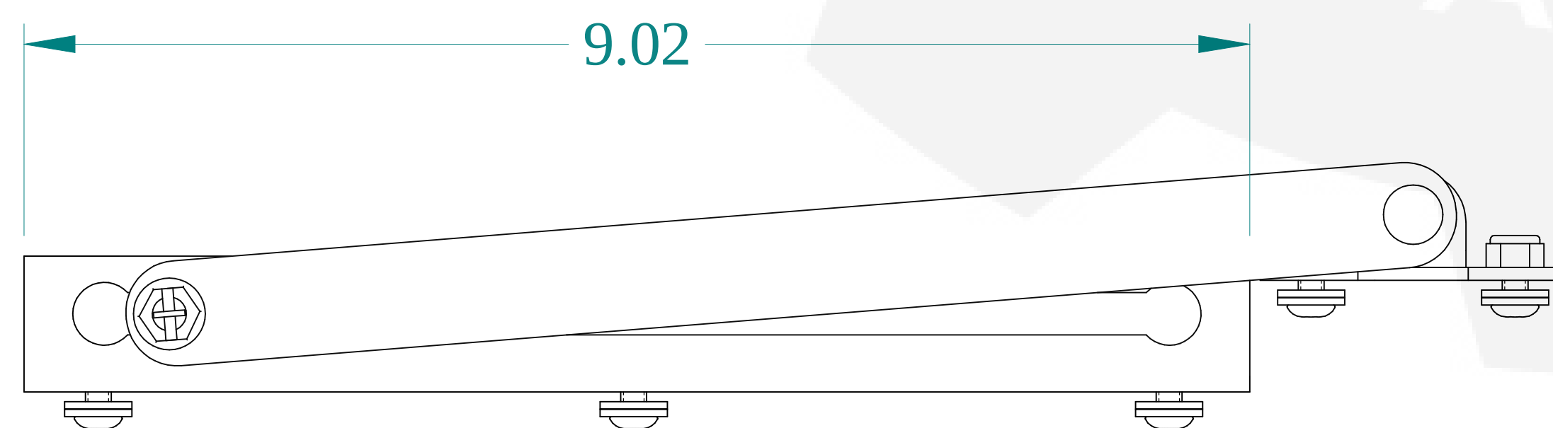
BOTTOM VIEW
