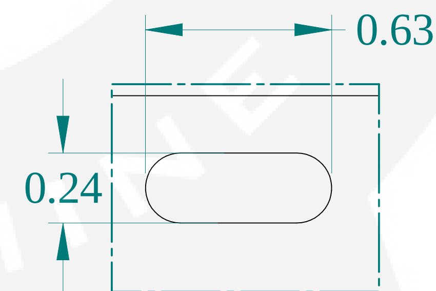
DETAIL Z
