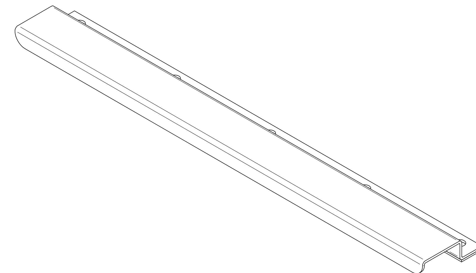
ISOMETRIC VIEW
