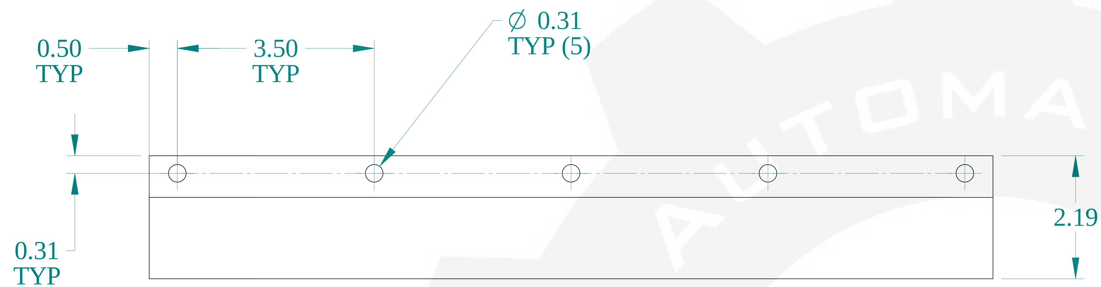
TOP VIEW
