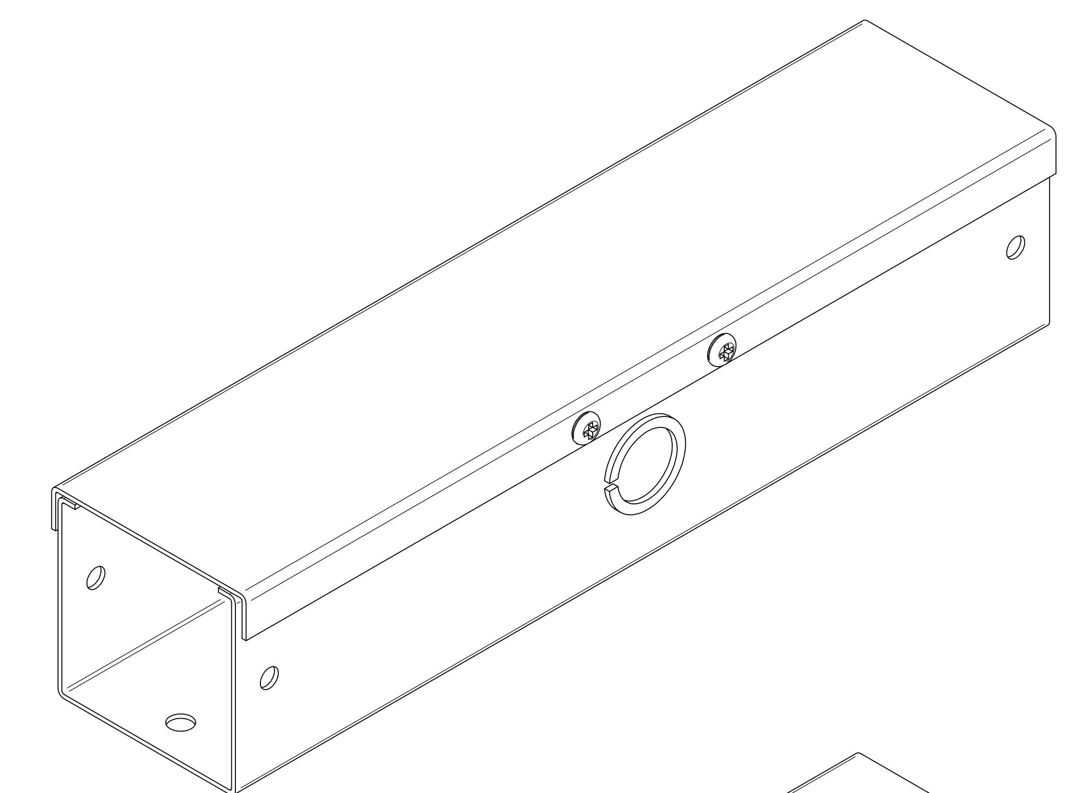
ISOMETRIC VIEWS
