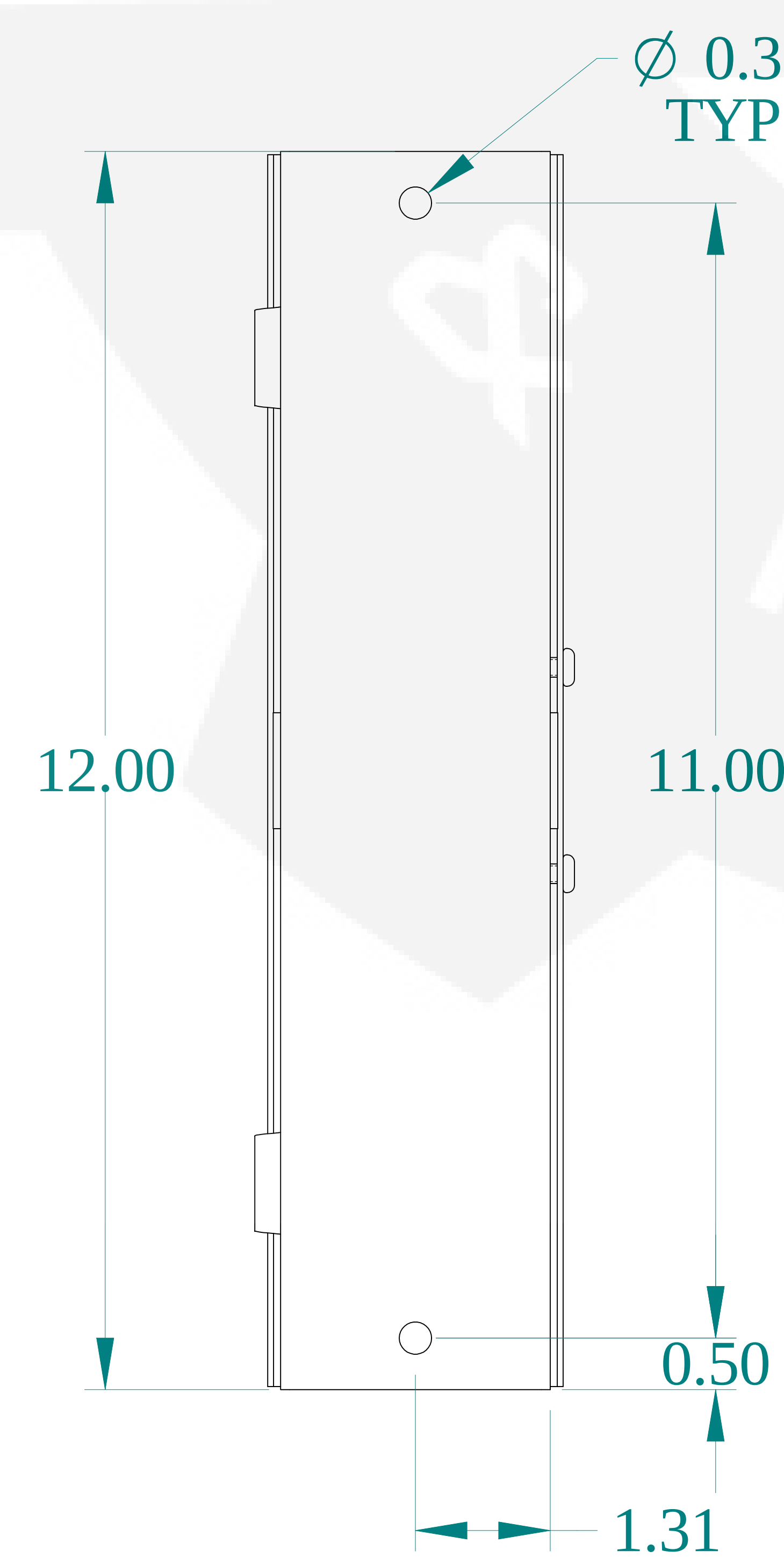
BOTTOM VIEW
