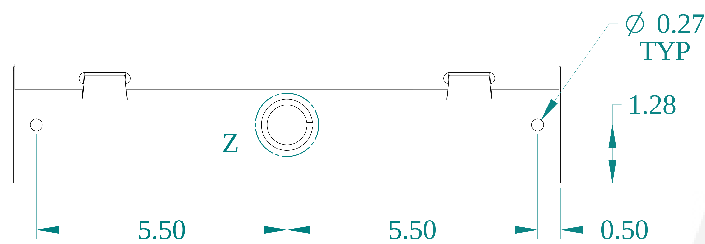
SIDE VIEW
