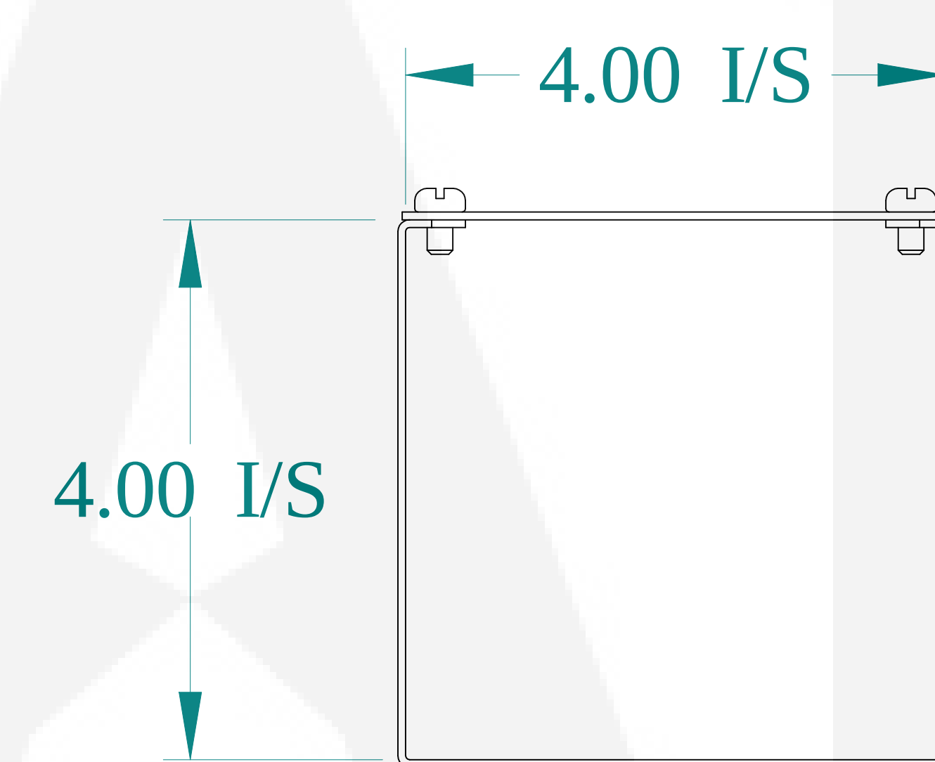
FRONT VIEW
