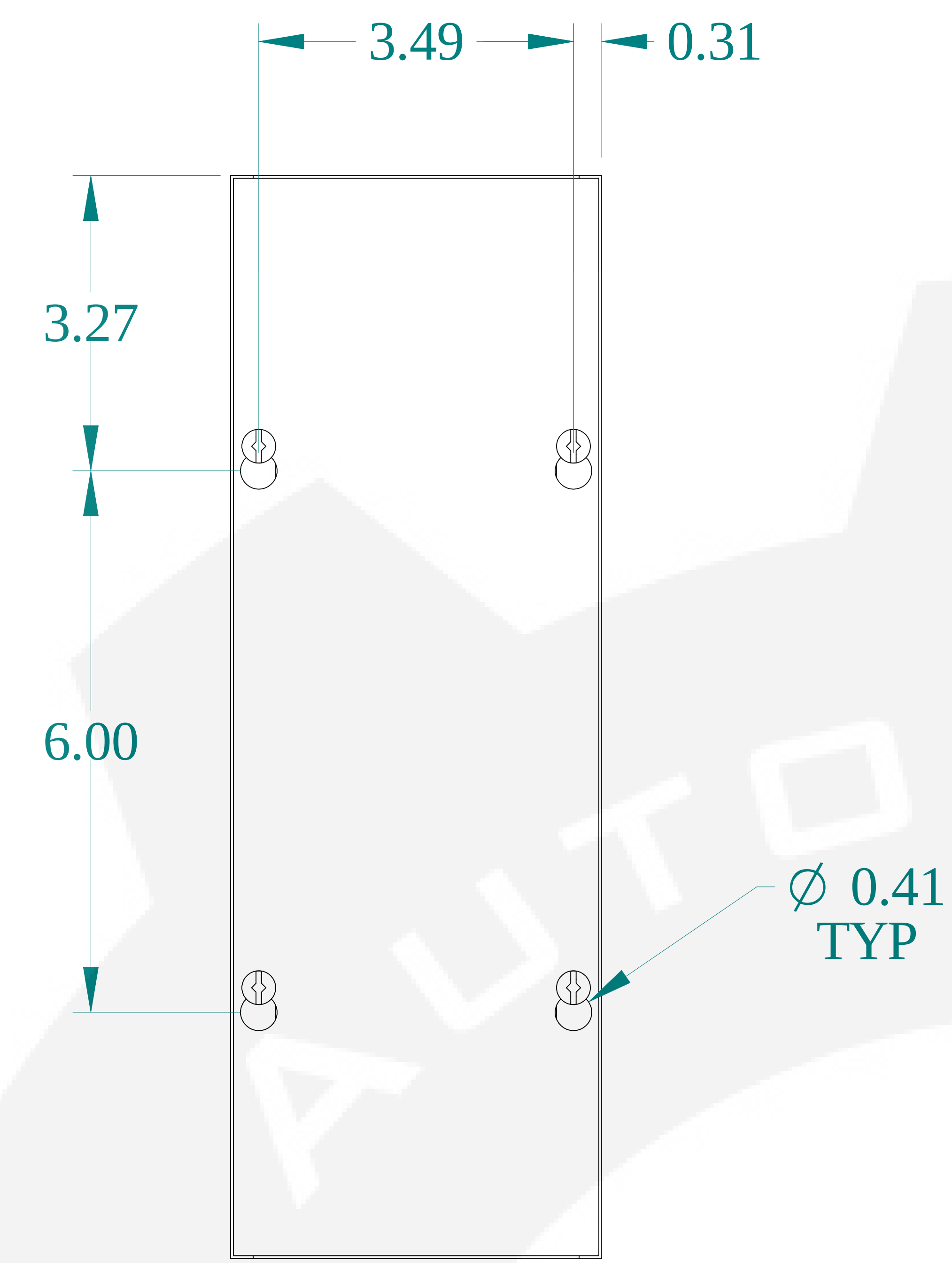
TOP VIEW
