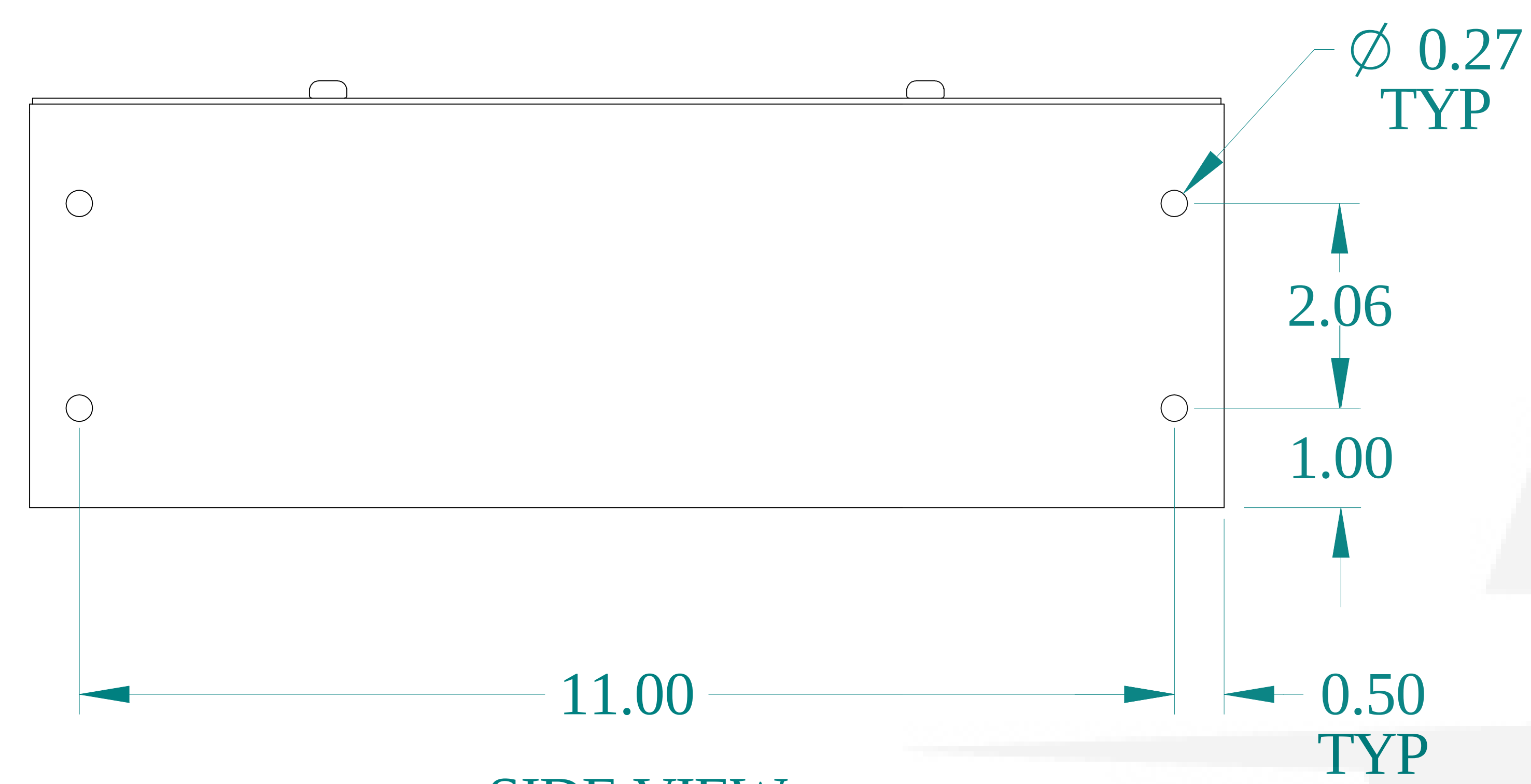
SIDE VIEW
