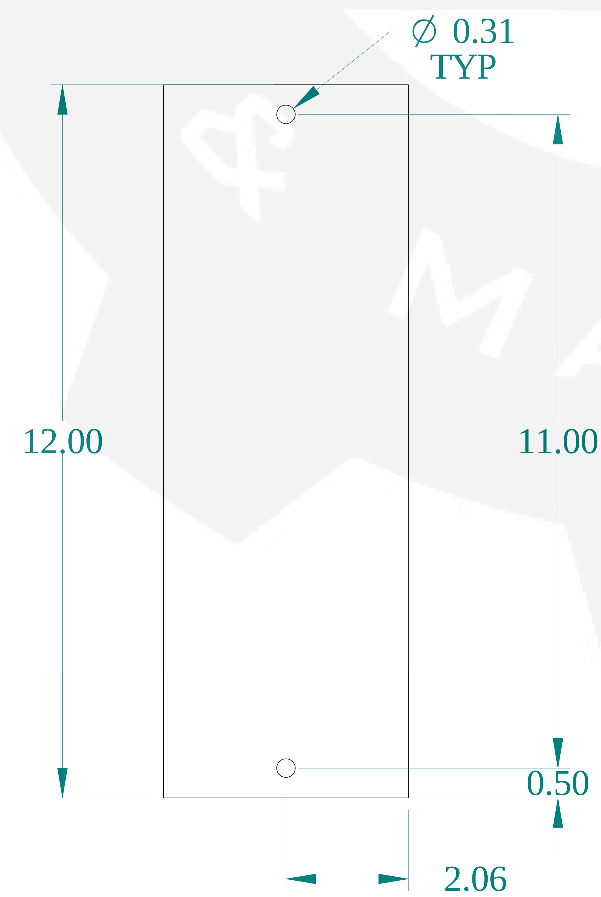
BOTTOM VIEW
