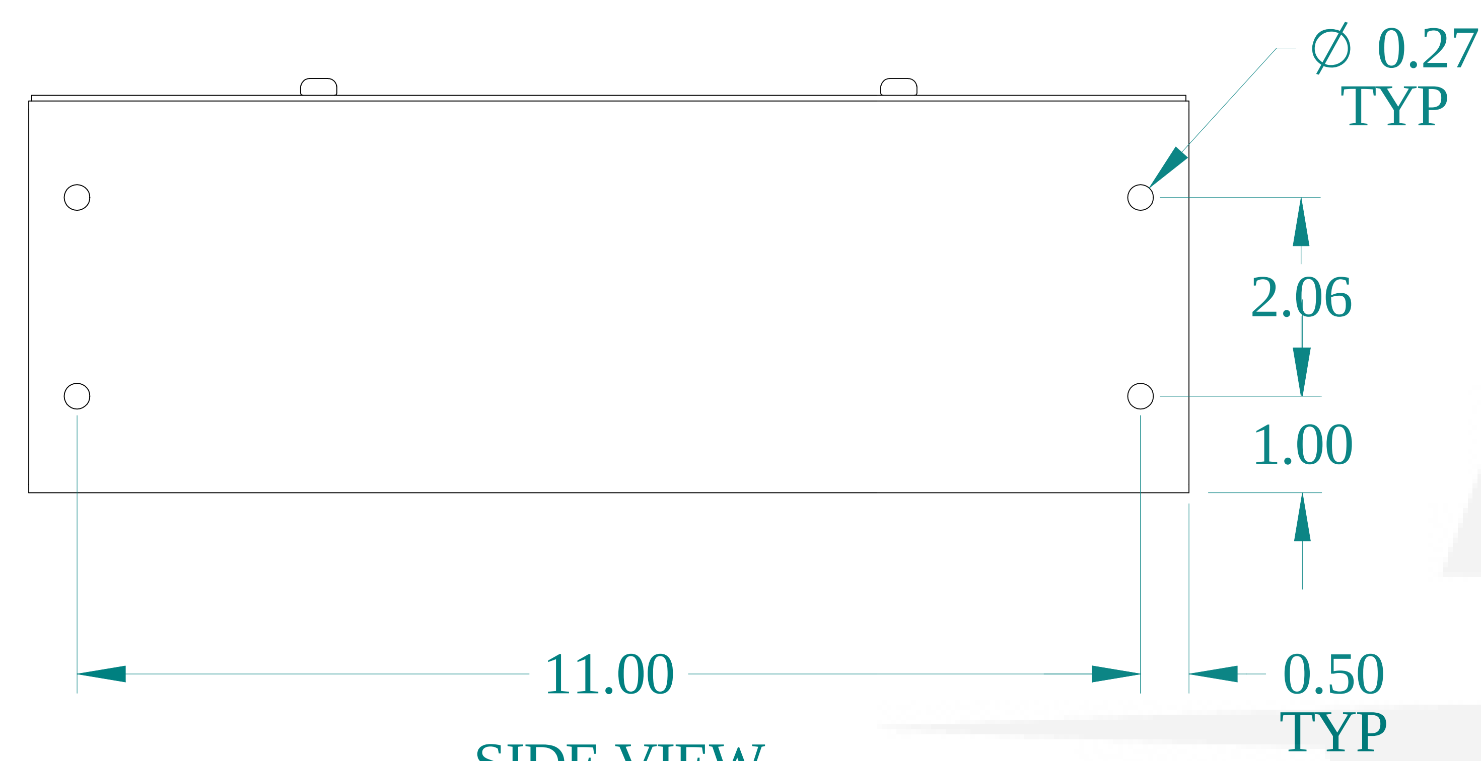
SIDE VIEW
