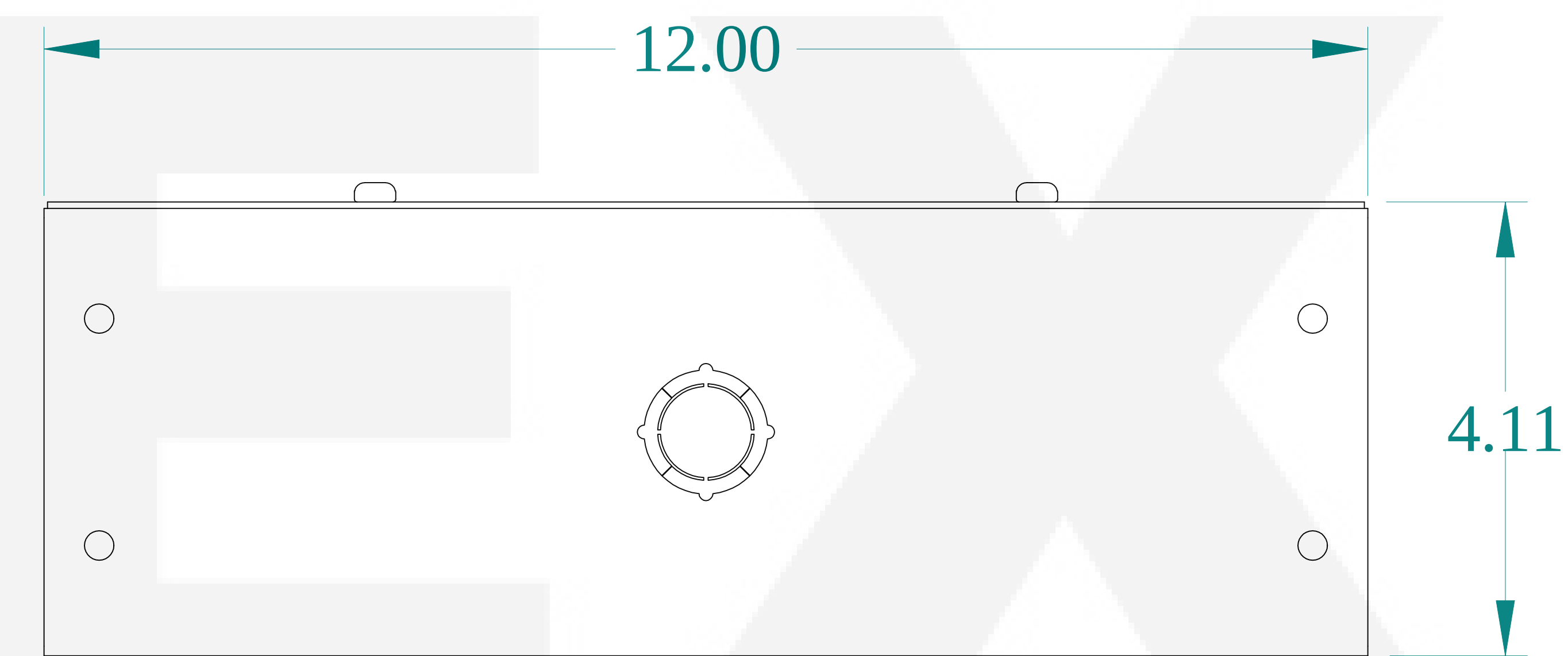
SIDE VIEW
