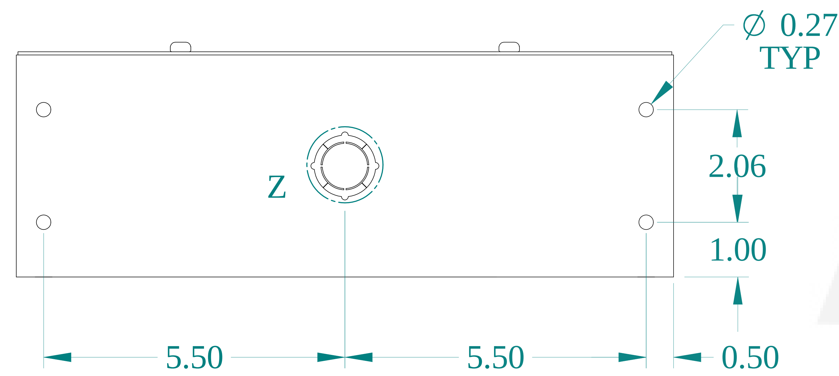
SIDE VIEW
