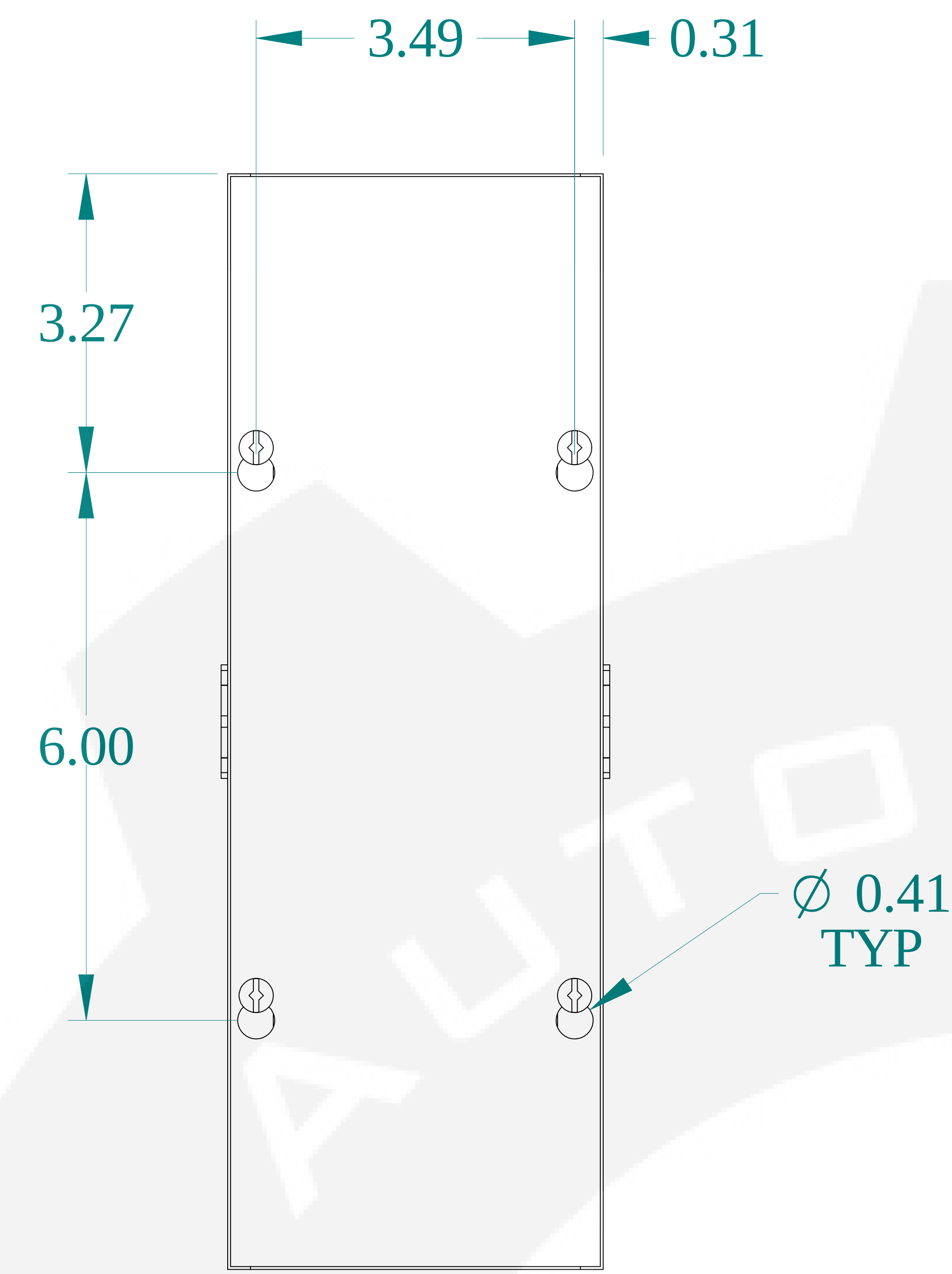
TOP VIEW
