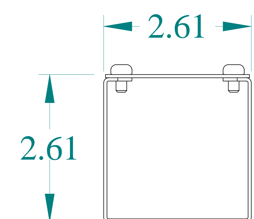
BACK VIEW
