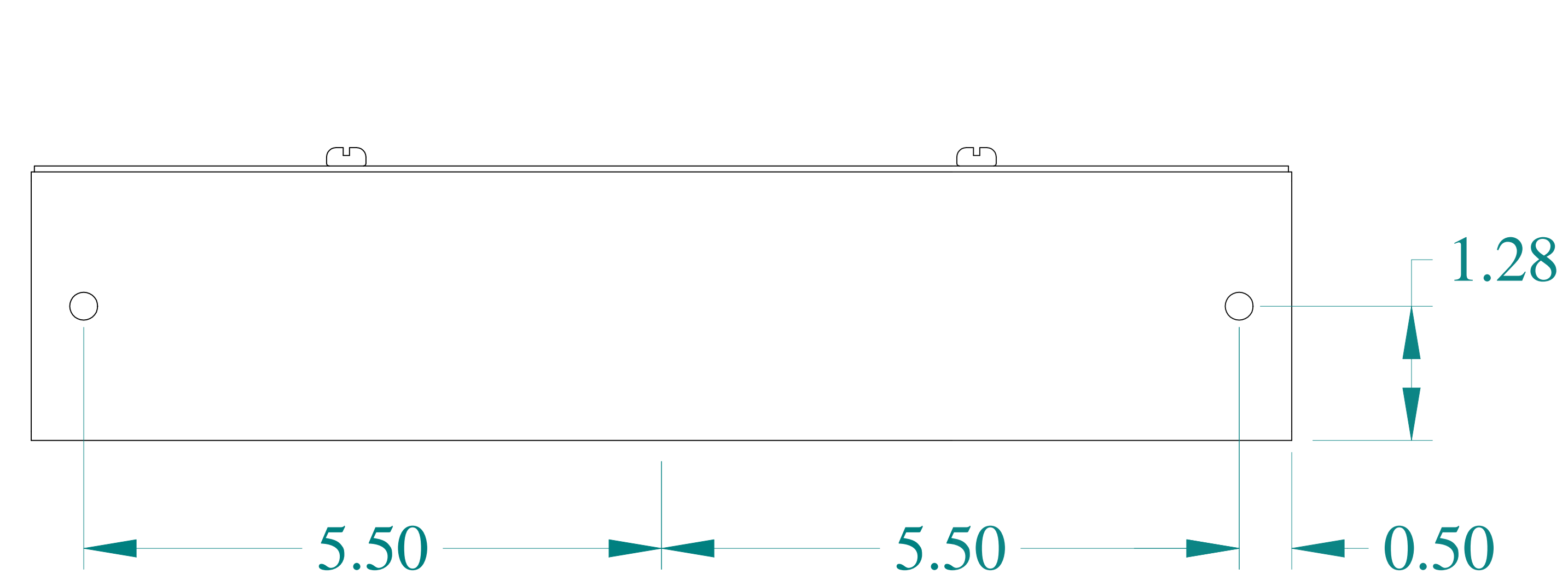
SIDE VIEW
