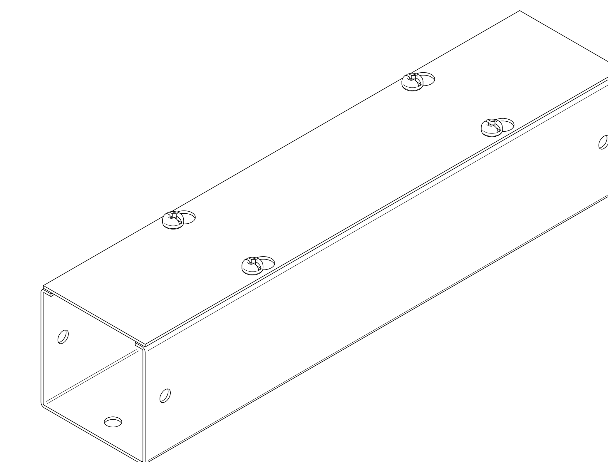
ISOMETRIC VIEWS
