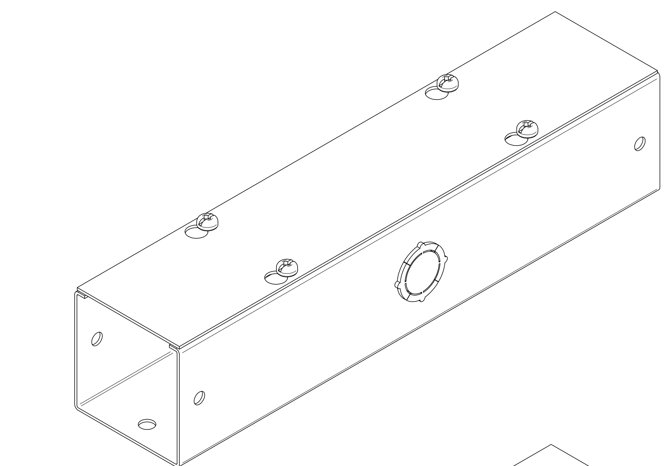
ISOMETRIC VIEWS
