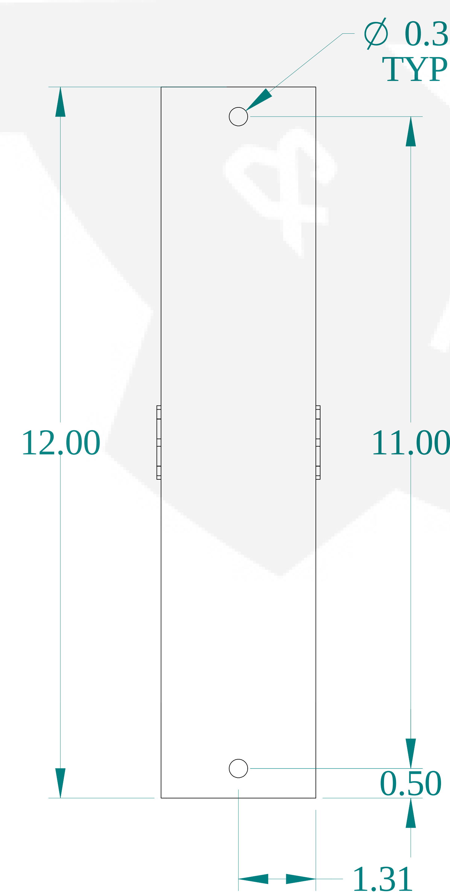
BOTTOM VIEW
