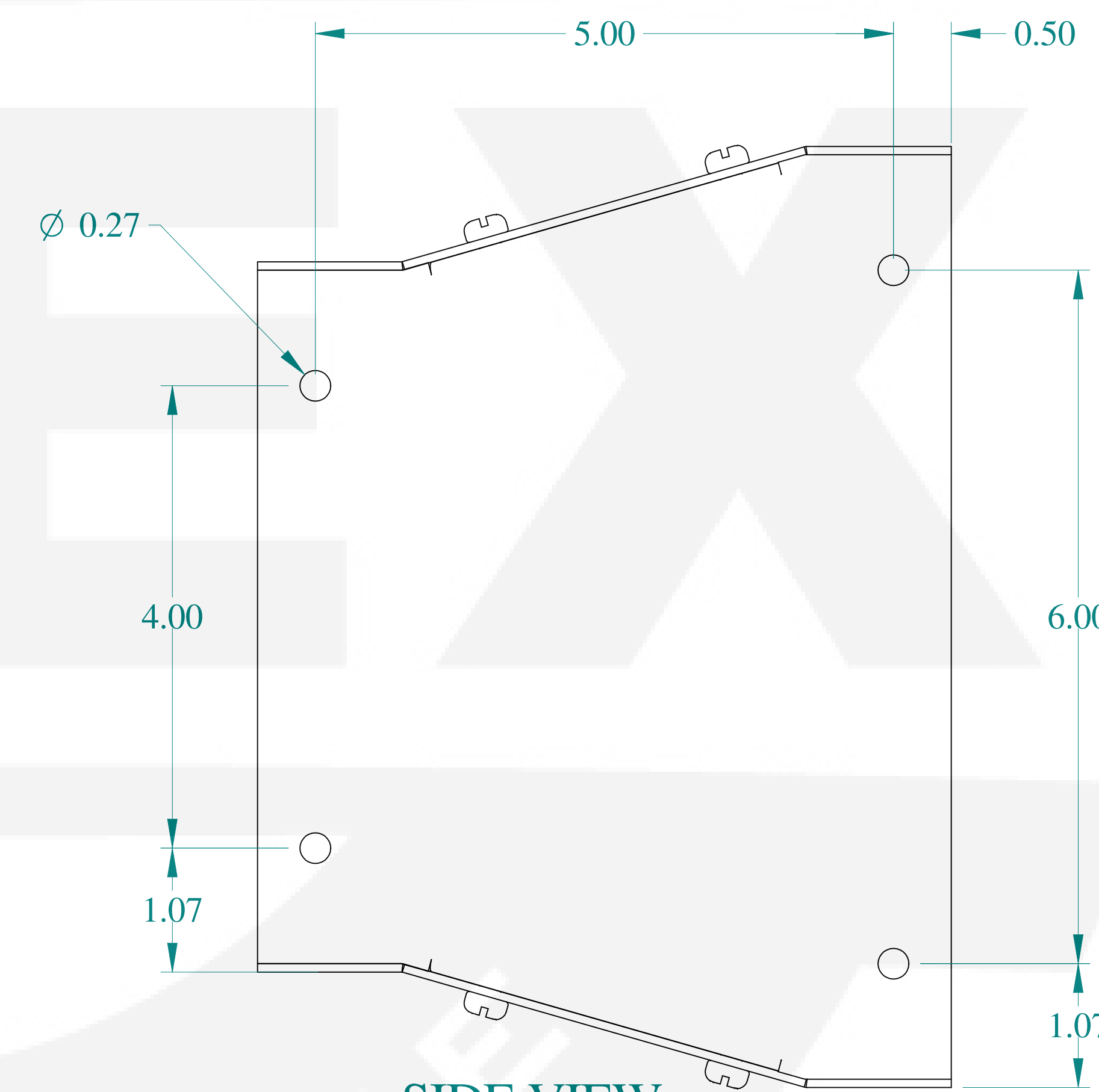
SIDE VIEW
