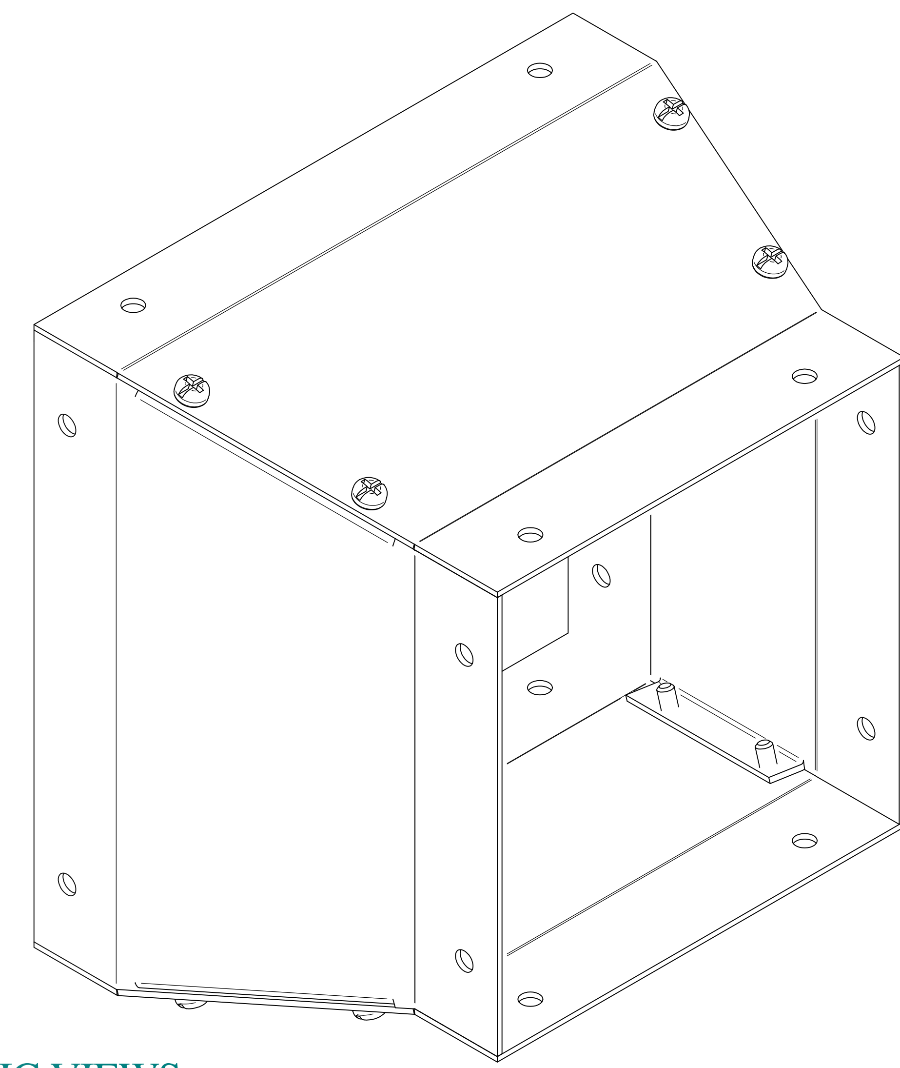
ISOMETRIC VIEWS
