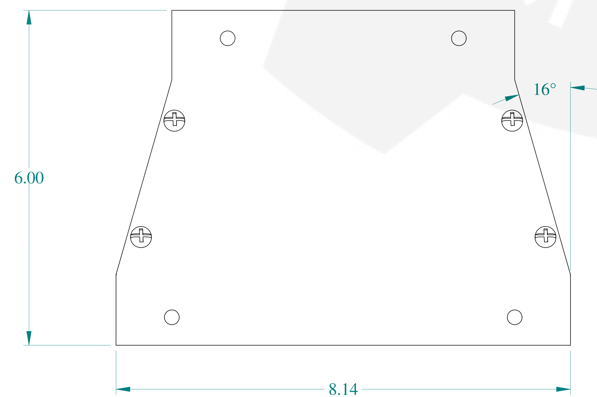
BOTTOM VIEW
