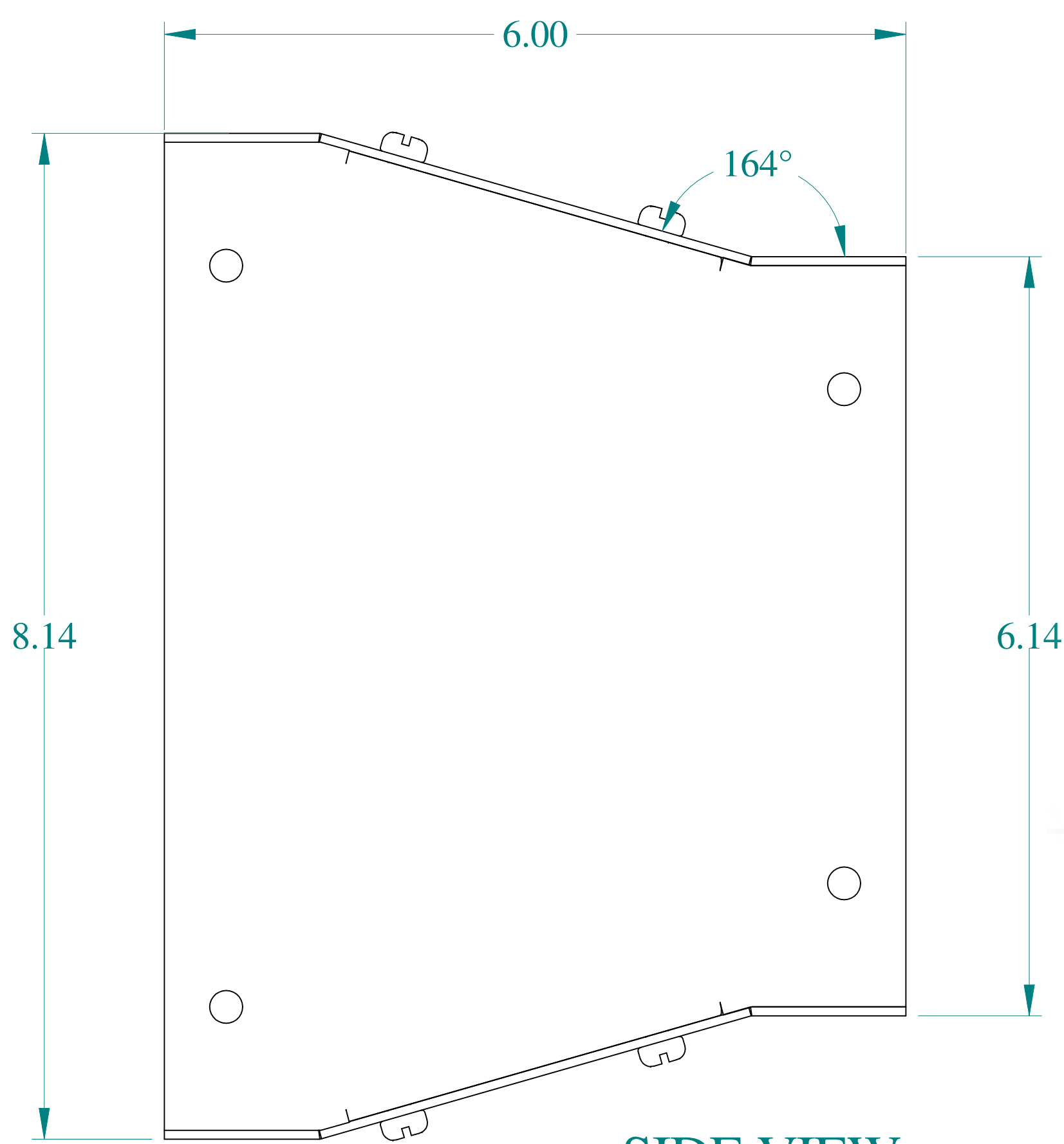
SIDE VIEW
