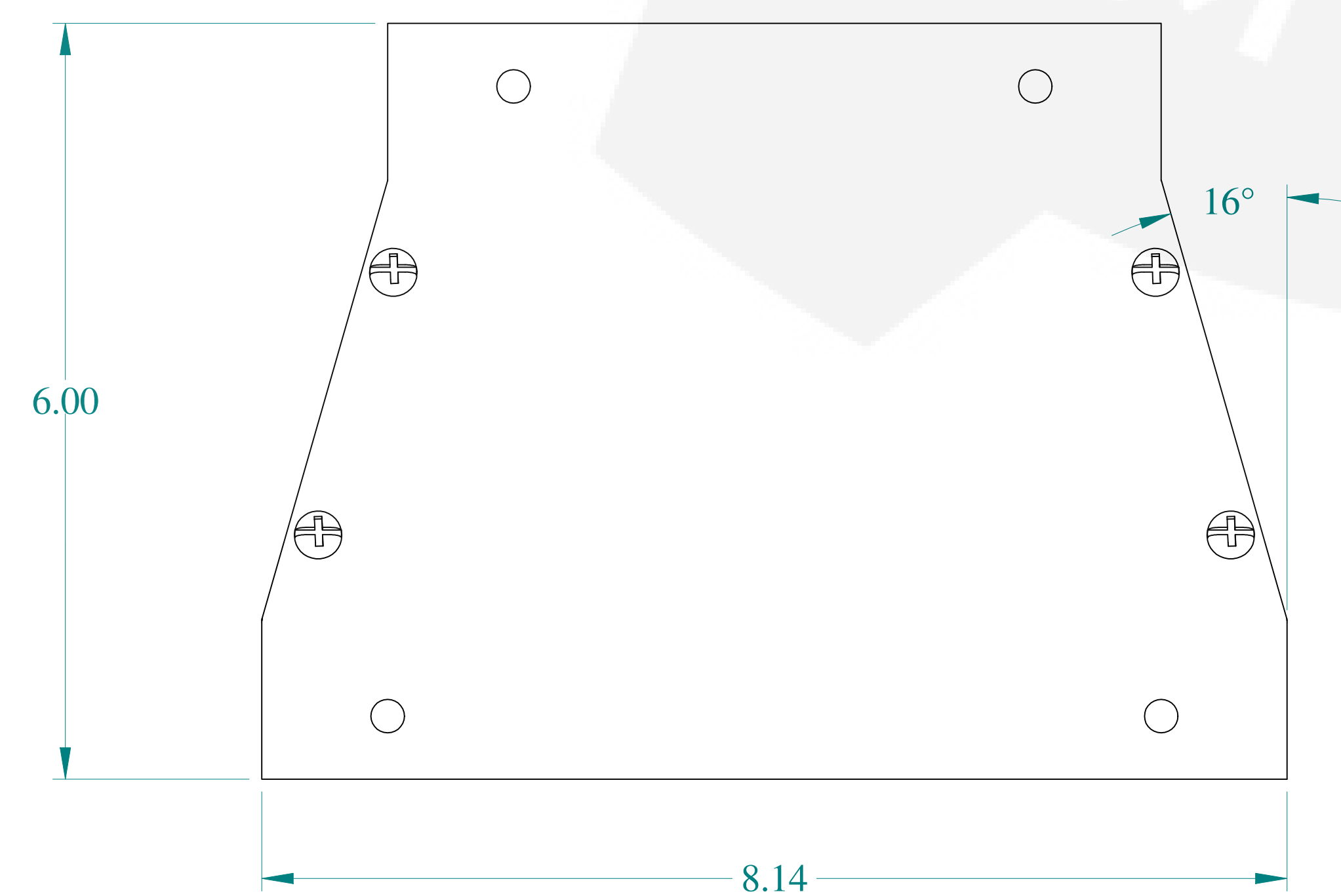
BOTTOM VIEW
