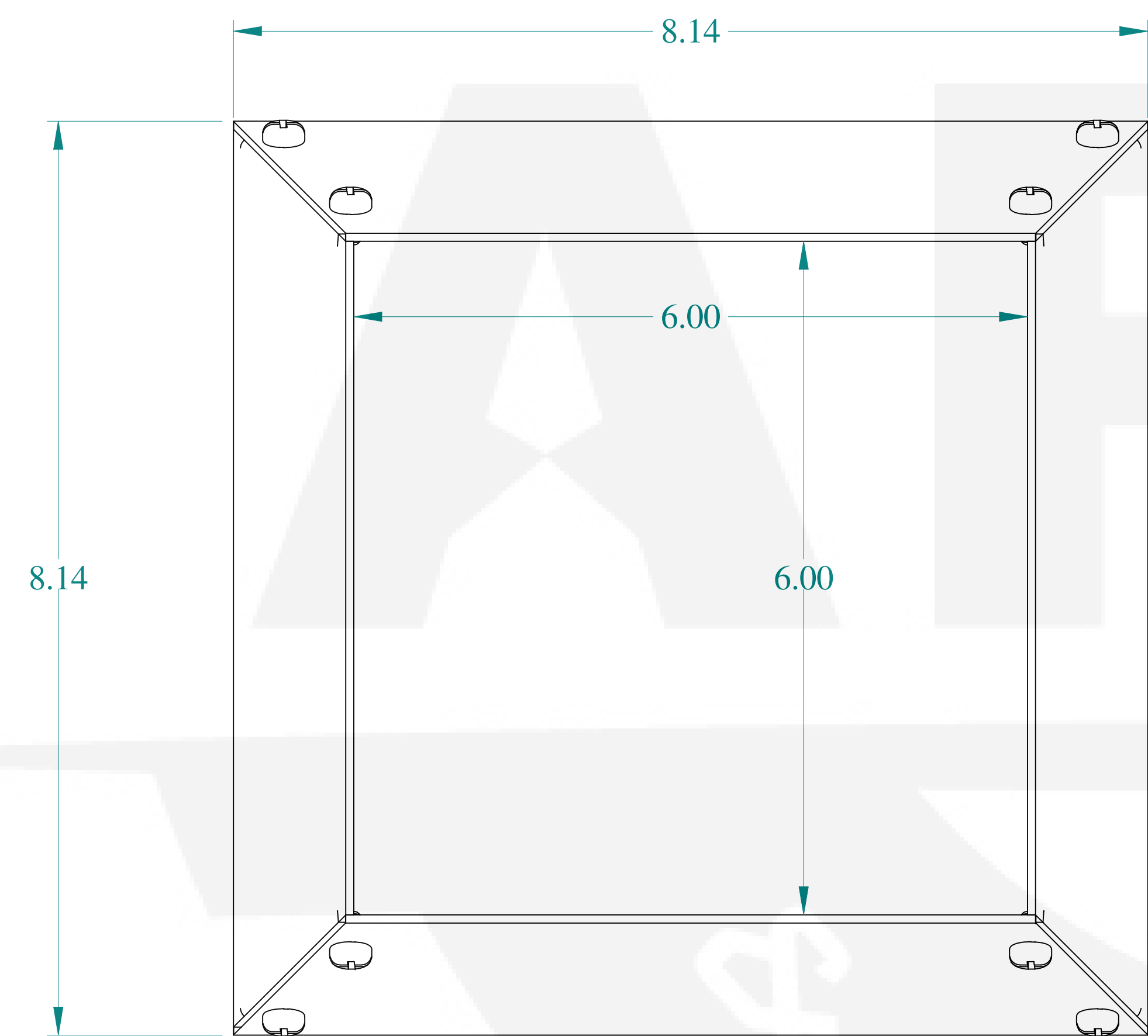
FRONT VIEW
