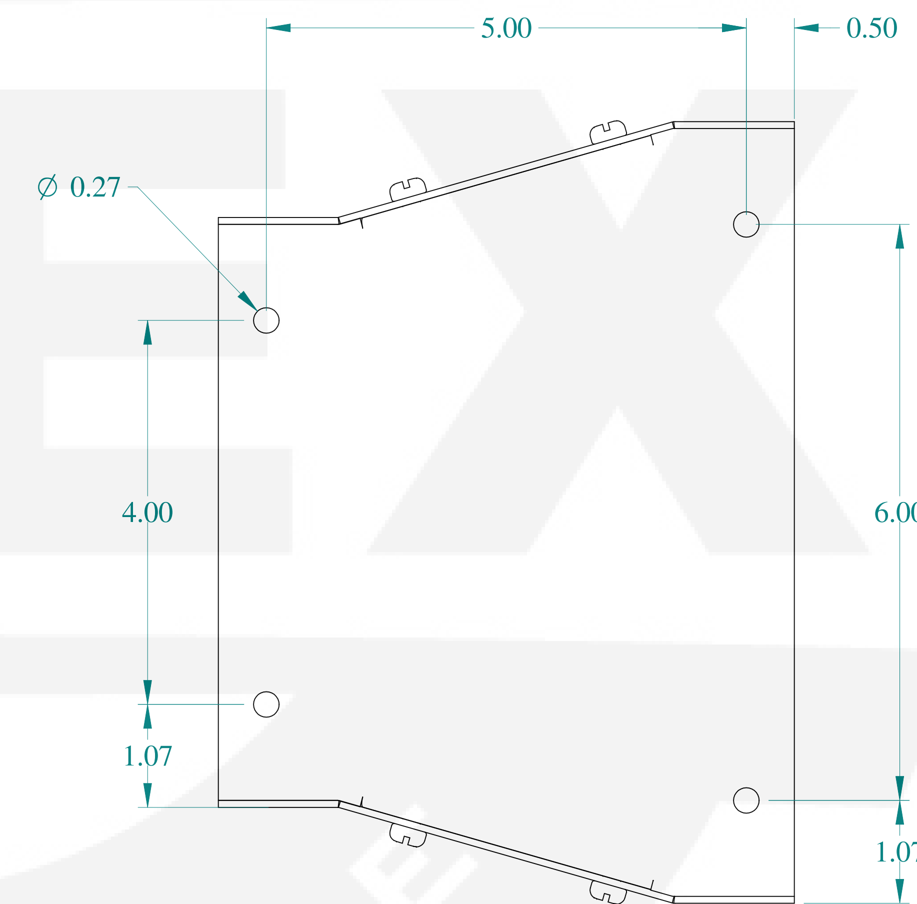
SIDE VIEW
