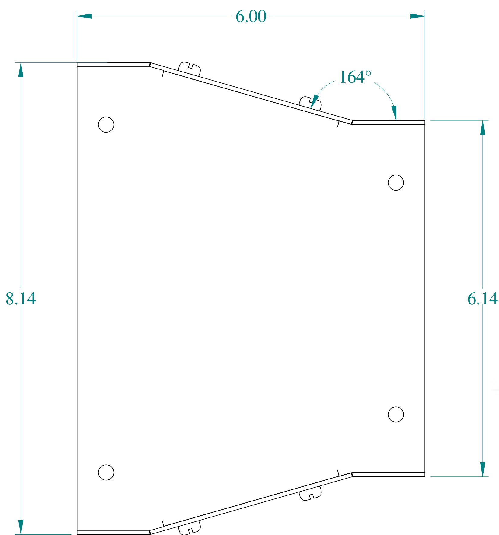
SIDE VIEW
