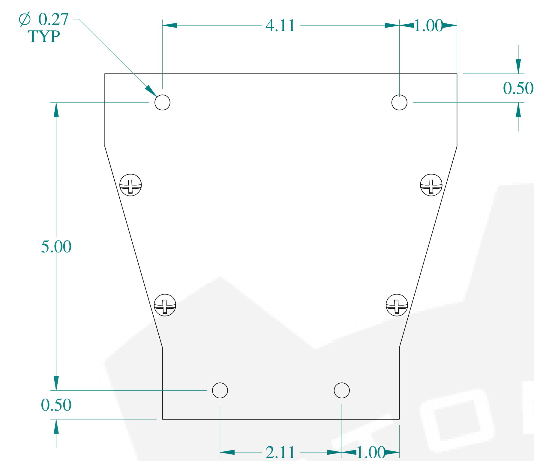
TOP VIEW
