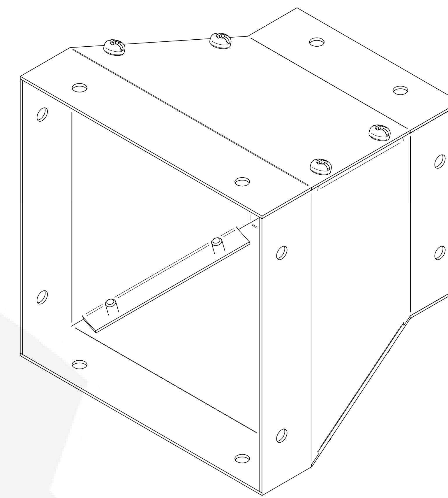
ISOMETRIC VIEWS
