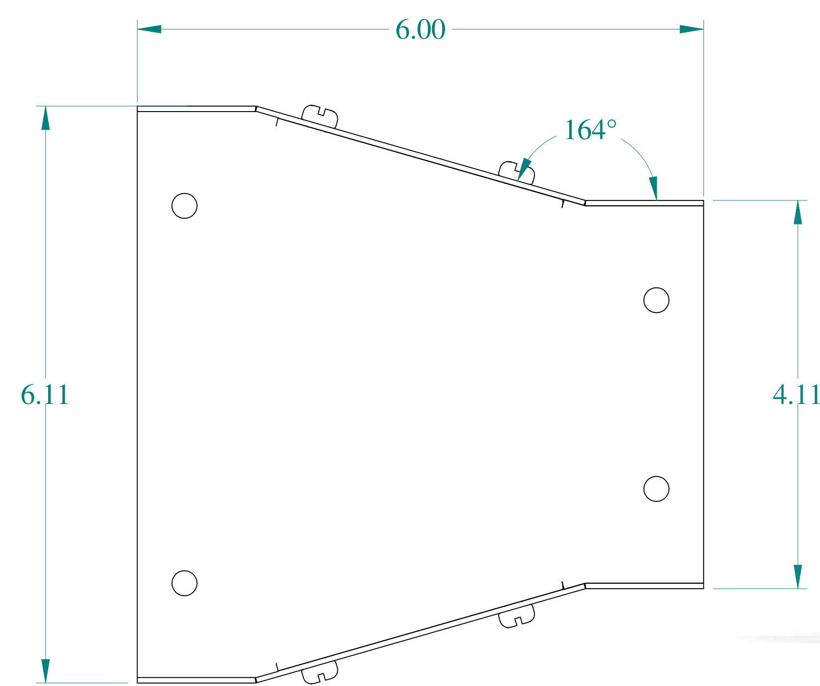
SIDE VIEW
