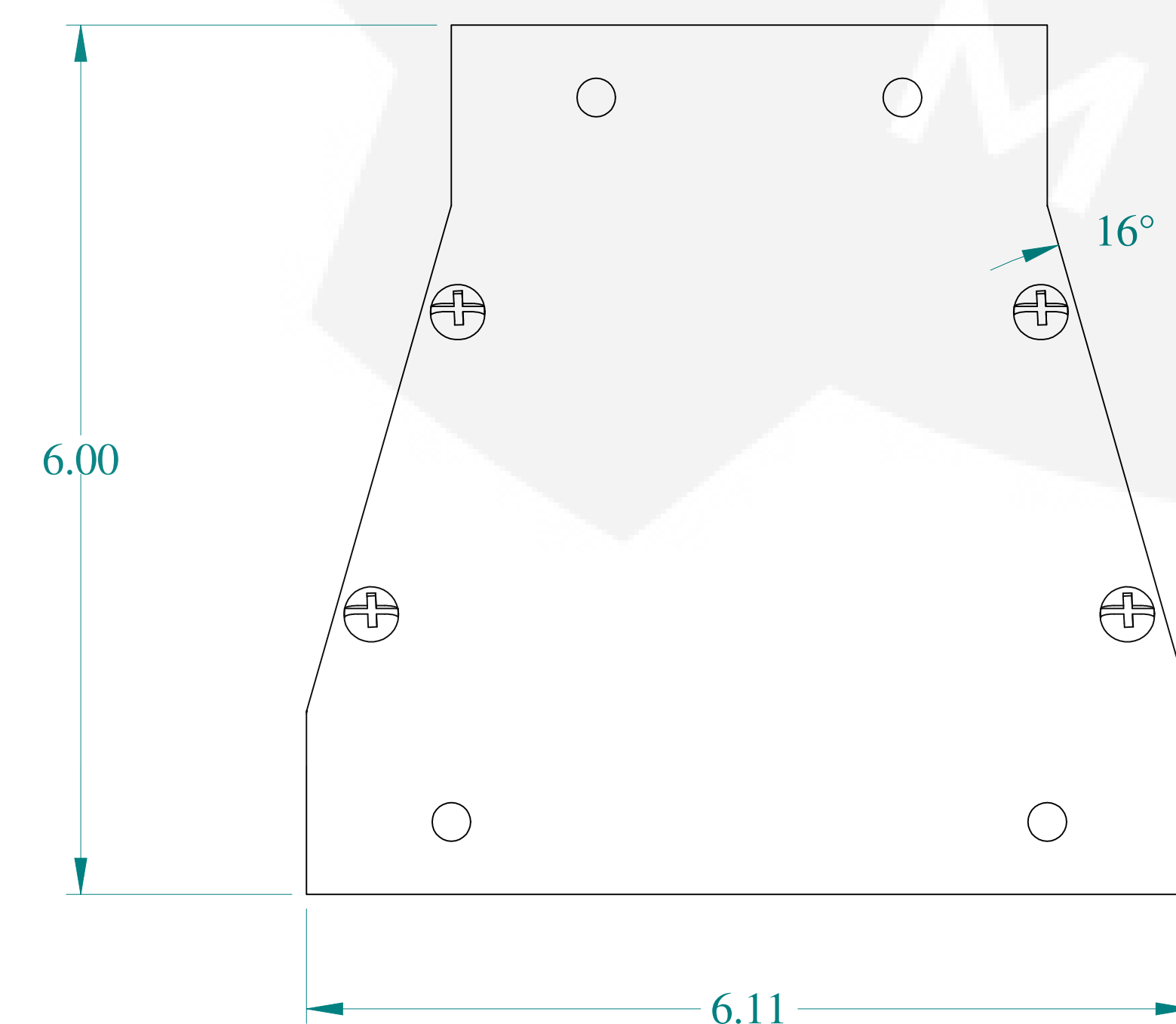
BOTTOM VIEW
