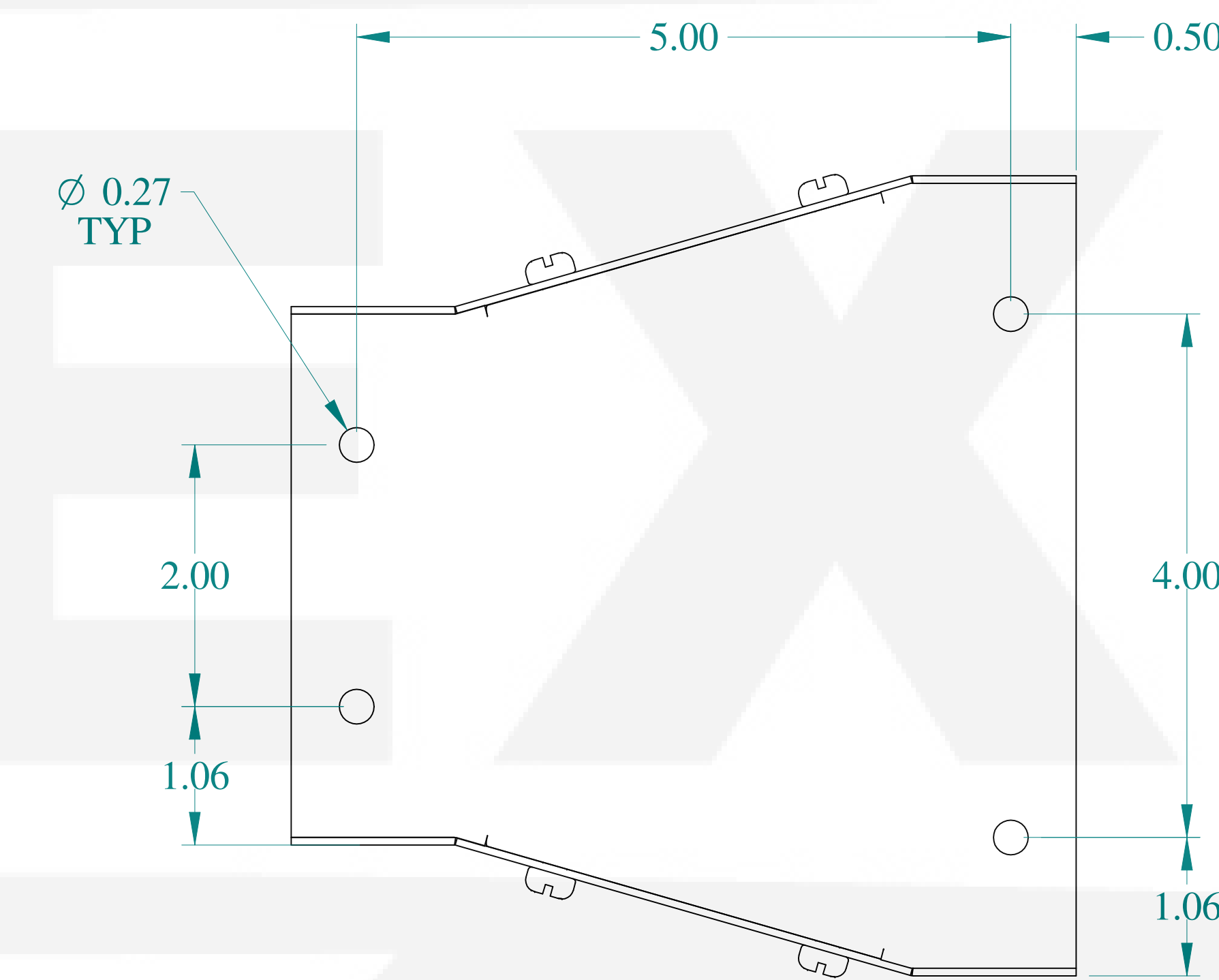
SIDE VIEW
