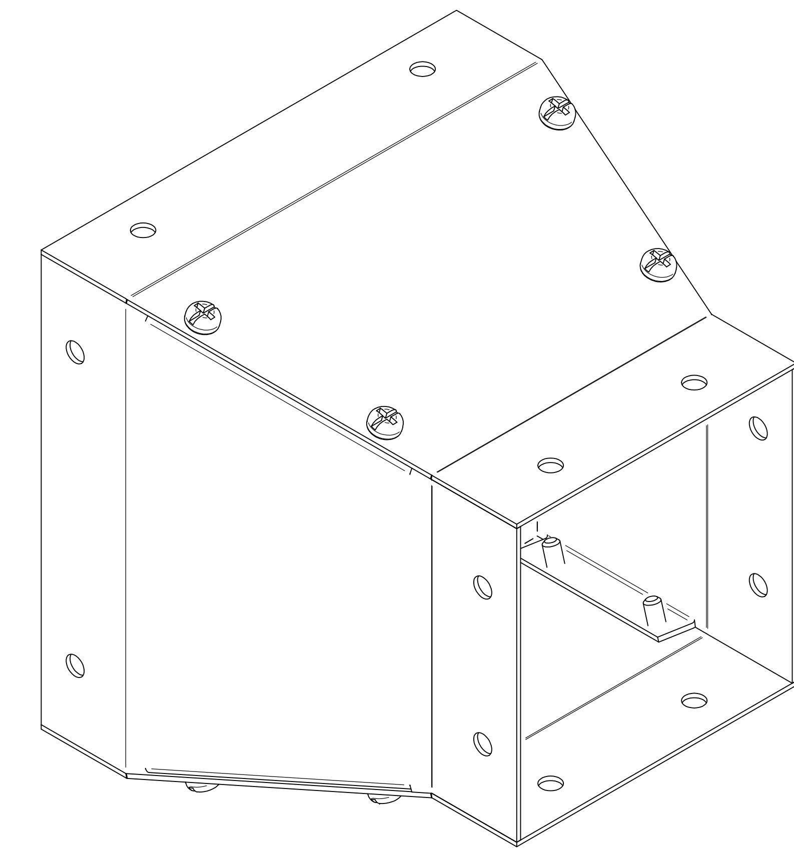
ISOMETRIC VIEWS
