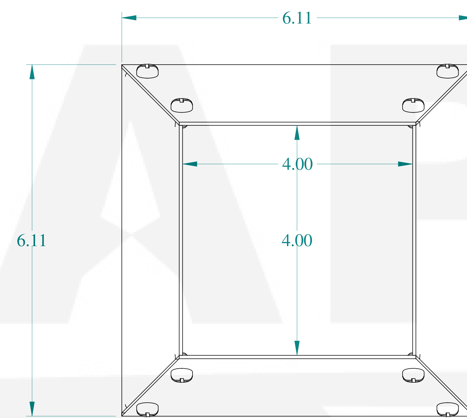
FRONT VIEW
