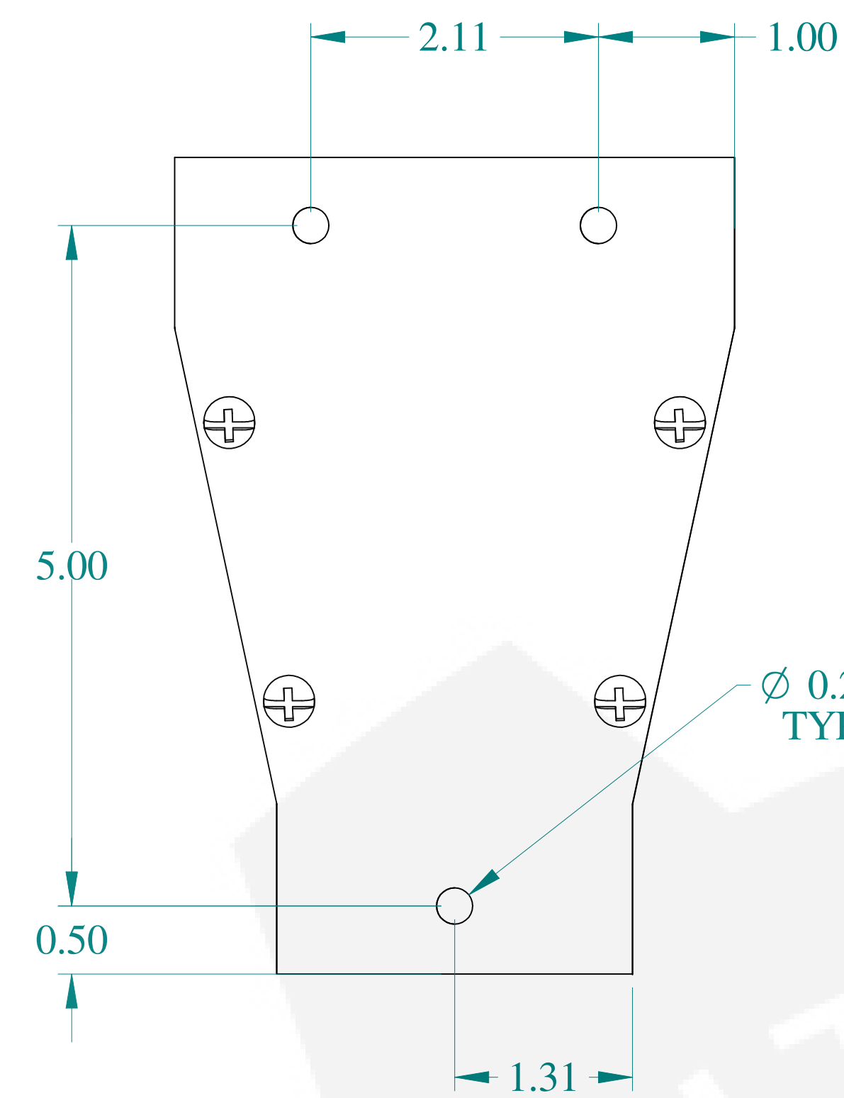
TOP VIEW
