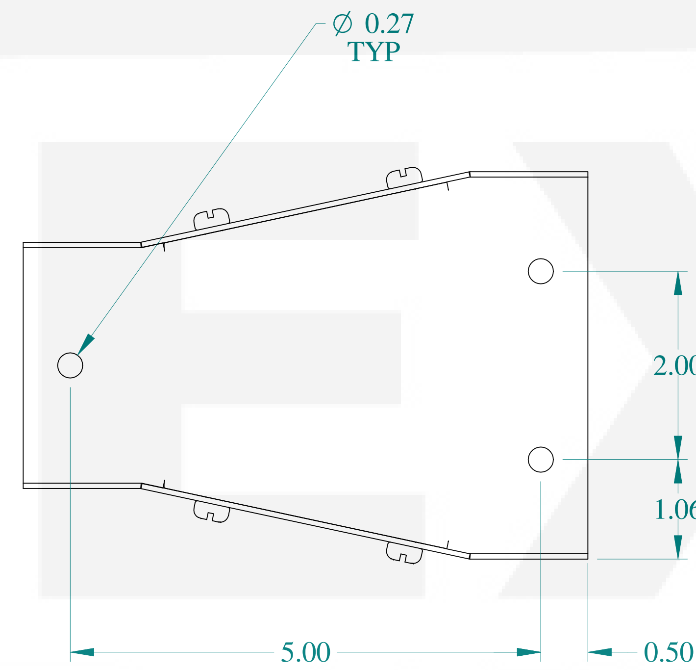
SIDE VIEW
