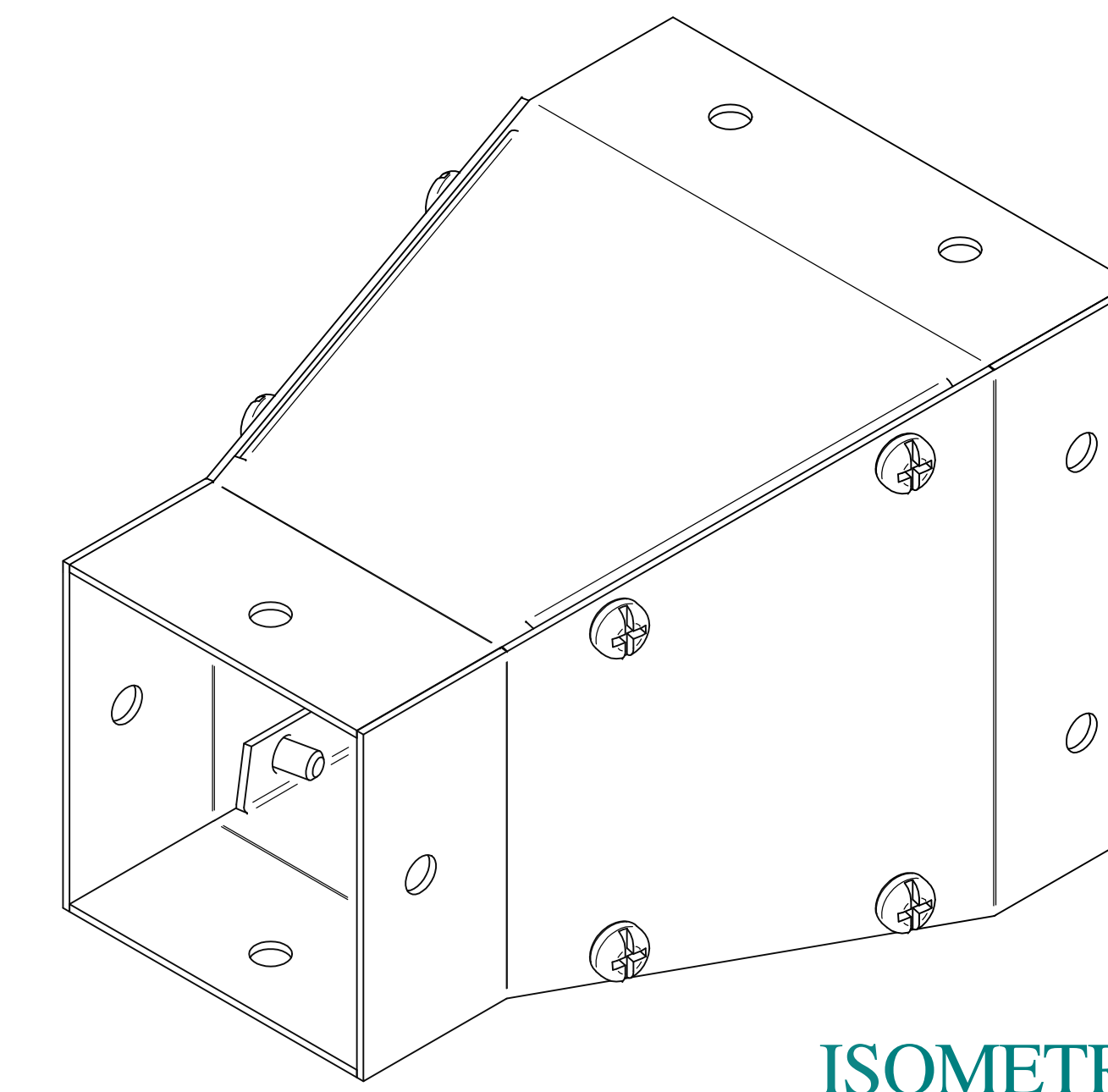
ISOMETRIC VIEWS
