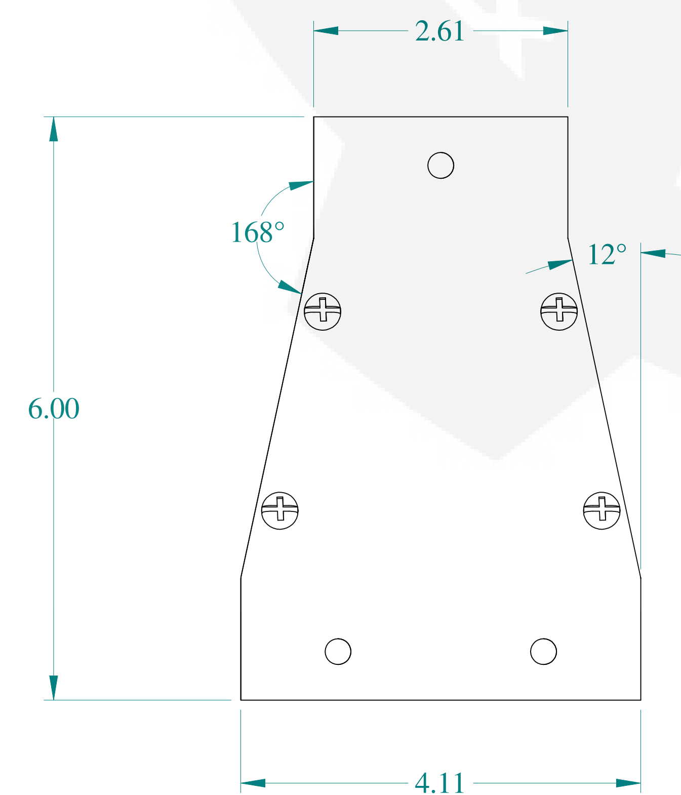
BOTTOM VIEW
