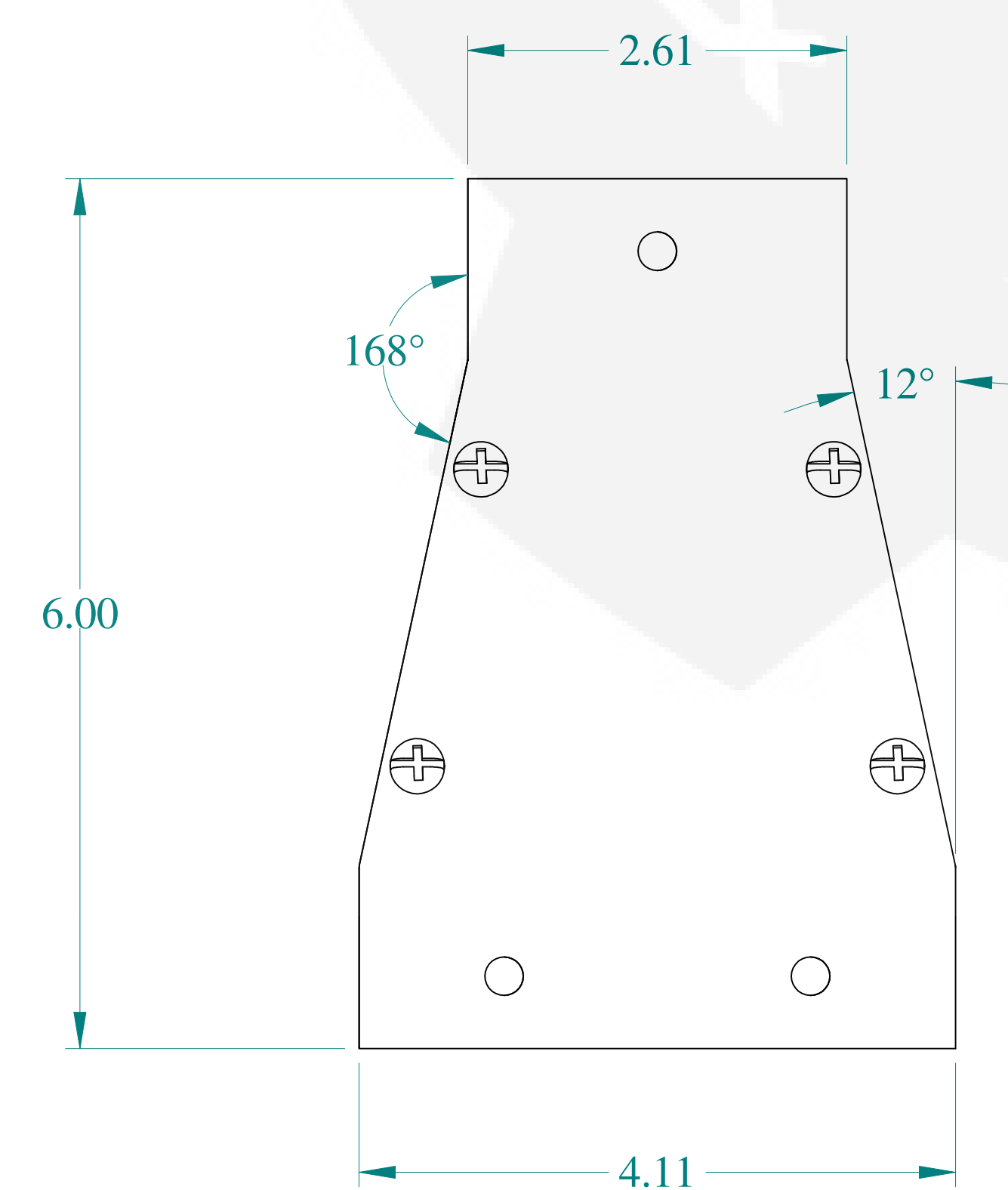
BOTTOM VIEW
