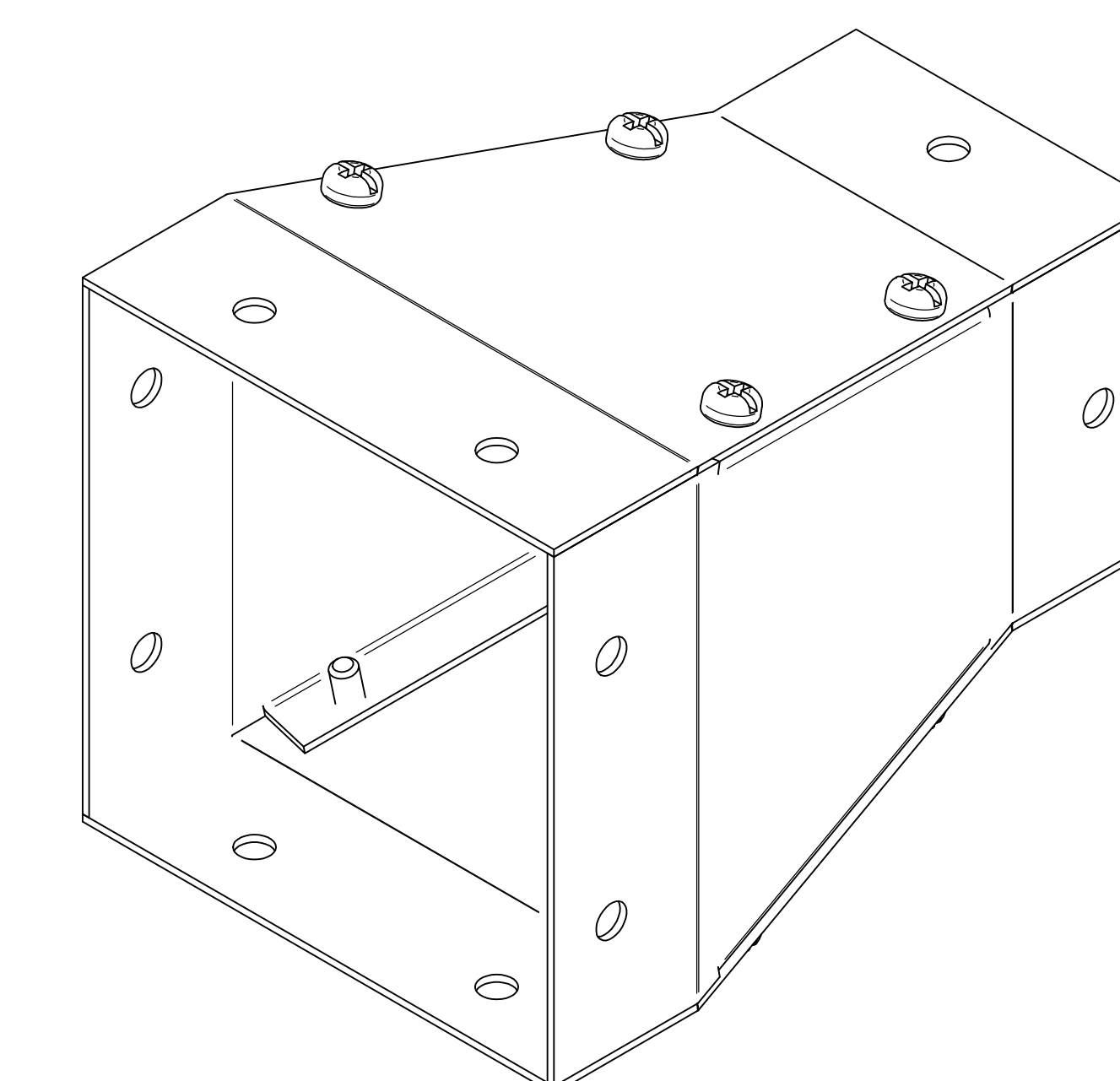
ISOMETRIC VIEWS
