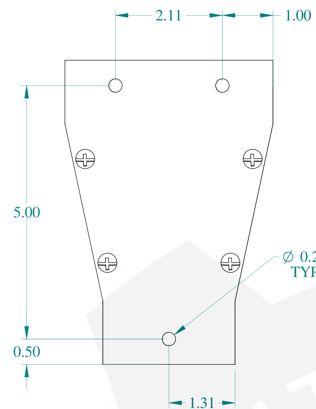
TOP VIEW
