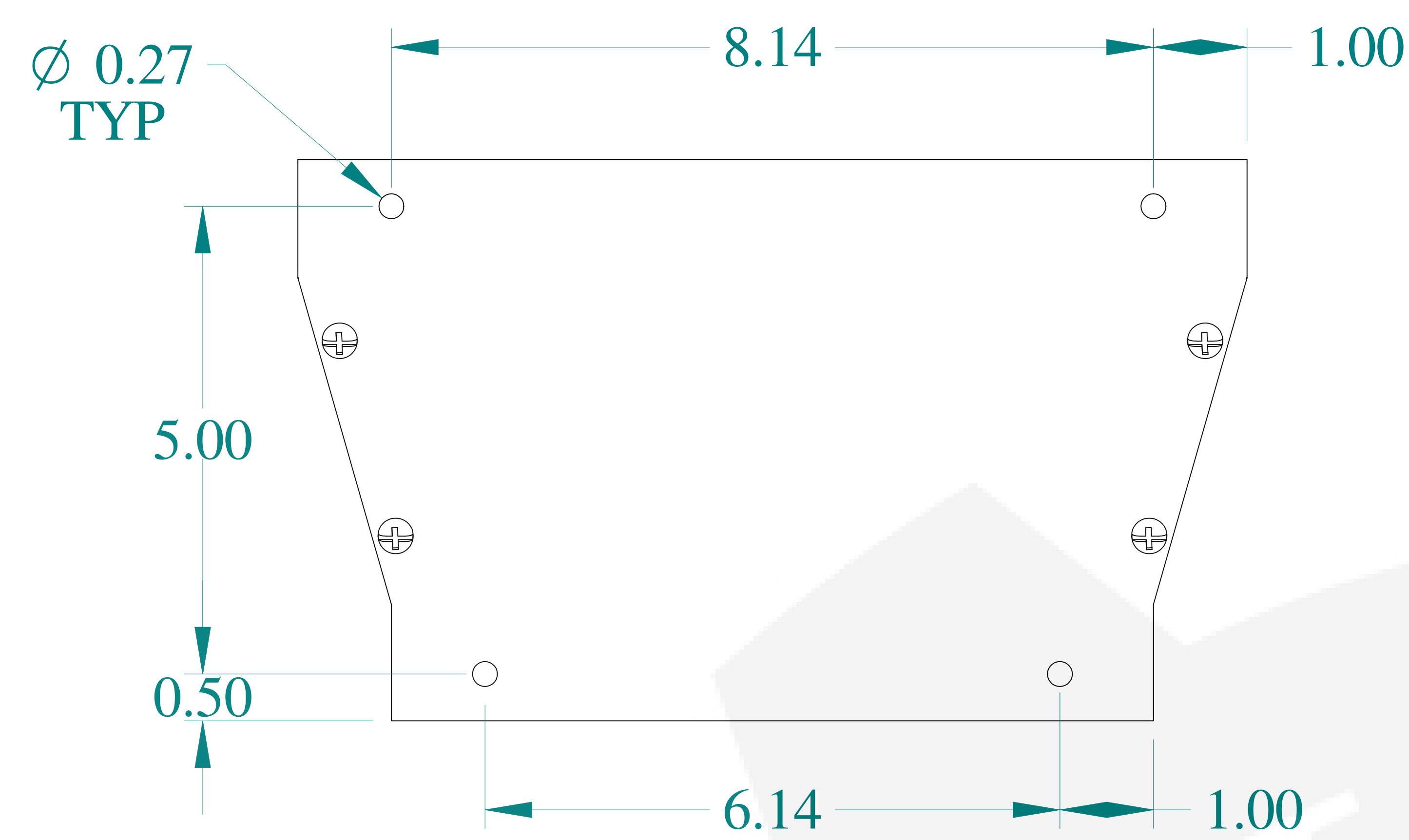
TOP VIEW
