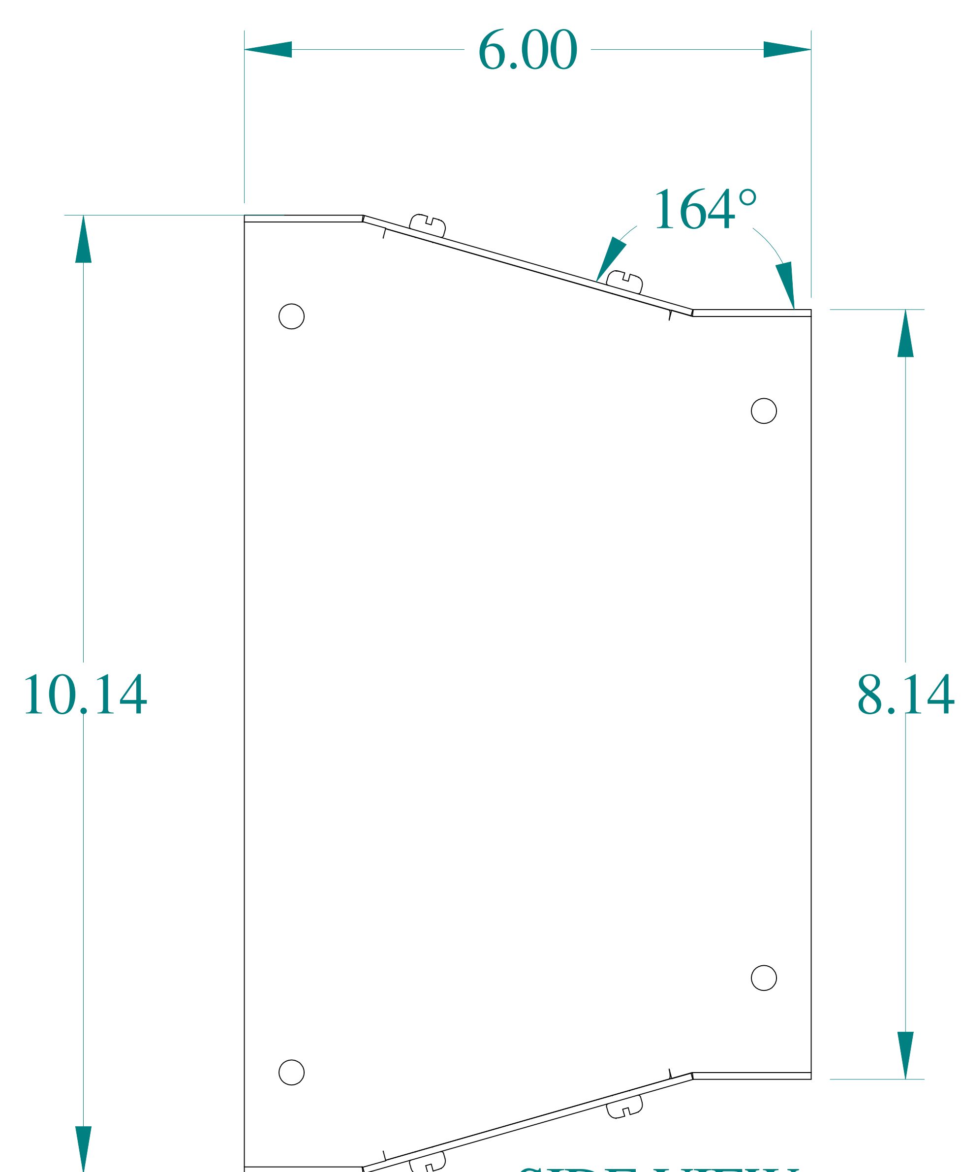
SIDE VIEW
