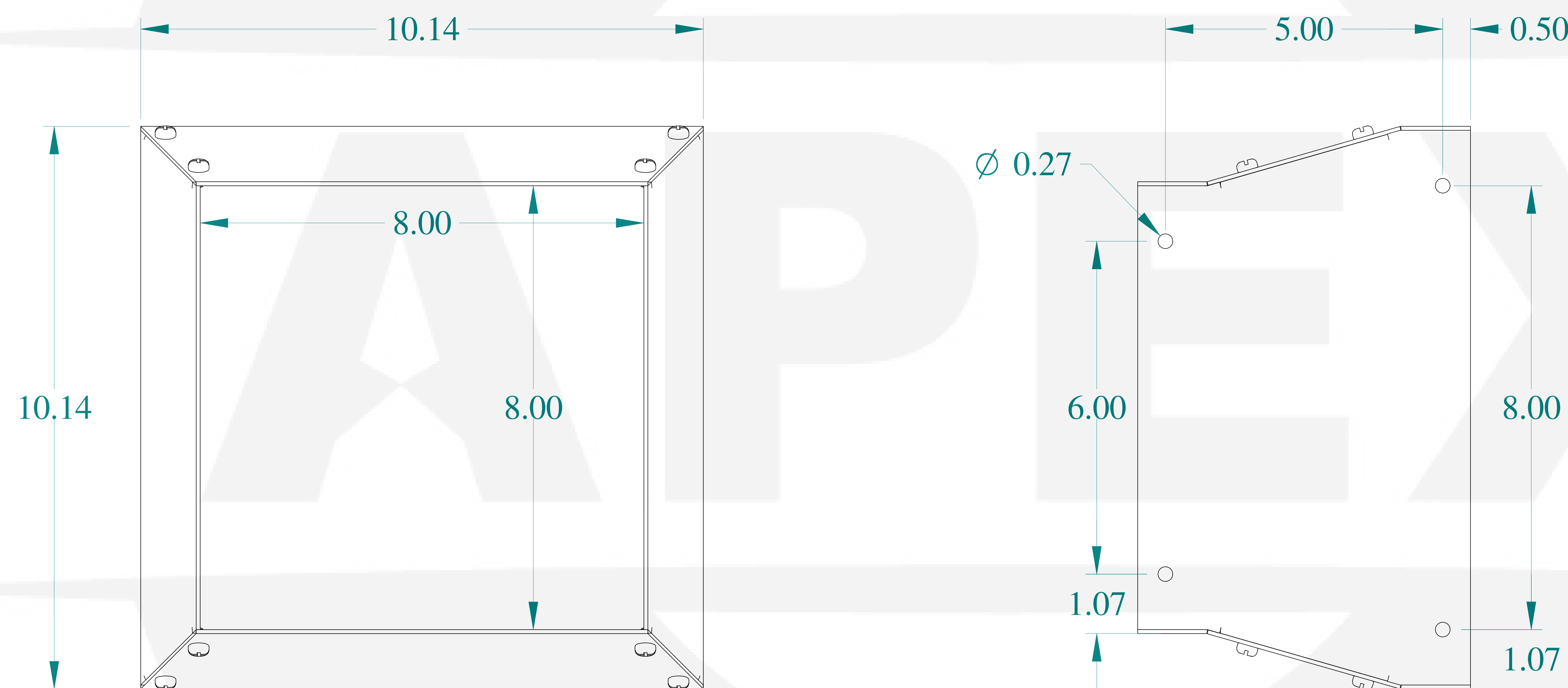
FRONT VIEW
