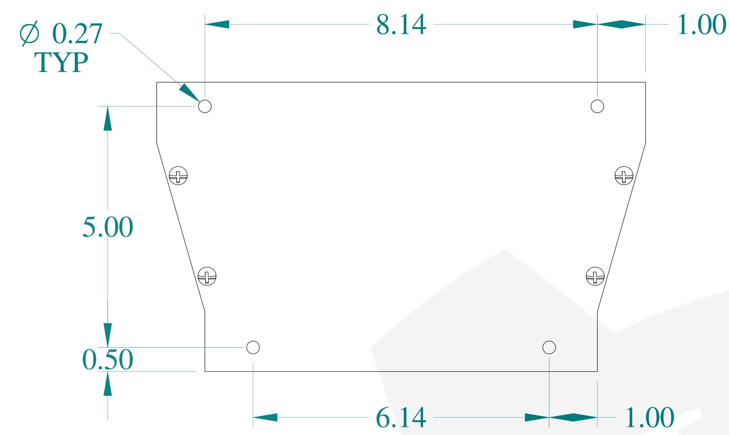
TOP VIEW
