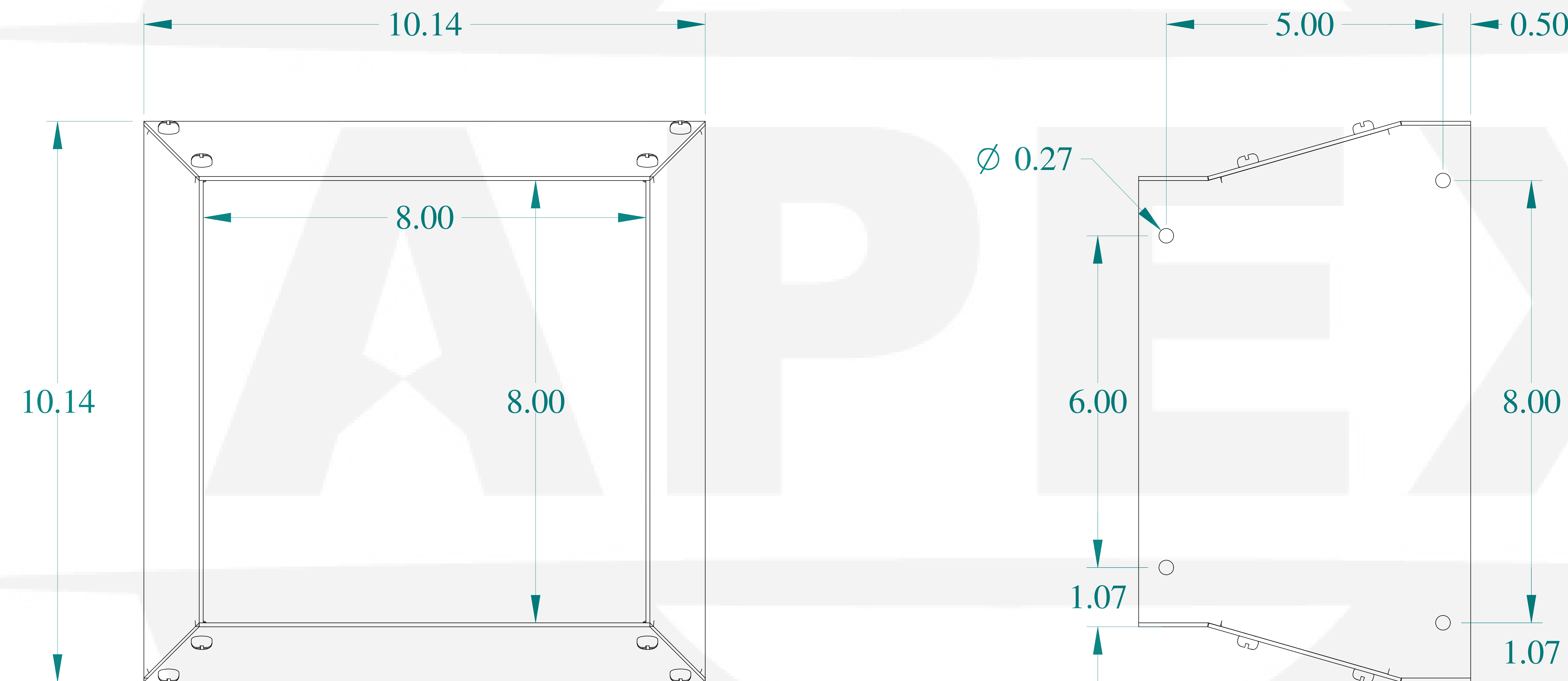
FRONT VIEW
