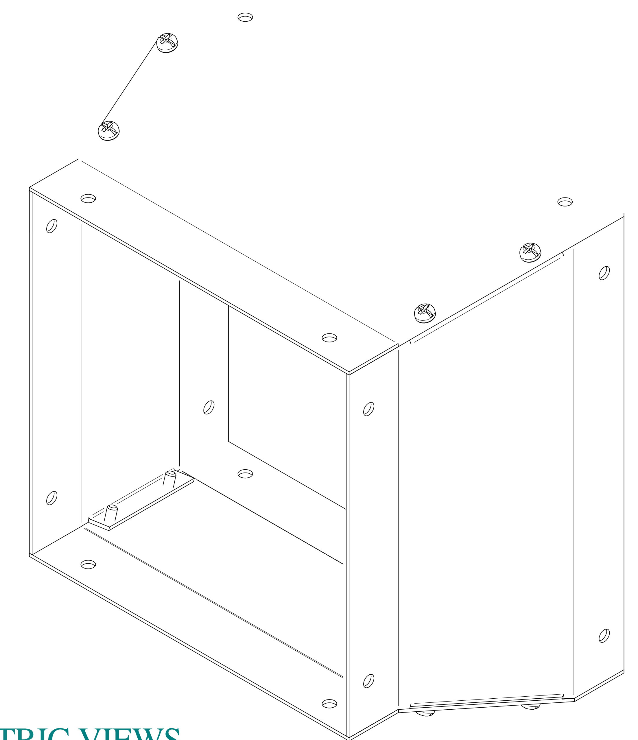
ISOMETRIC VIEWS
