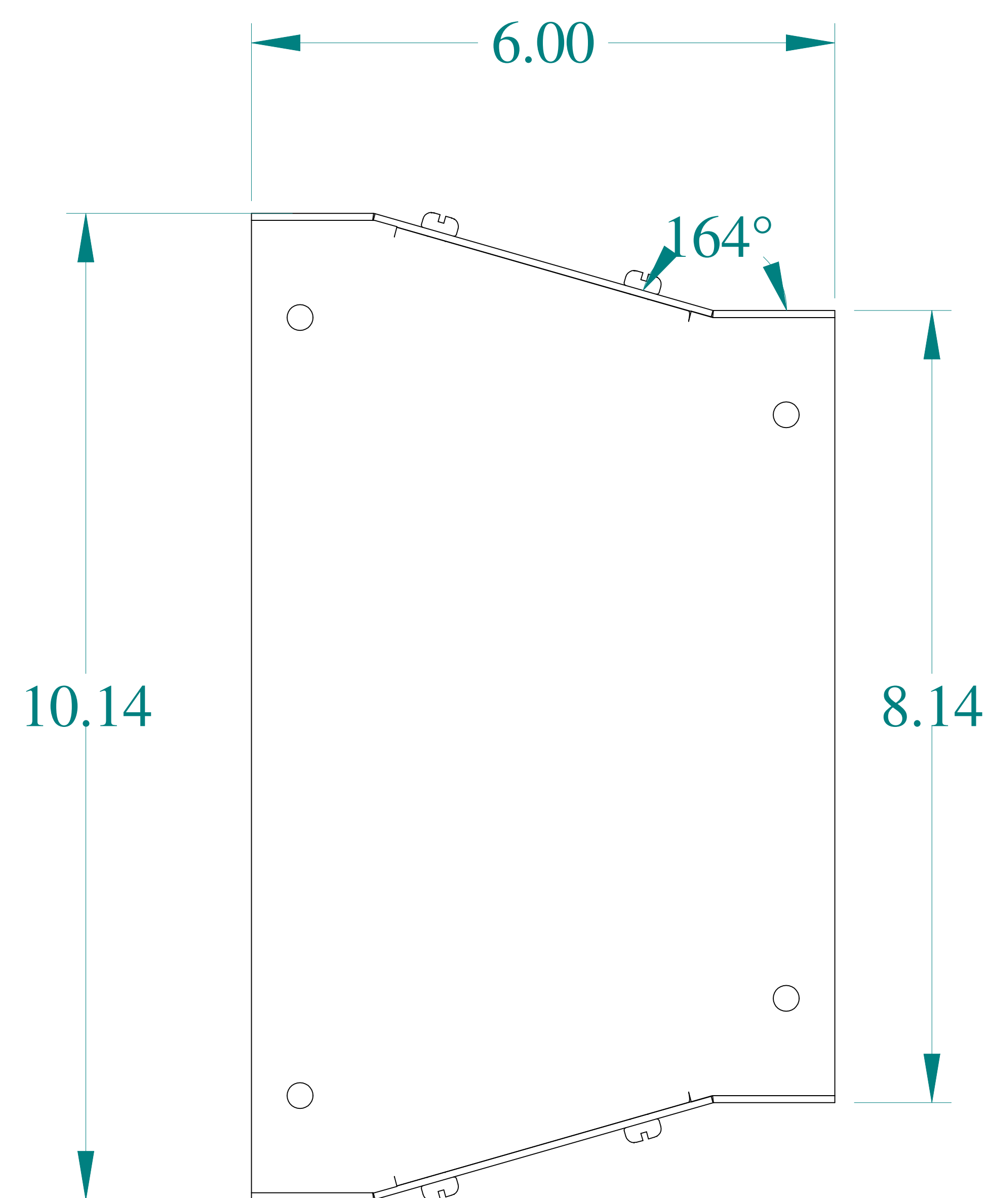
SIDE VIEW
