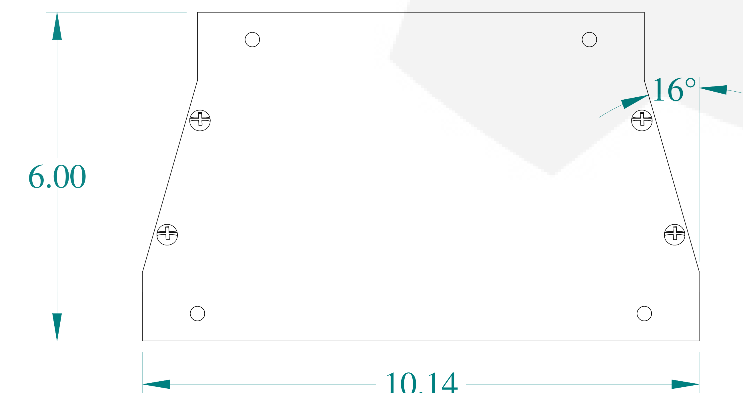
BOTTOM VIEW
