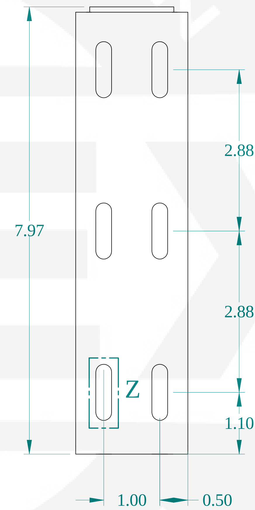
SIDE VIEW
