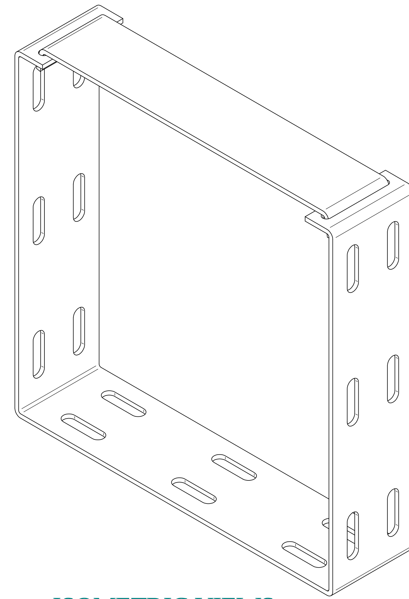
ISOMETRIC VIEWS
