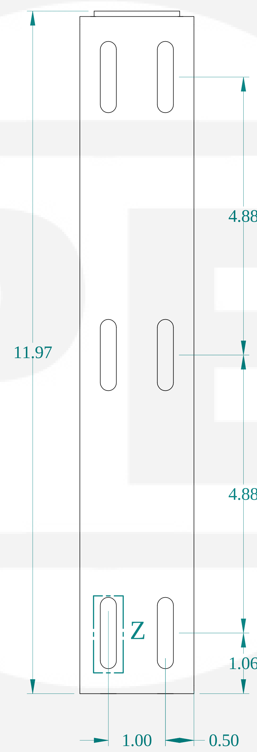
SIDE VIEW
