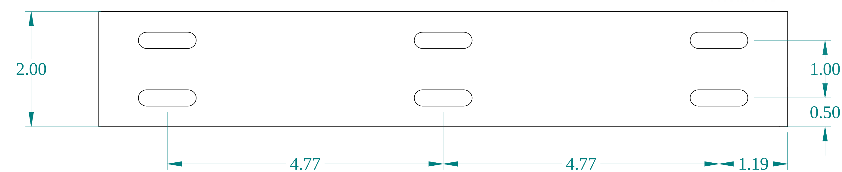
BOTTOM VIEW
