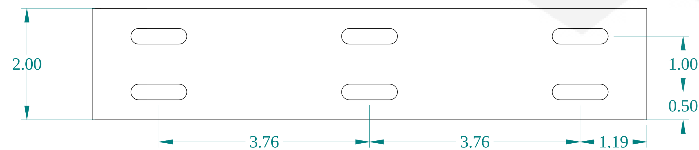
BOTTOM VIEW
