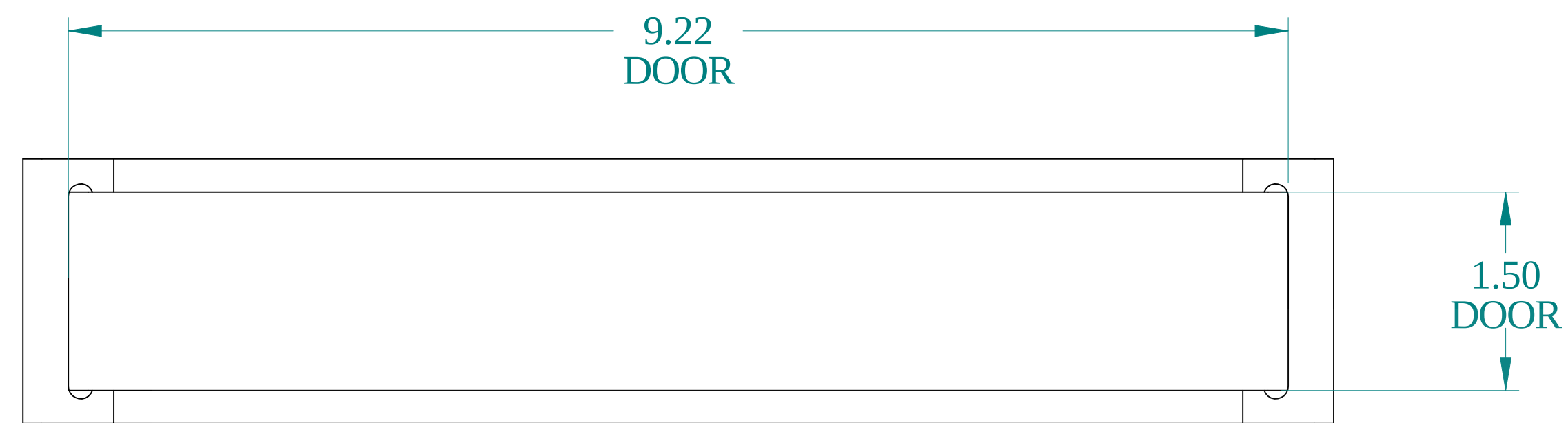
TOP VIEW
