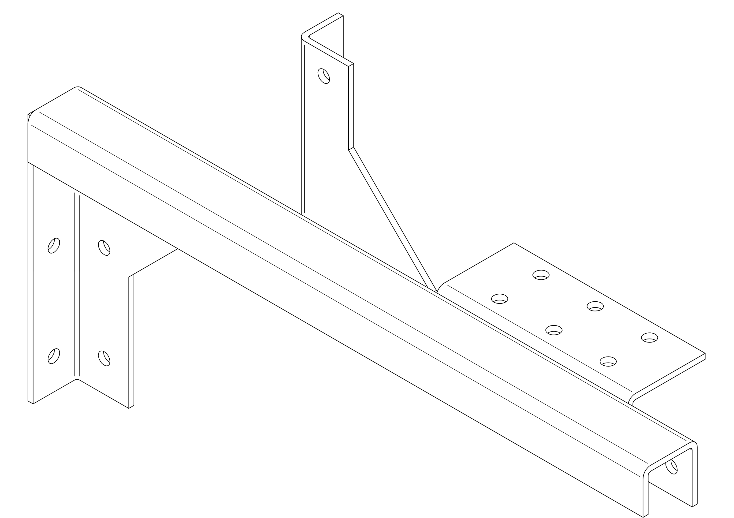
ISOMETRIC VIEWS
