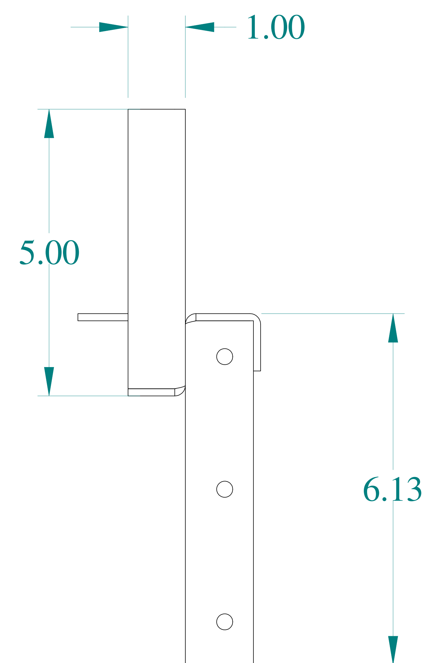
SIDE VIEW
