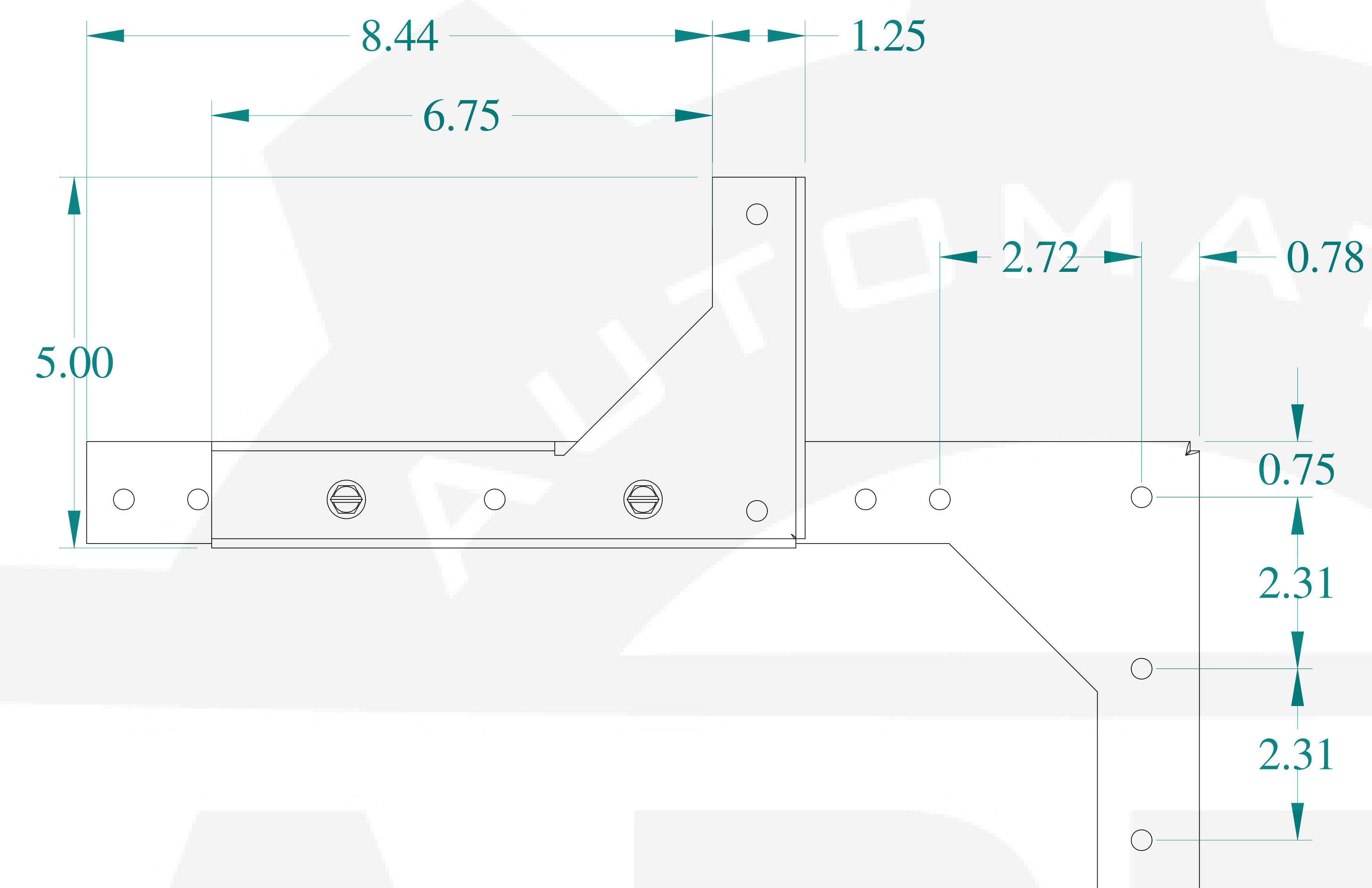
BACK VIEW
