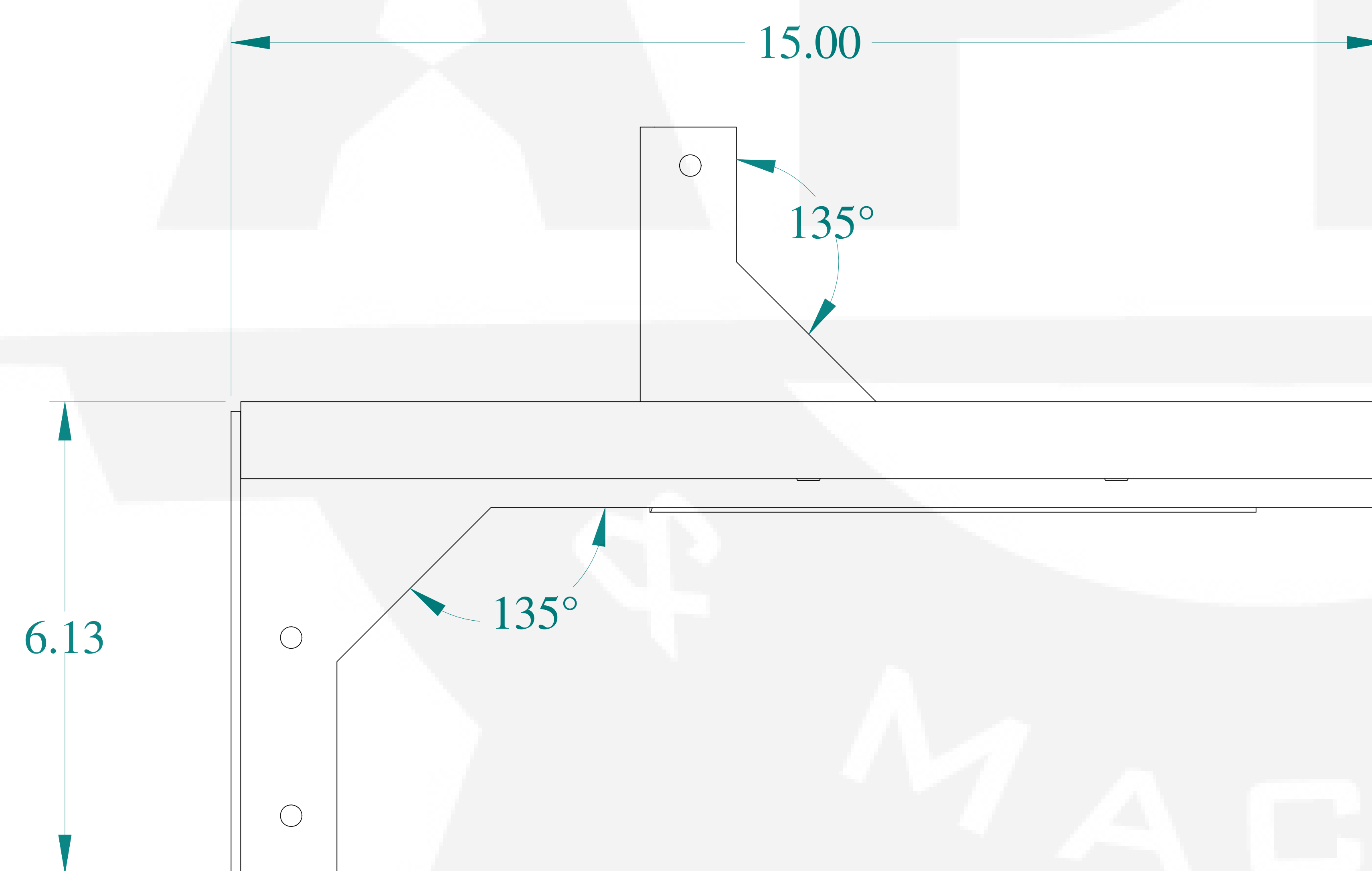
FRONT VIEW
