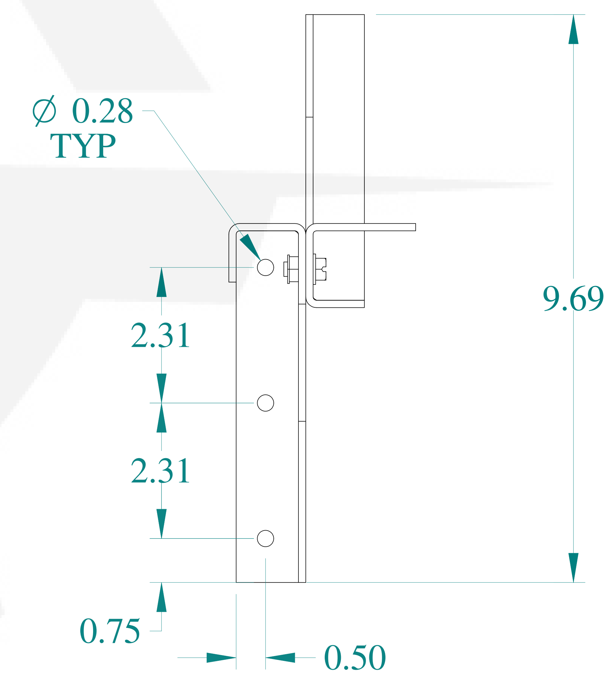
SIDE VIEW
