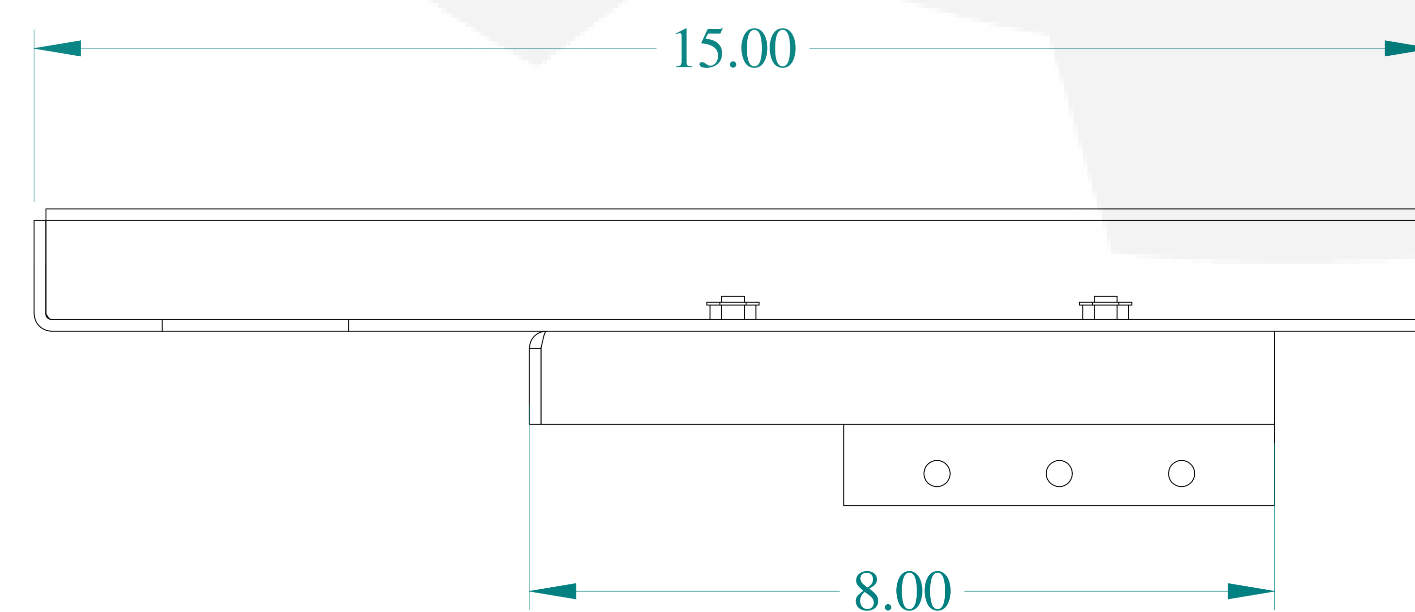
BOTTOM VIEW
