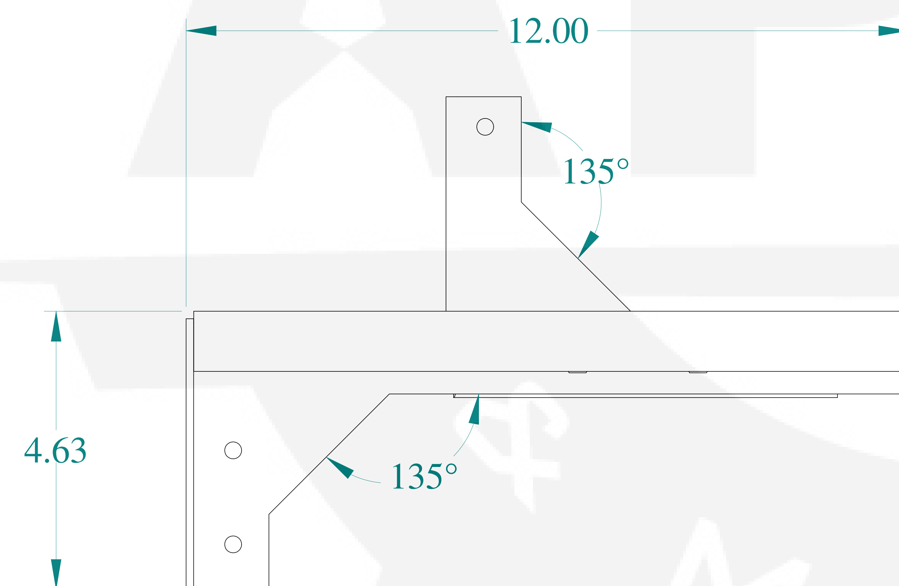
FRONT VIEW
