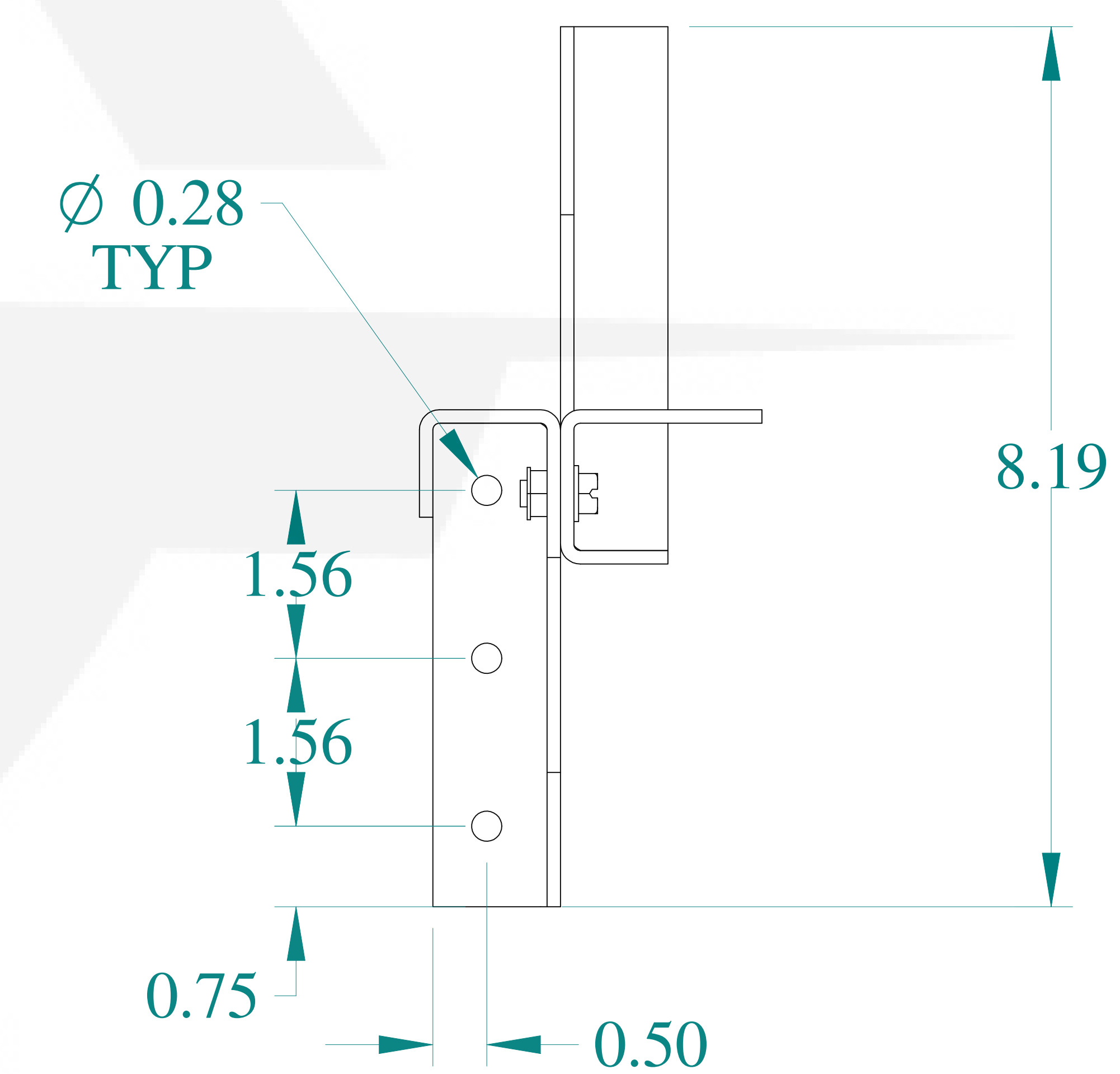
SIDE VIEW
