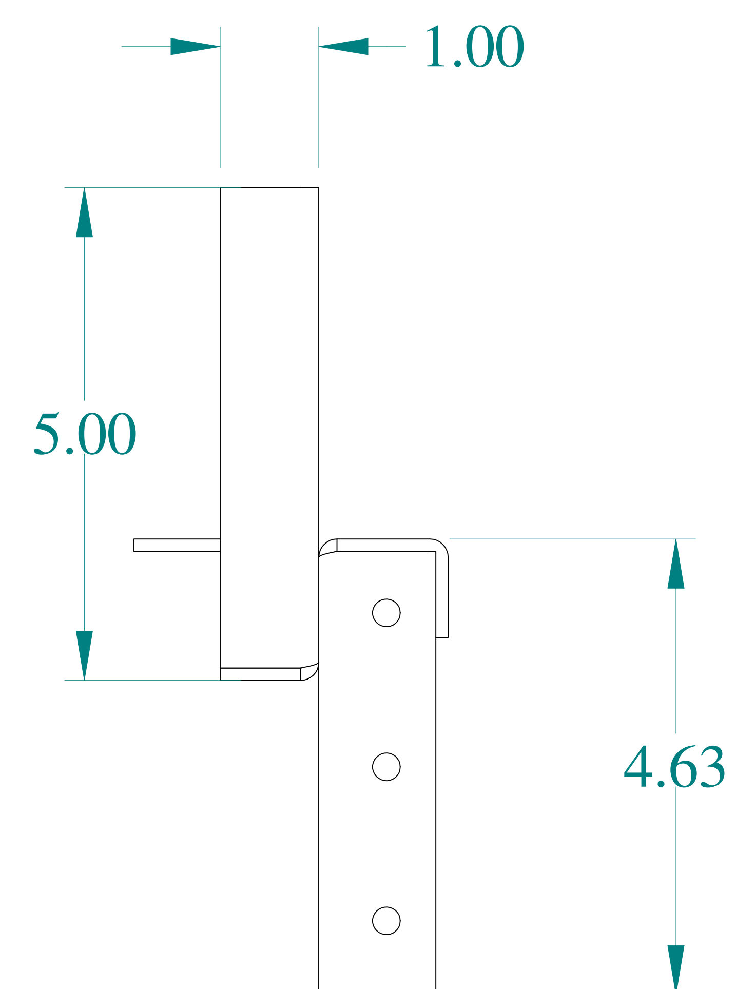
SIDE VIEW
