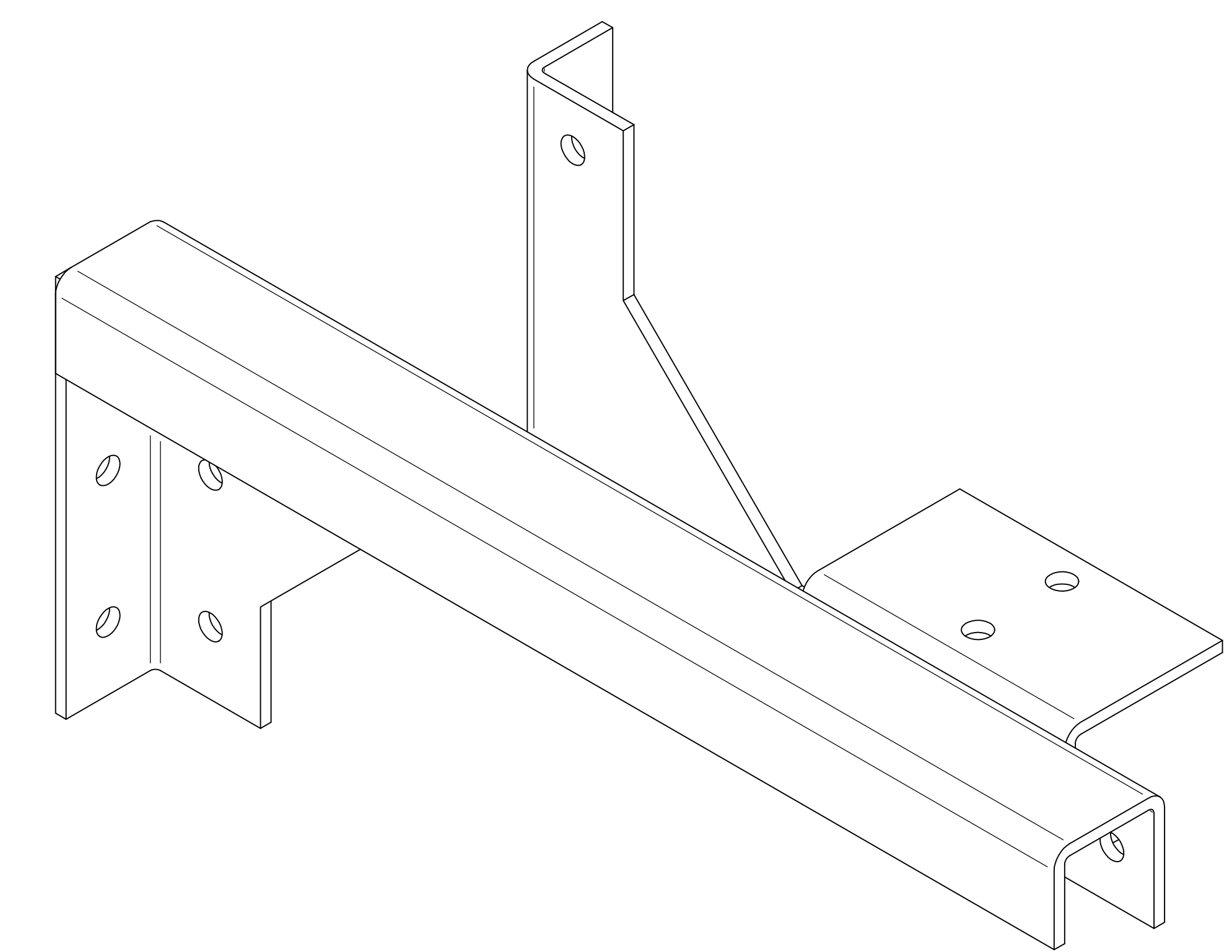
ISOMETRIC VIEWS
