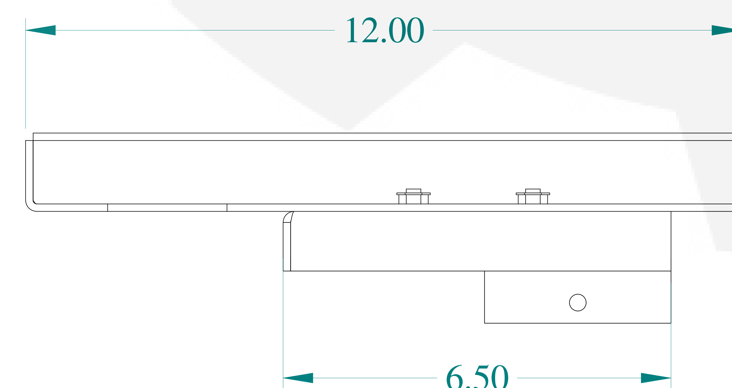
BOTTOM VIEW
