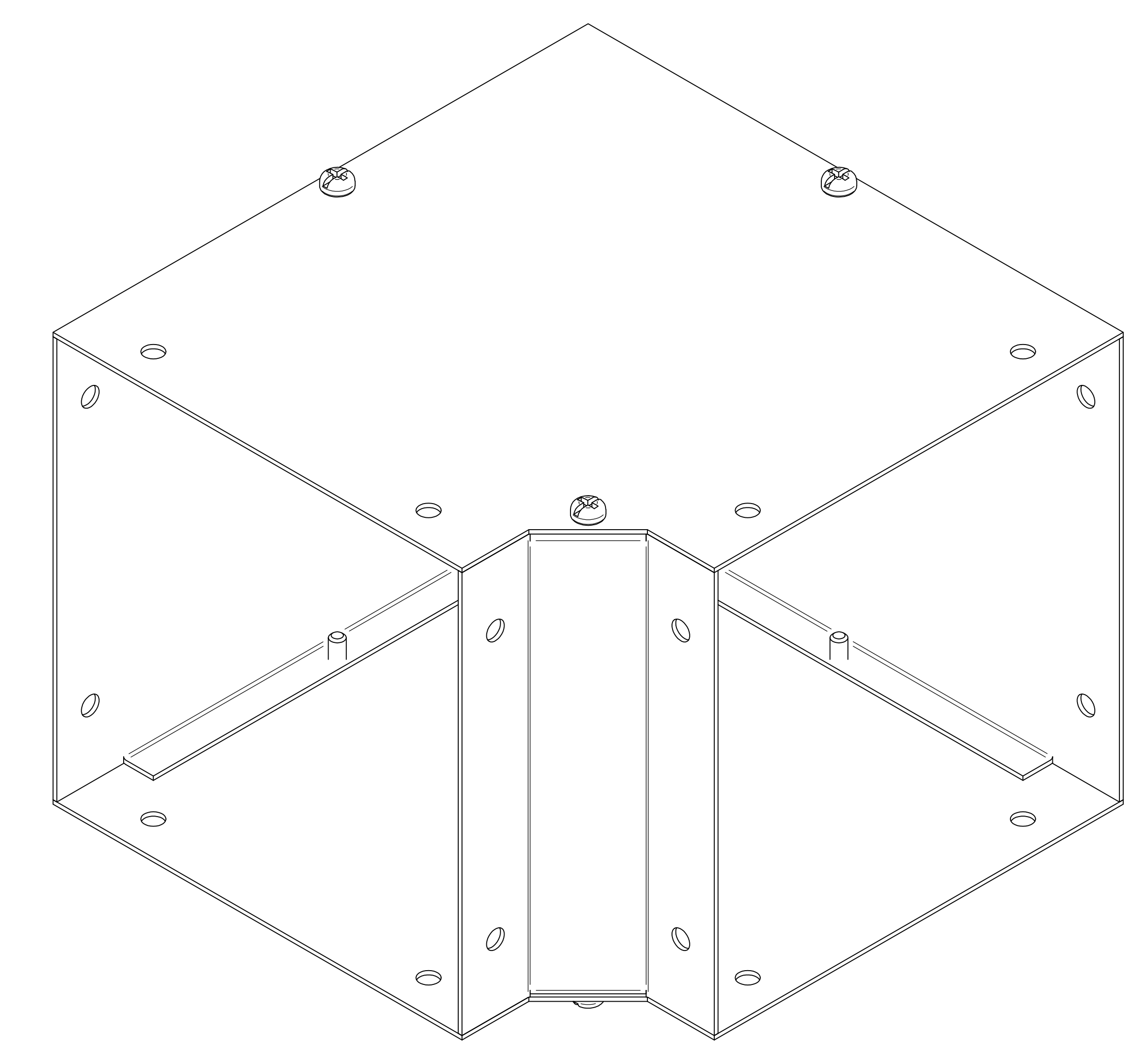
ISOMETRIC VIEWS
