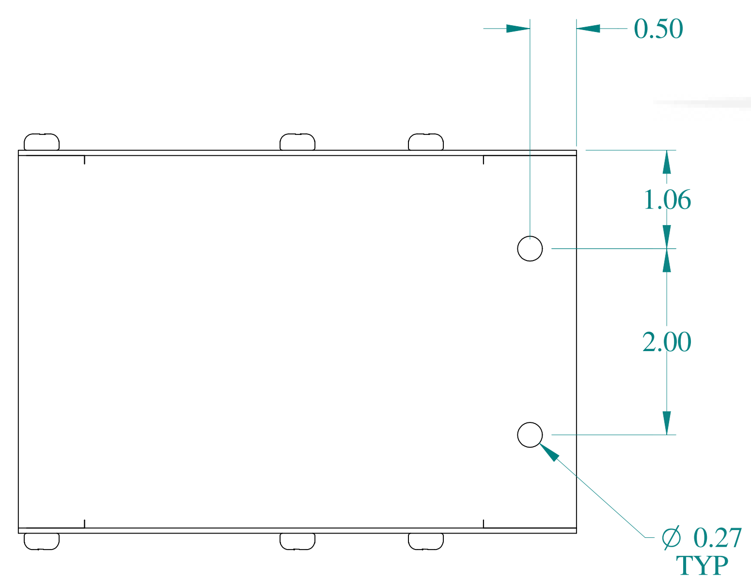
SIDE VIEW
