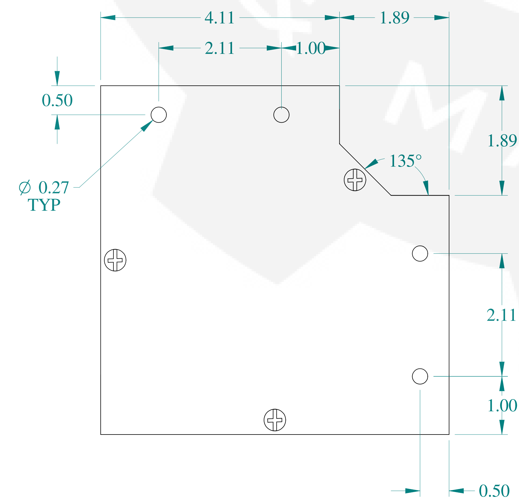
BOTTOM VIEW
