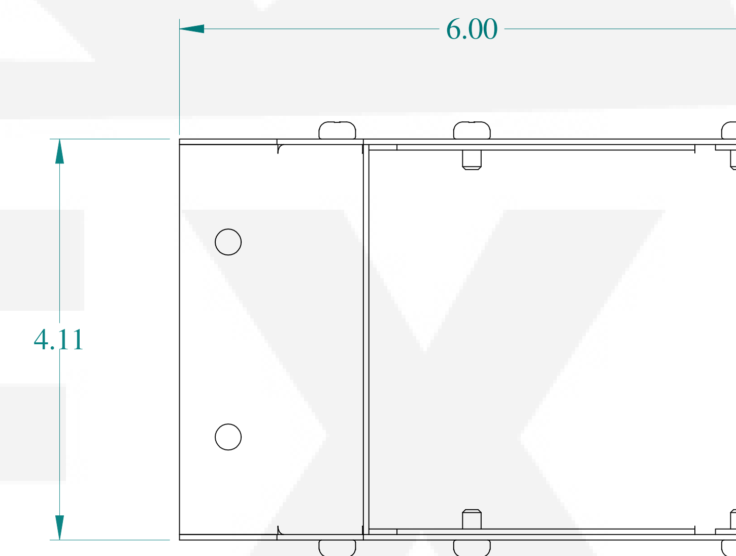
SIDE VIEW
