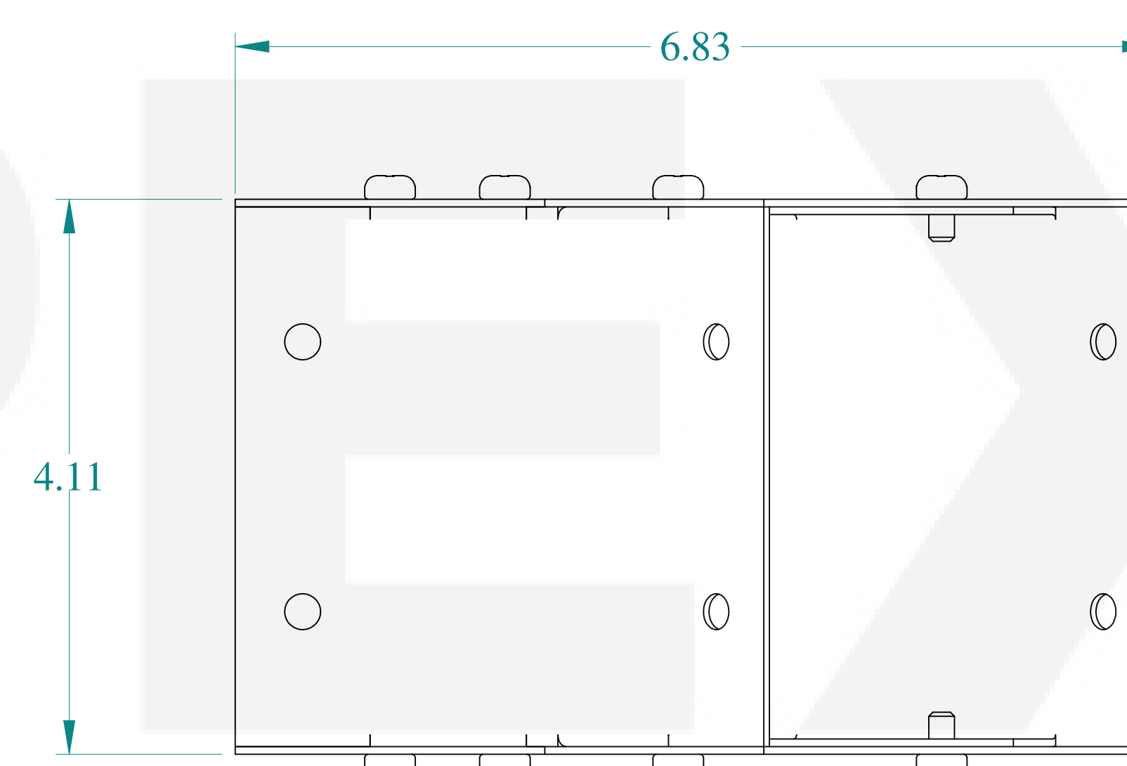
SIDE VIEW
