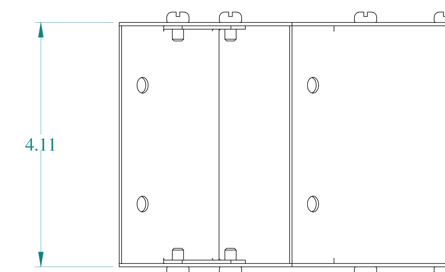
BACK VIEW
