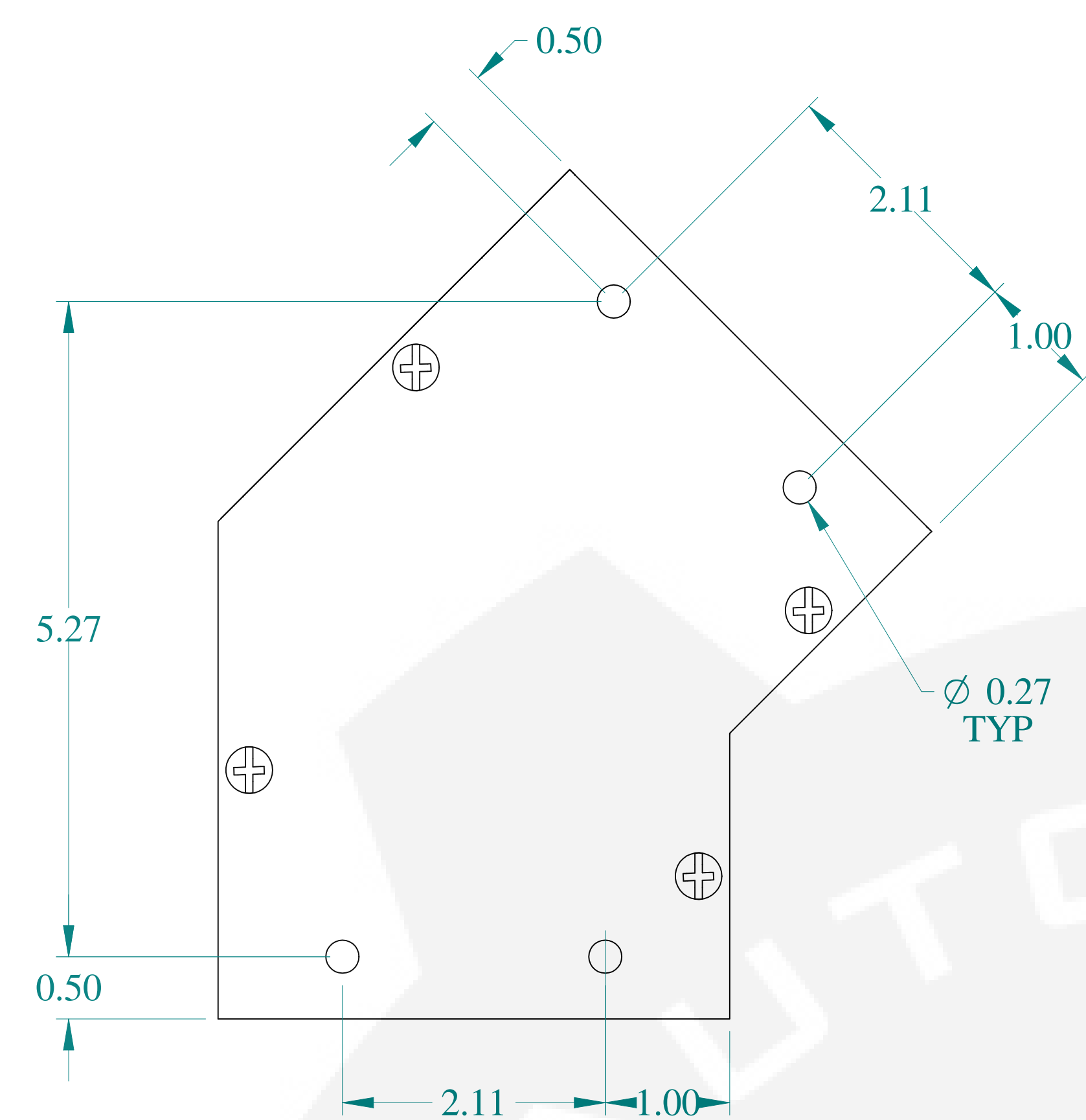
TOP VIEW
