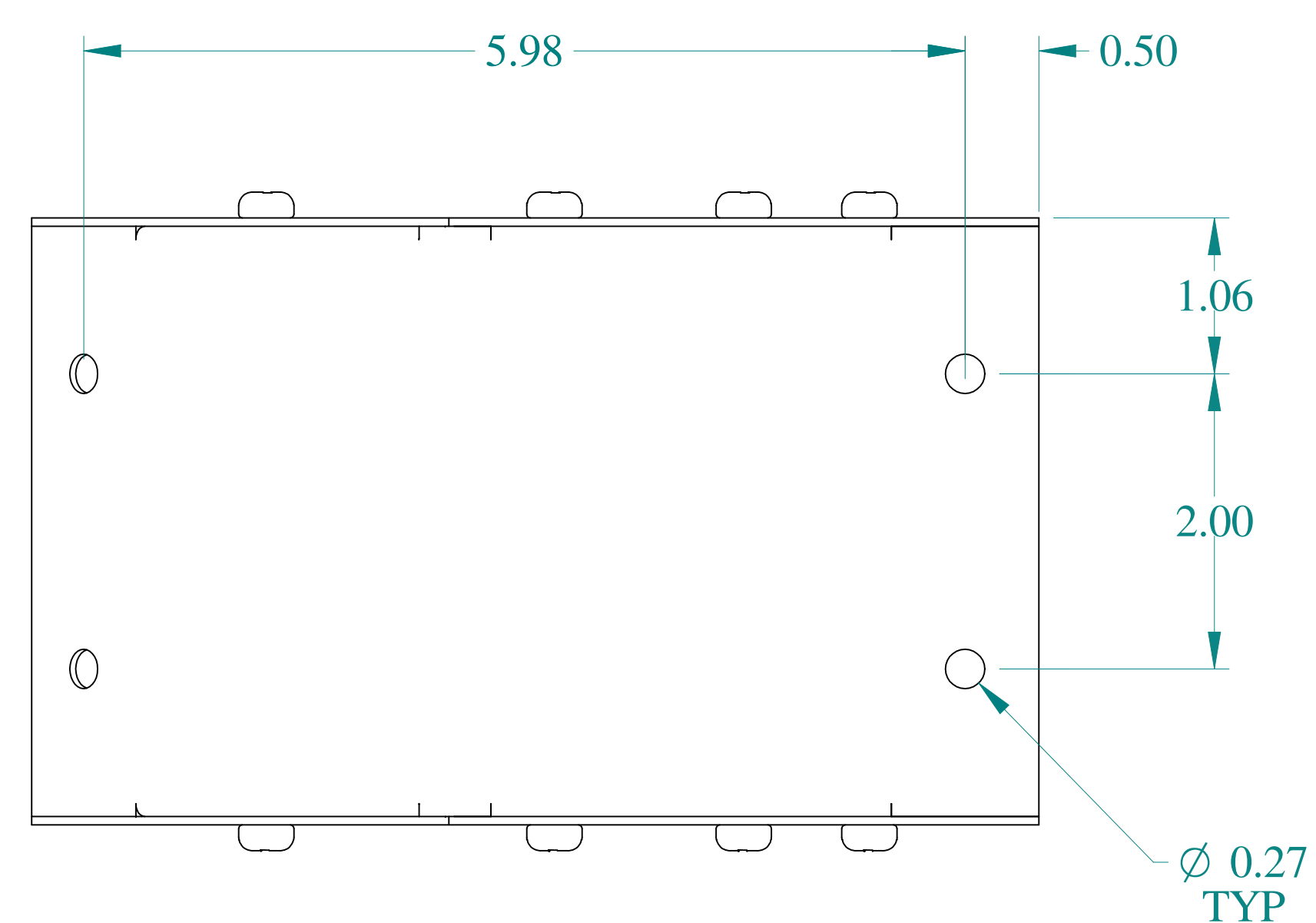
SIDE VIEW
