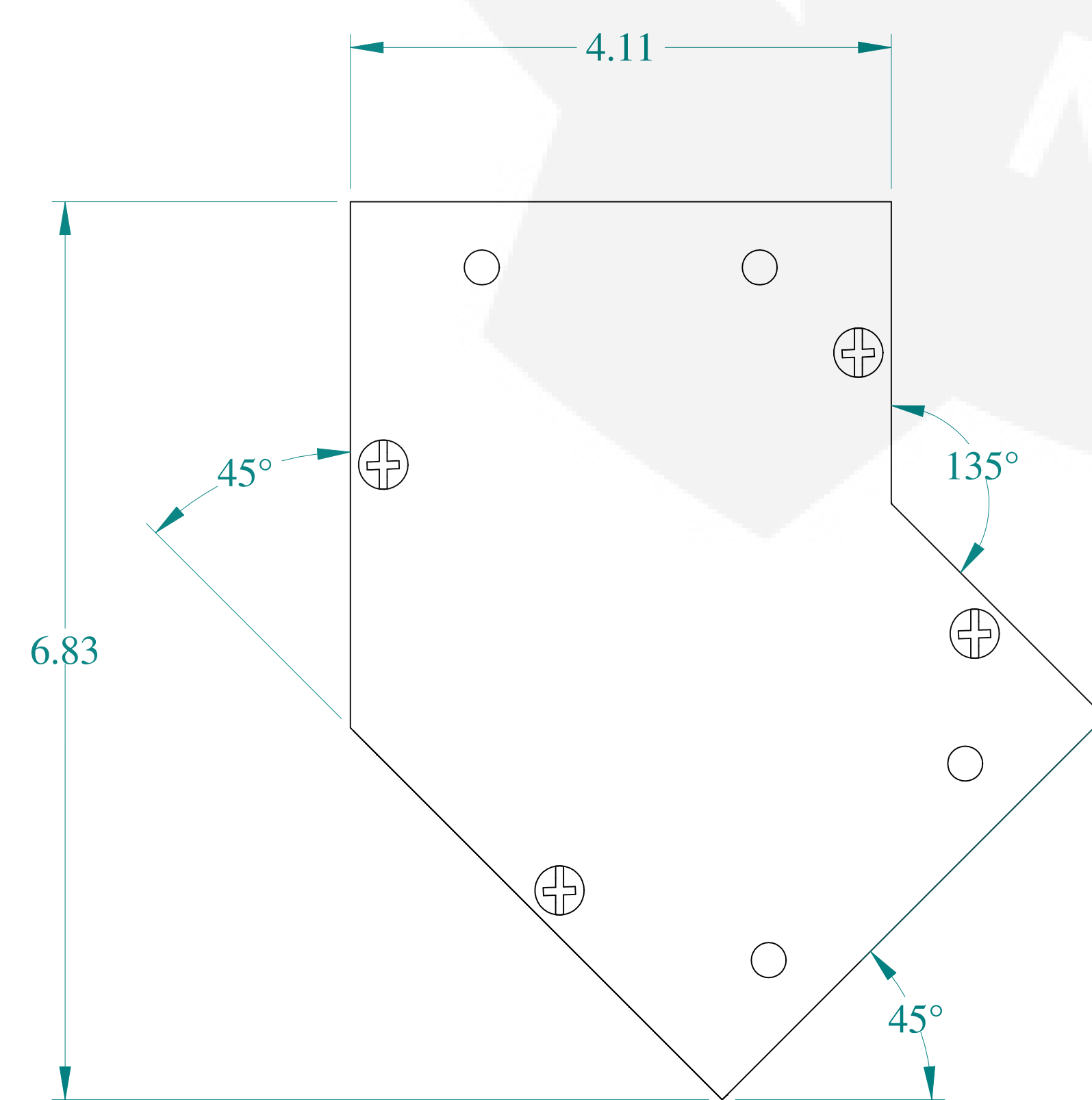
BOTTOM VIEW
