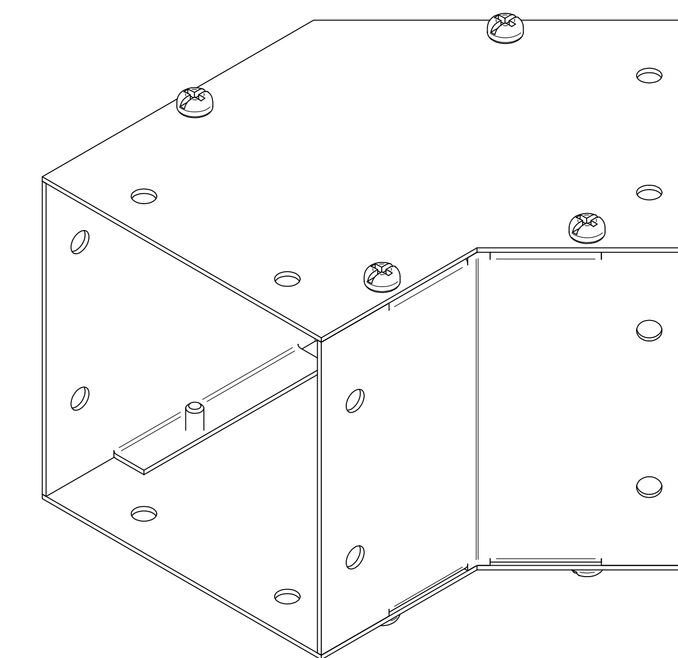
ISOMETRIC VIEWS
