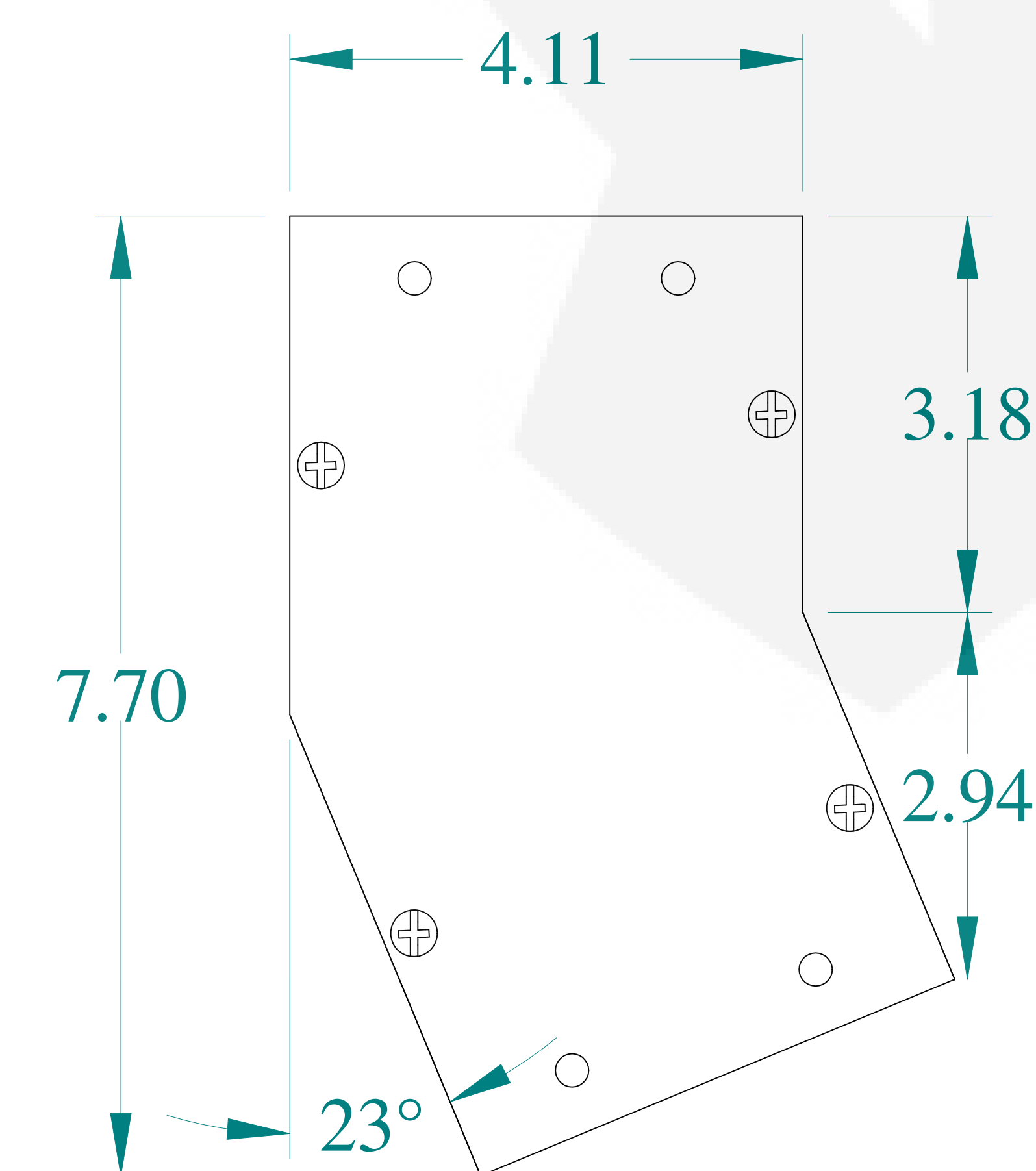
BOTTOM VIEW
