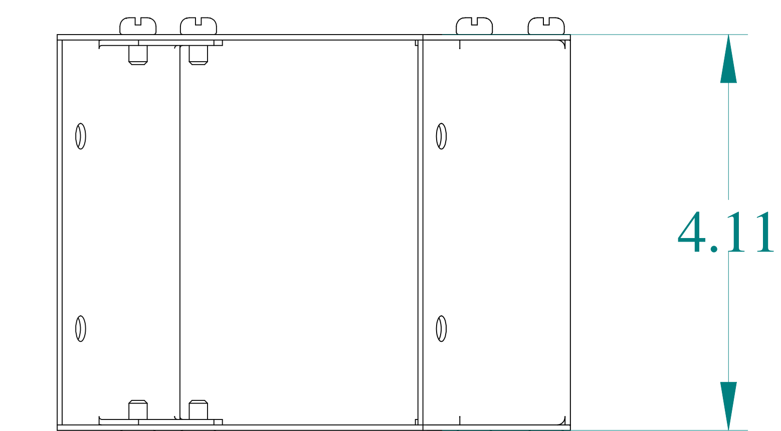
BACK VIEW
