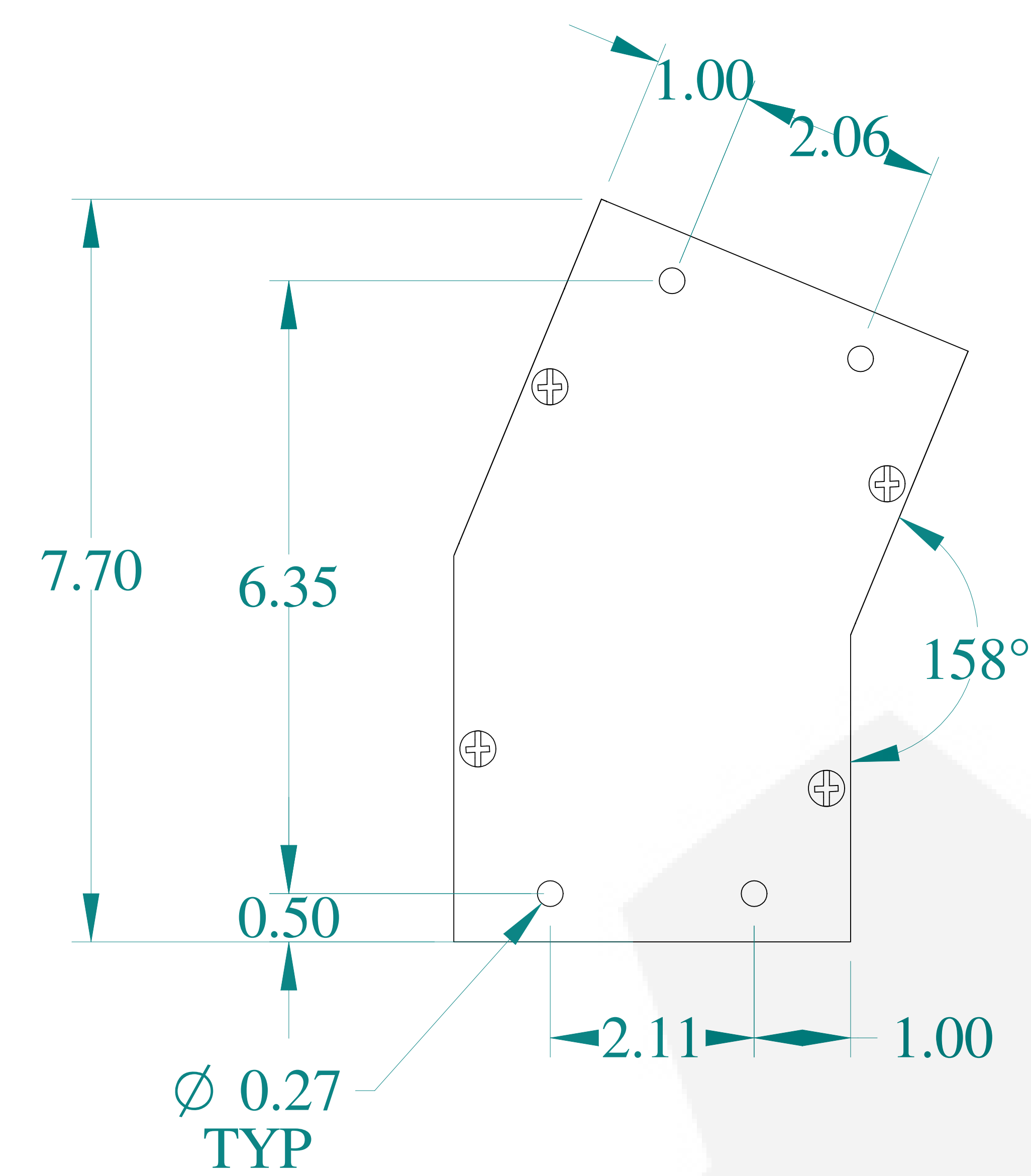
TOP VIEW
