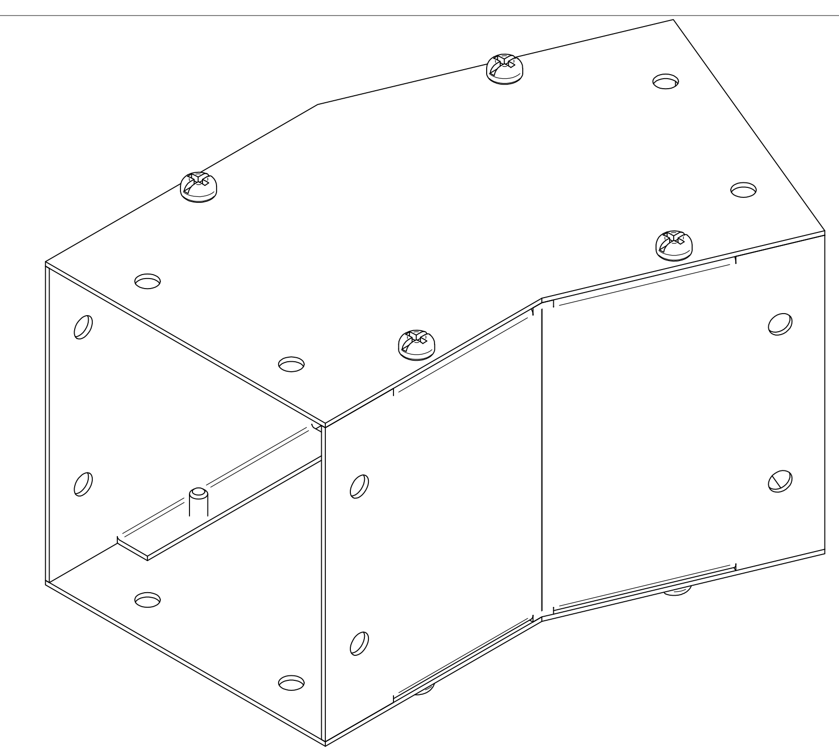
ISOMETRIC VIEWS
