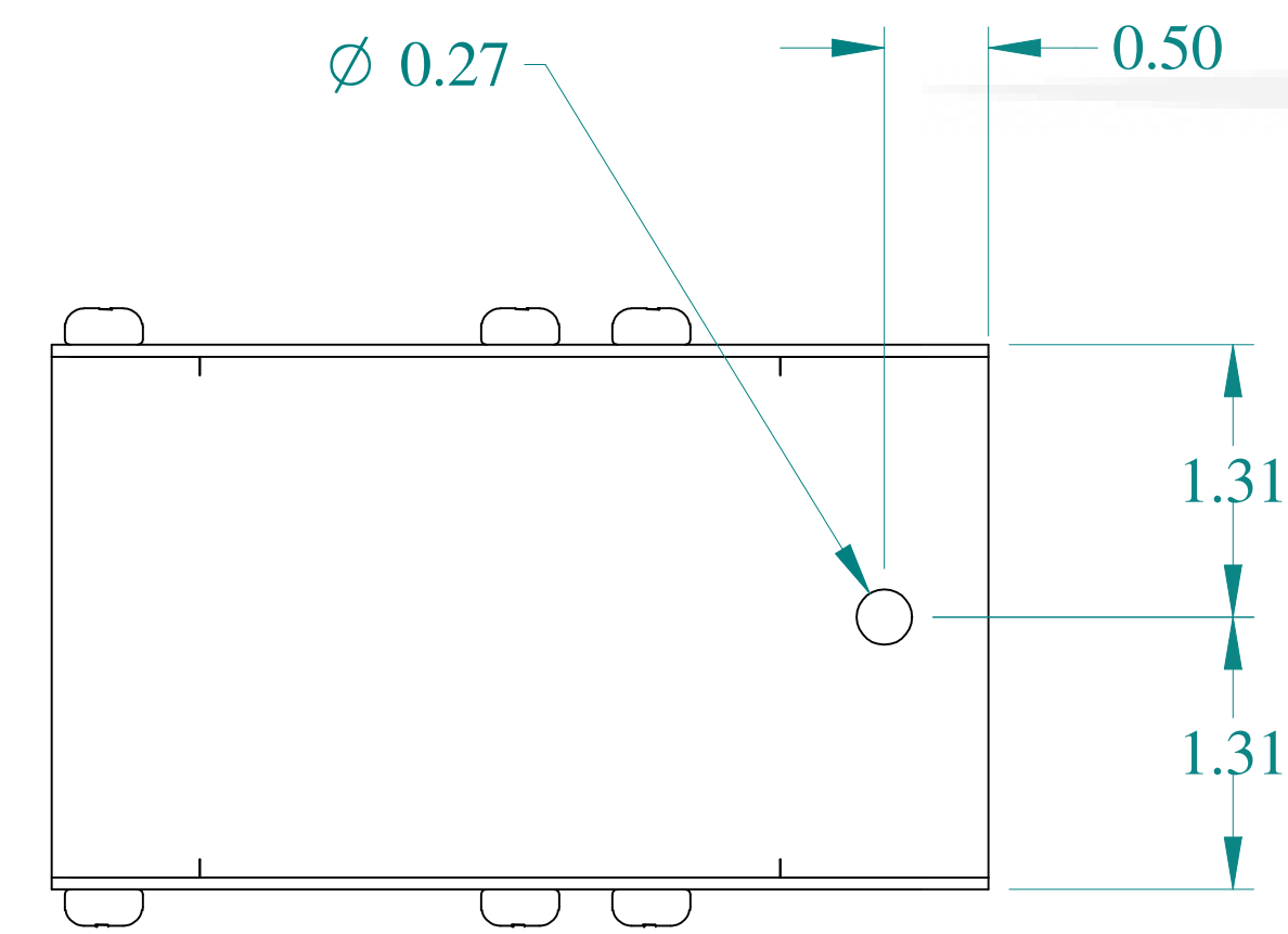
SIDE VIEW
