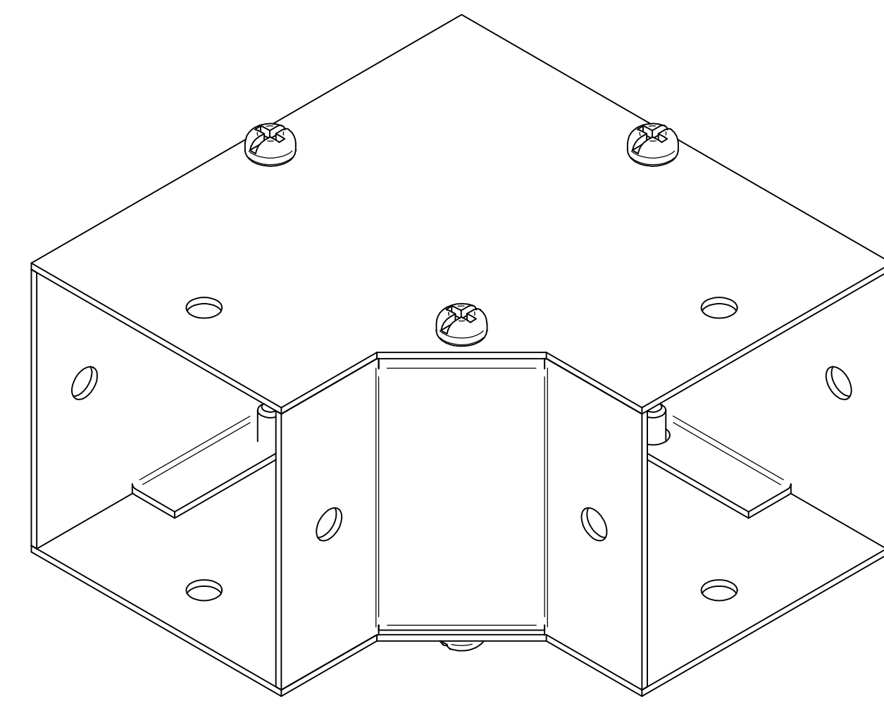
ISOMETRIC VIEWS
