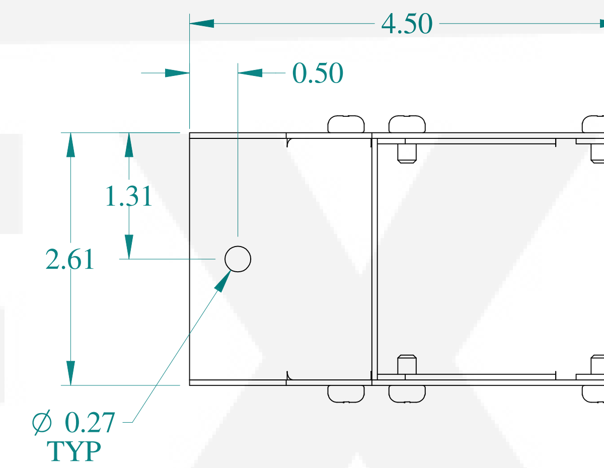
SIDE VIEW
