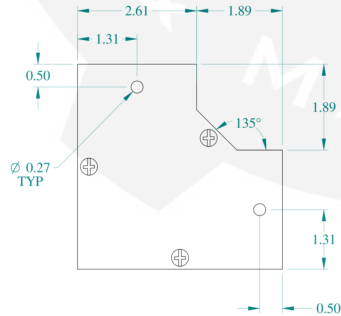
BOTTOM VIEW
