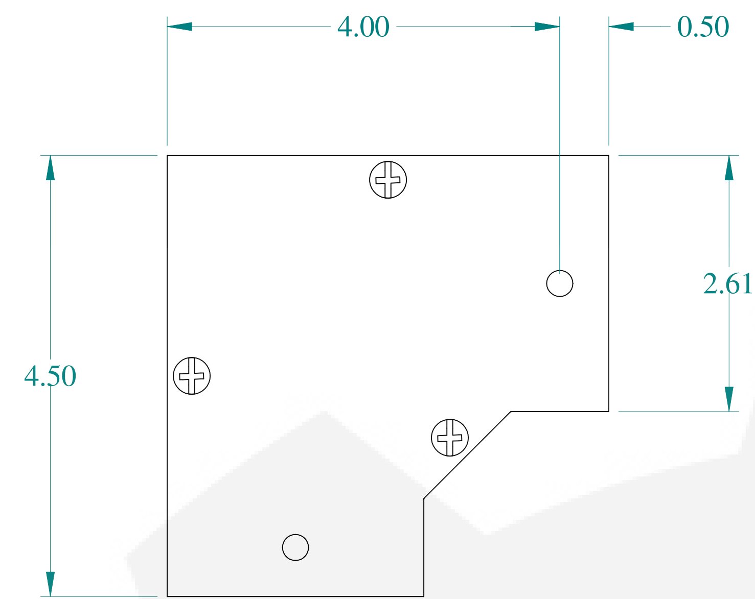
TOP VIEW
