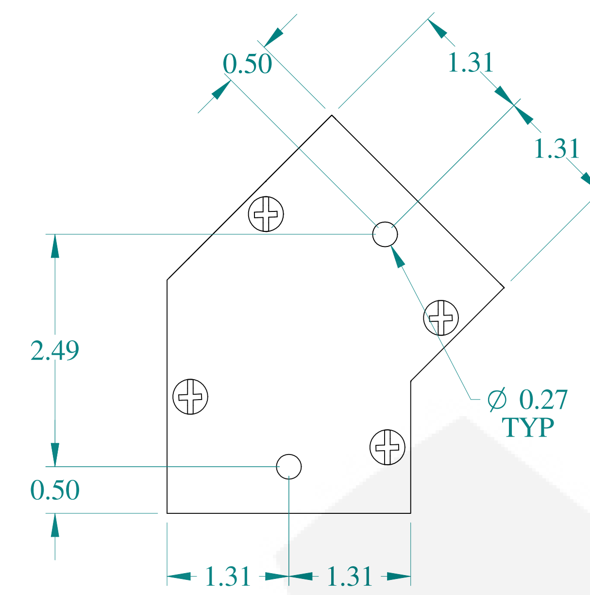
TOP VIEW
