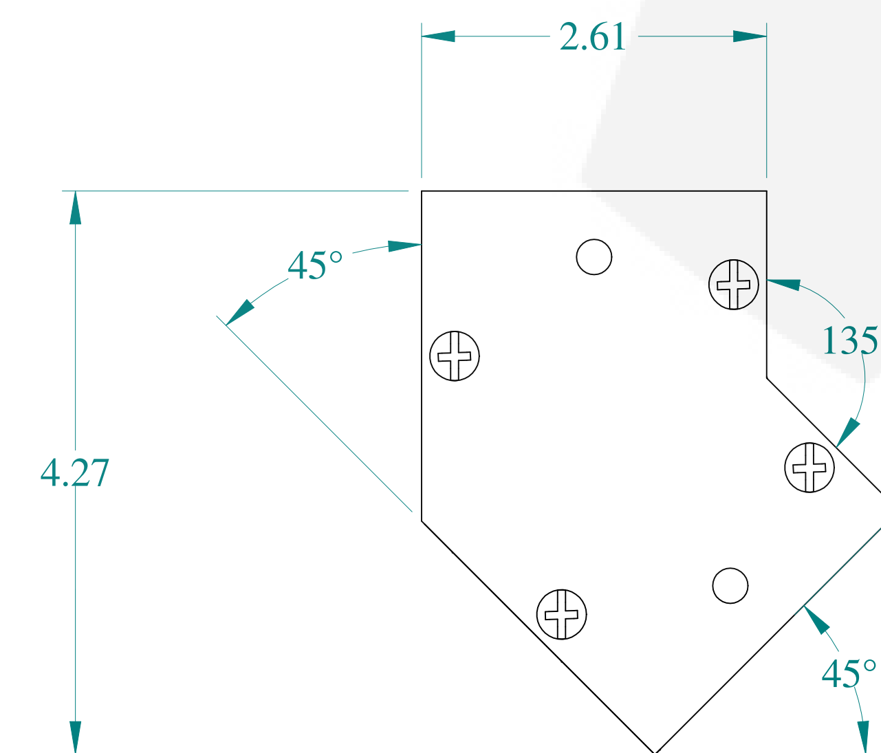
BOTTOM VIEW
