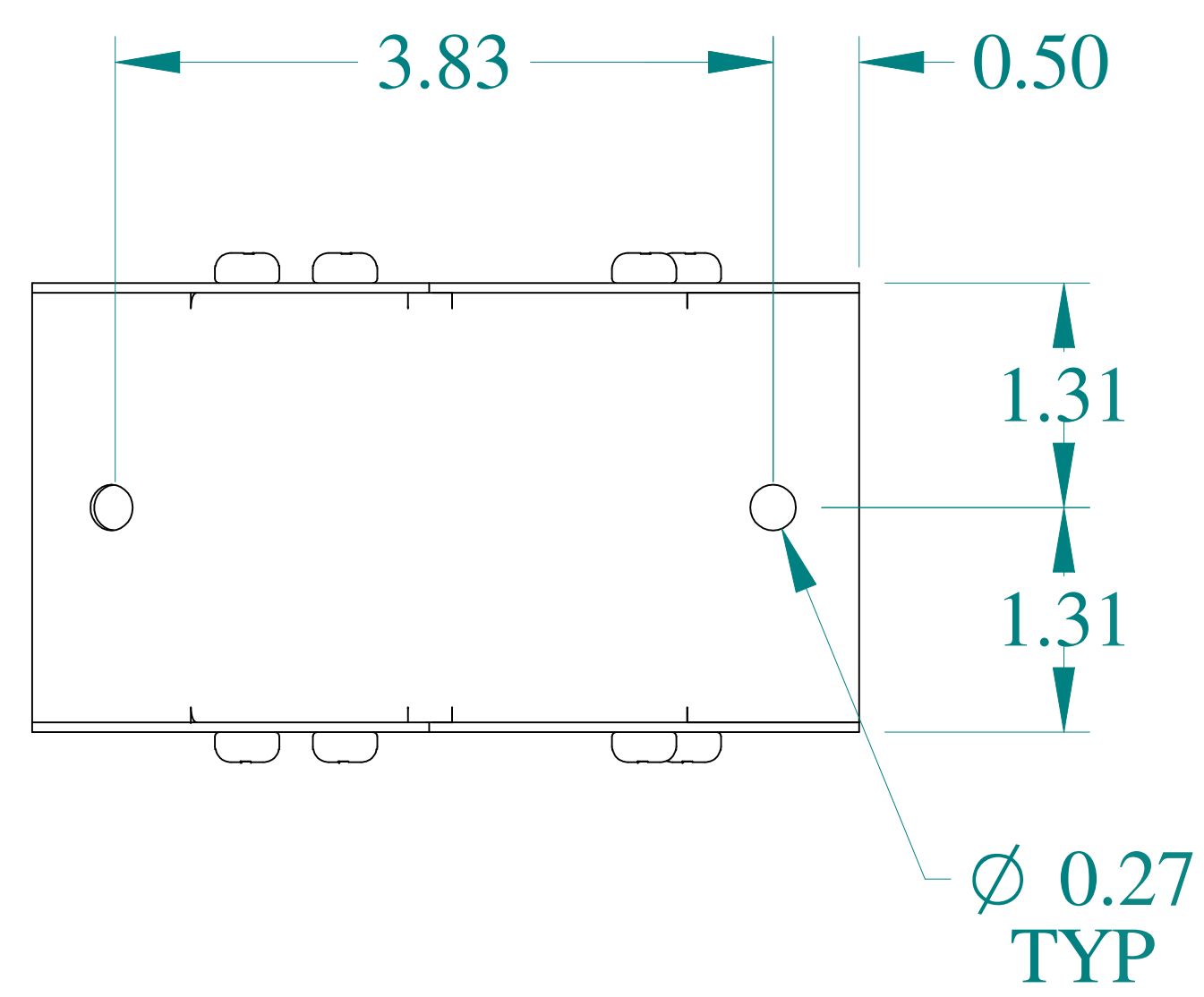
SIDE VIEW
