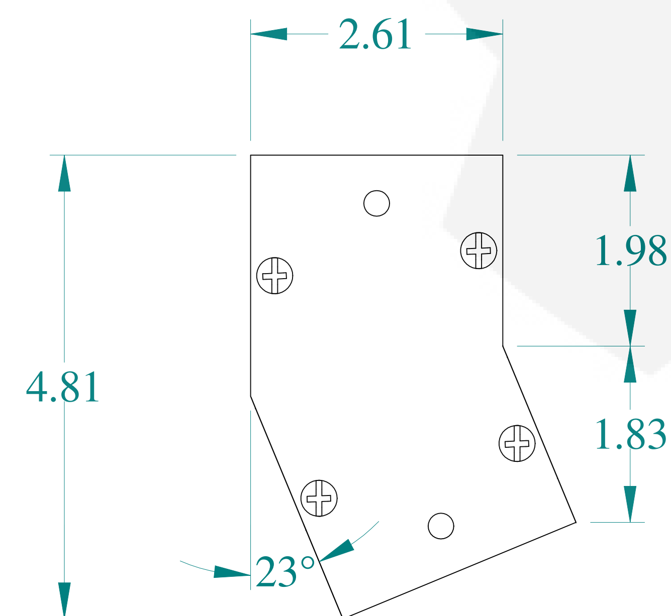
BOTTOM VIEW
