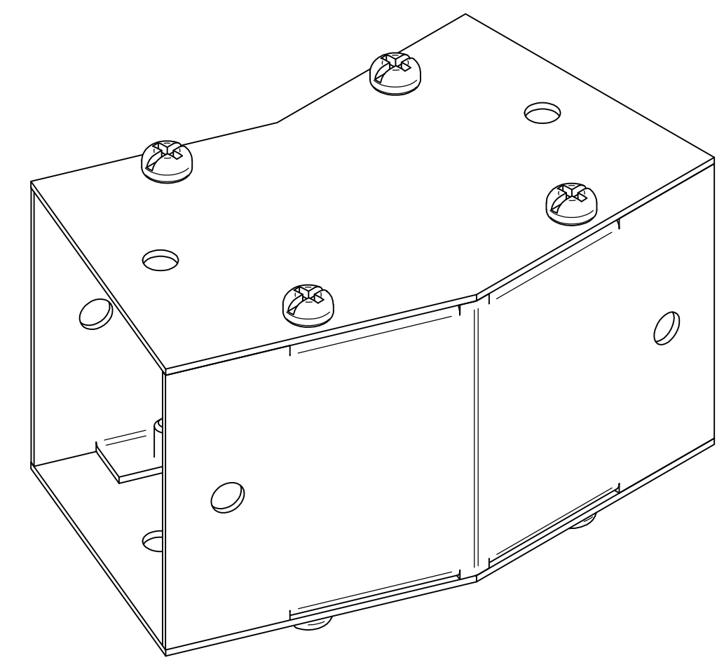
ISOMETRIC VIEWS
