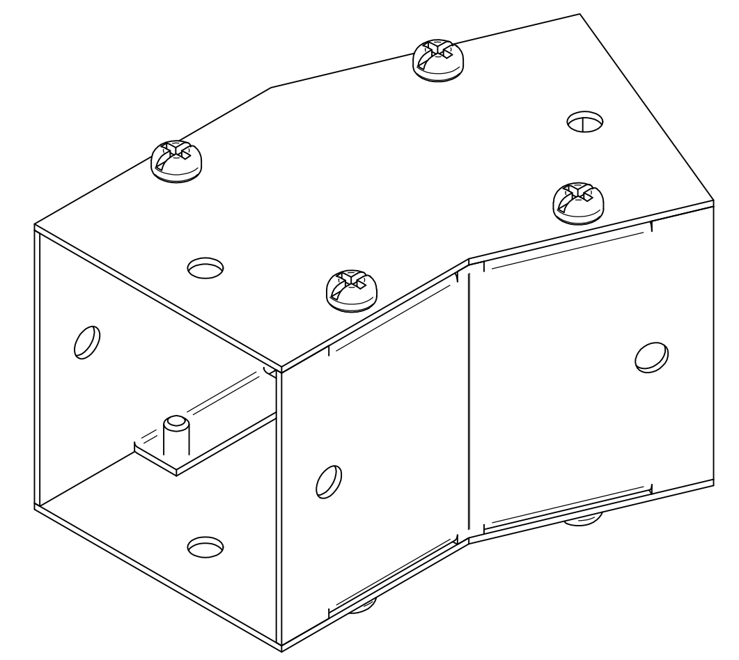
ISOMETRIC VIEWS
