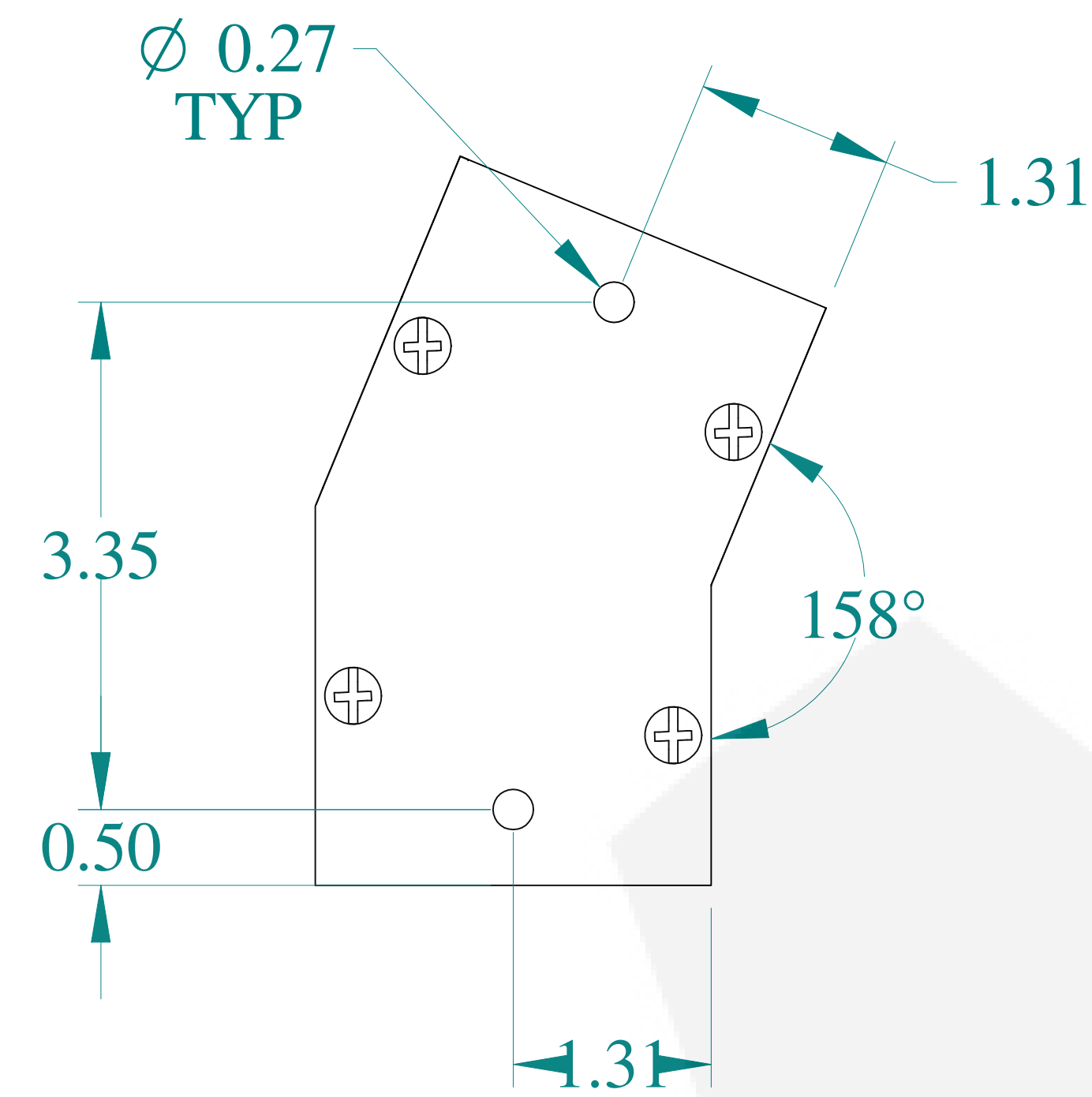
TOP VIEW
