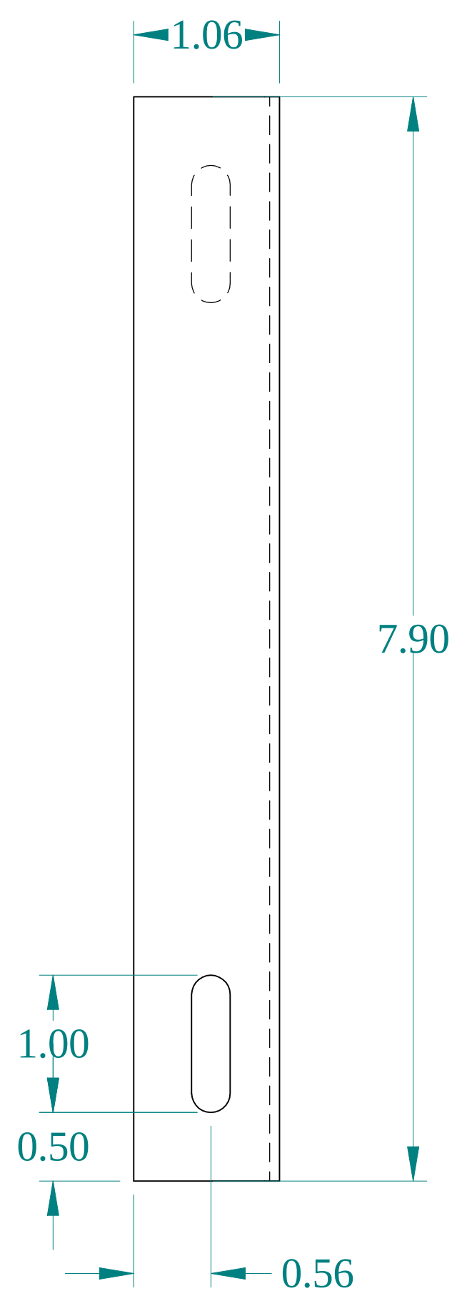
SIDE VIEW
