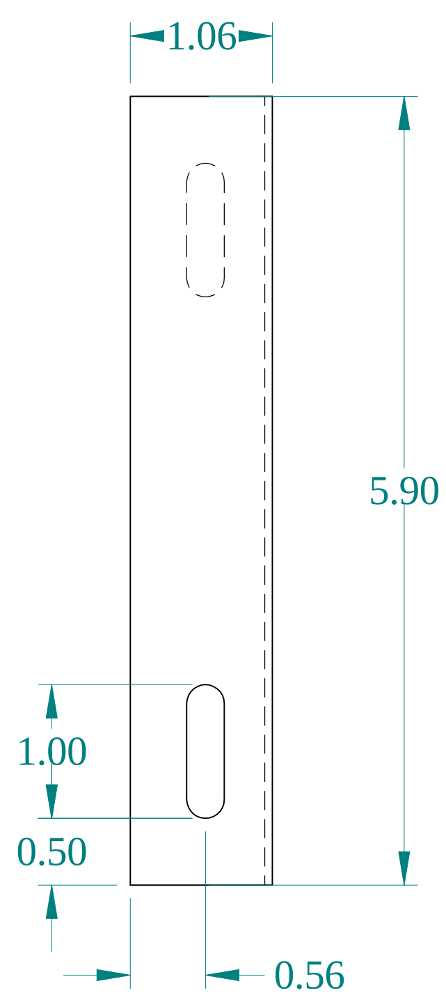
SIDE VIEW
