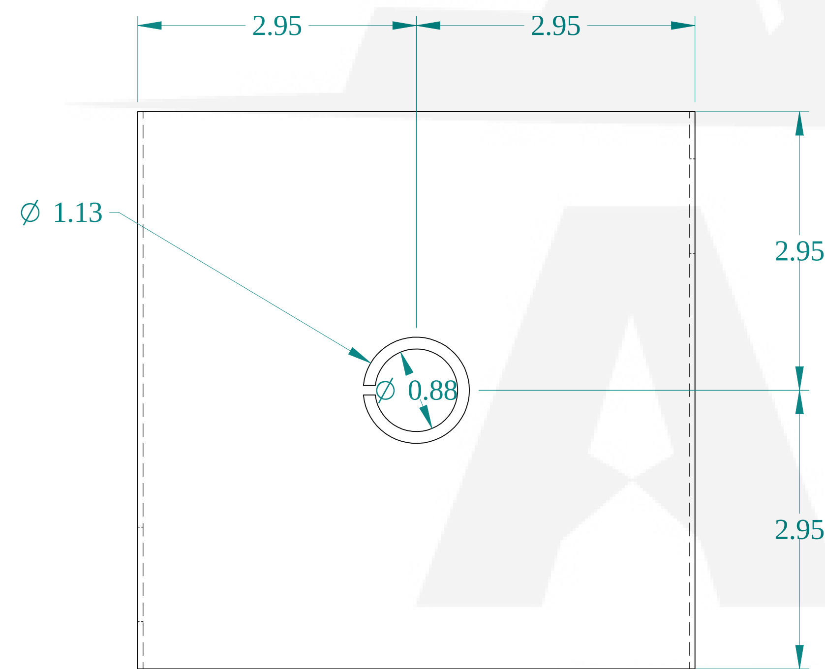
FRONT VIEW
