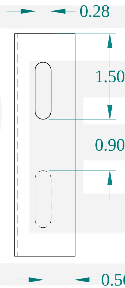
SIDE VIEW
